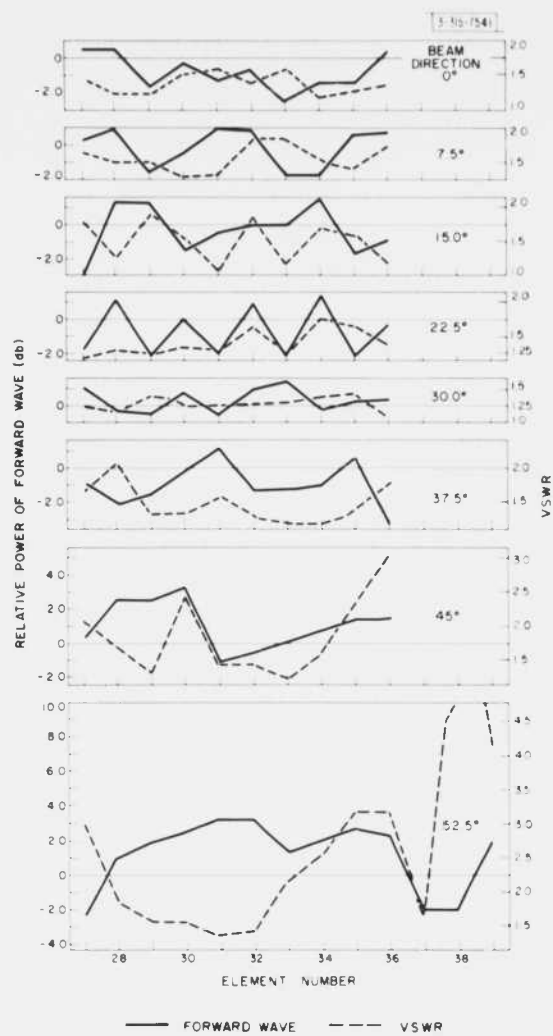
Fig. 22. Relative power of forward wave and VSWR in a few successive branch lines of row 5. Dipole length 128 inches, stub length 34 inches.
