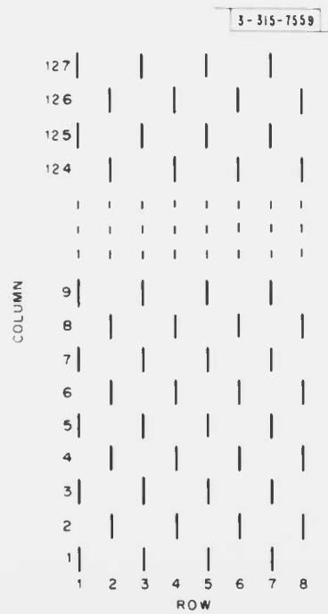
Fig. 36. Arrangement of dipoles in orthogonal array antenna.
