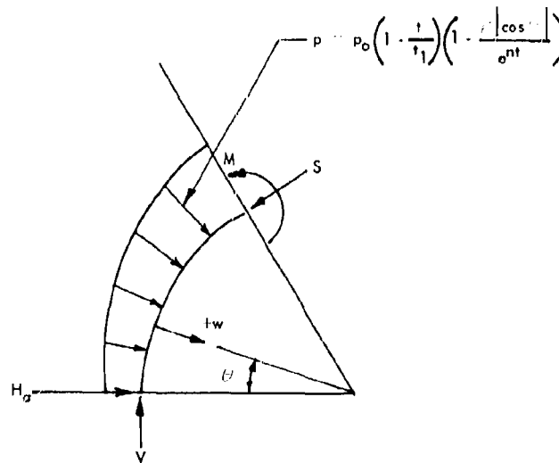
Figure 3. Load distribution on arch.
