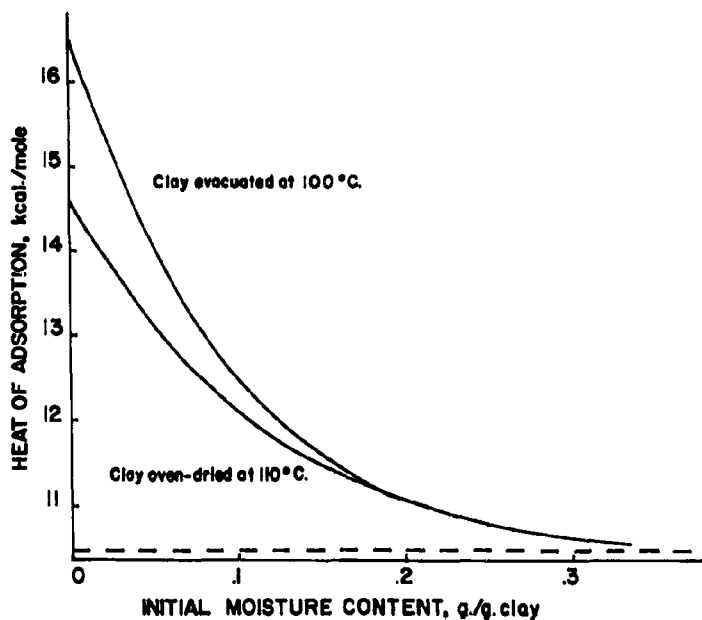
Figure 6. Variation with initial moisture content of the heat of adsorption of water vapor by Arizona bentonite.
