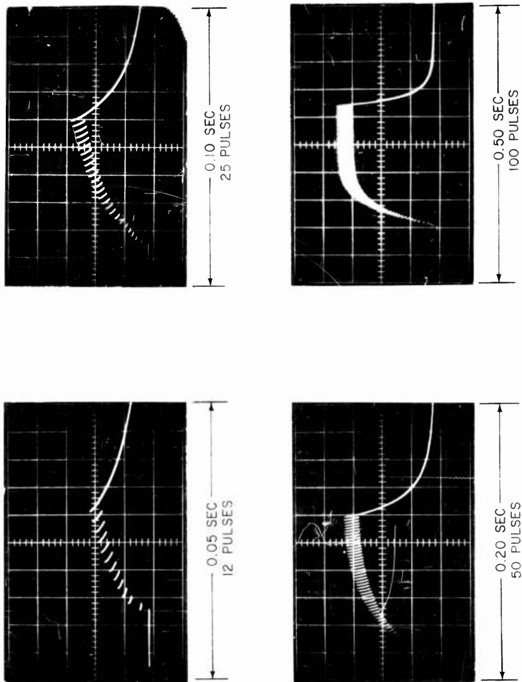
FIG.4 OBSERVED THERMAL STACKING OF SQUIB BRIDGE-WIRE DURING 9KMc RADAR TEST
