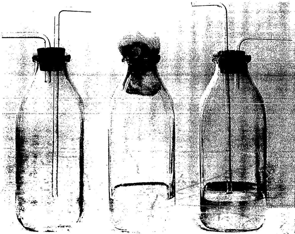
Figure 4. Critical-orifice liquid impingers.
