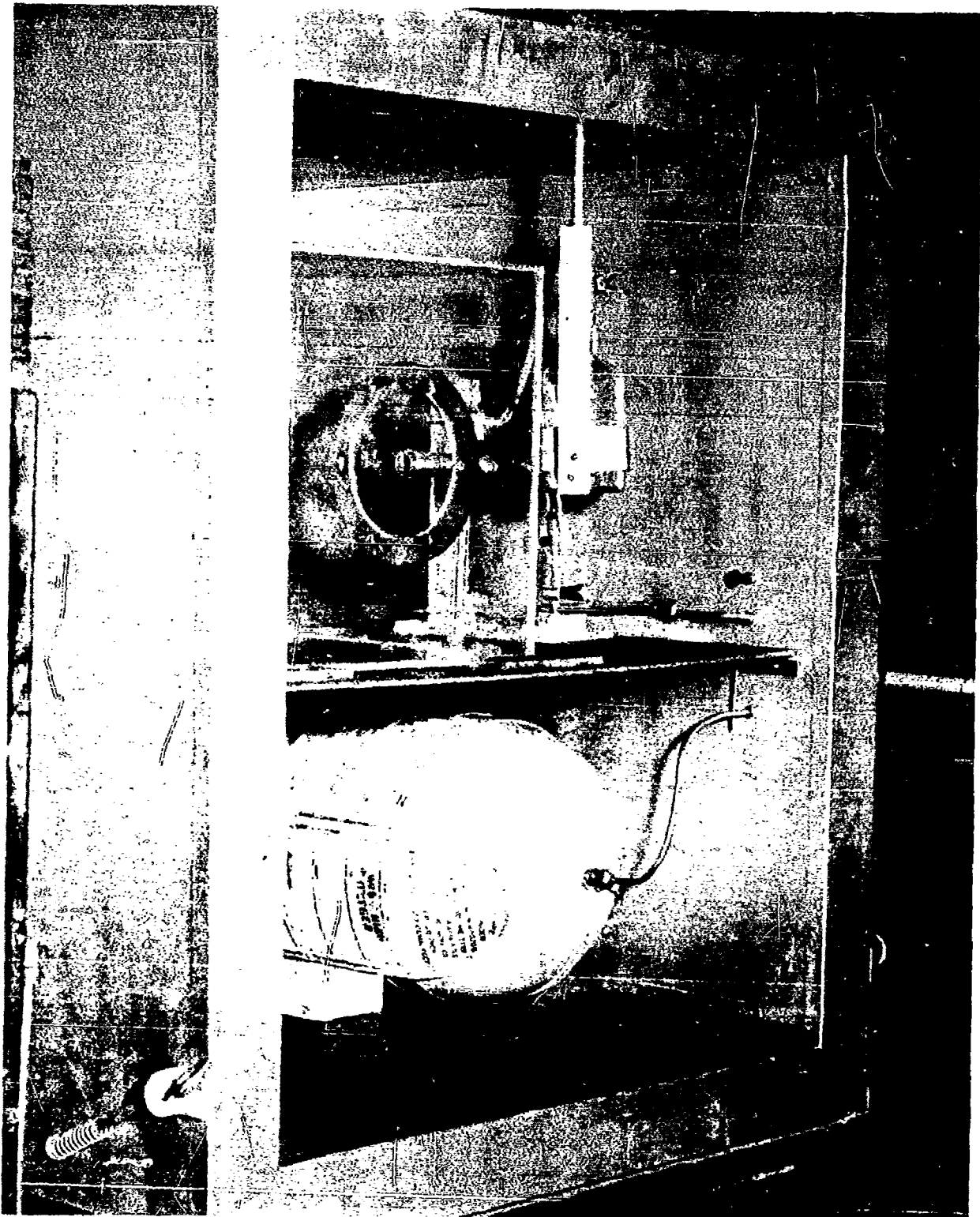
Figure 6. Prechamber box with lid open.
