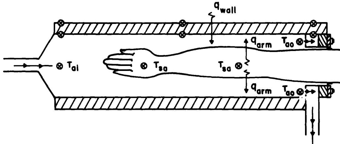
HEAT FLOWS AND THERMOCOUPLE LOCATIONS
