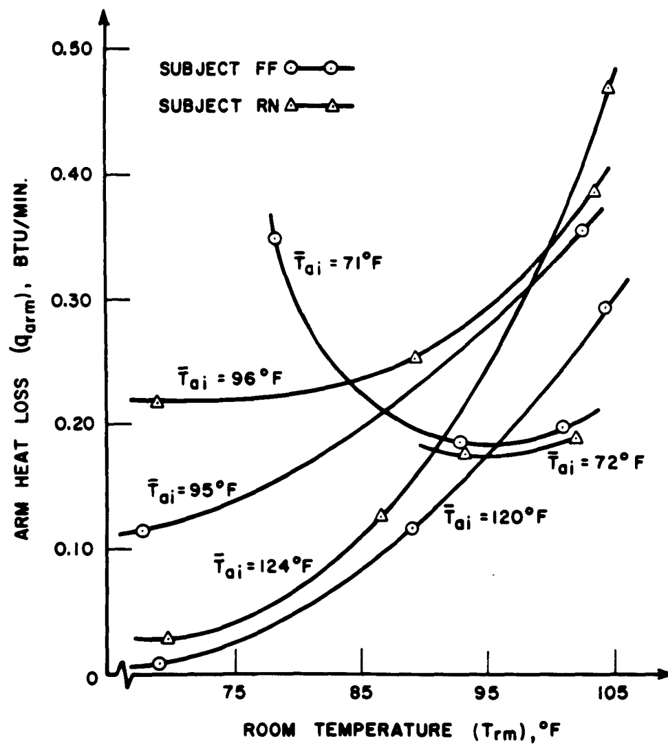
ARM HEAT LOSS AS A FUNCTION OF ROOM AIR TEMPERATURE FIGURE 16
