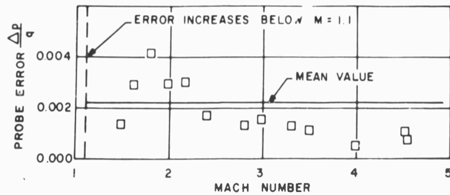
Fig.5.3 Error in indicated static pressure p_m measured in fraction of dynamic pressure q
