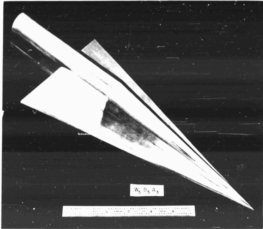
Fig.7.9 Boeing Aircraft Corporation hypersonic research force model
