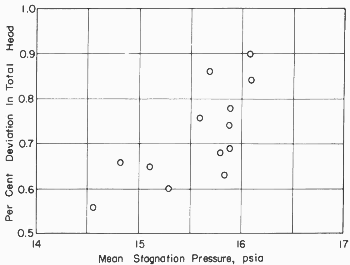
Fig.4.8 Variation of stagnation pressure fluctuations, M = 1.1 (From Ref.4.3)
