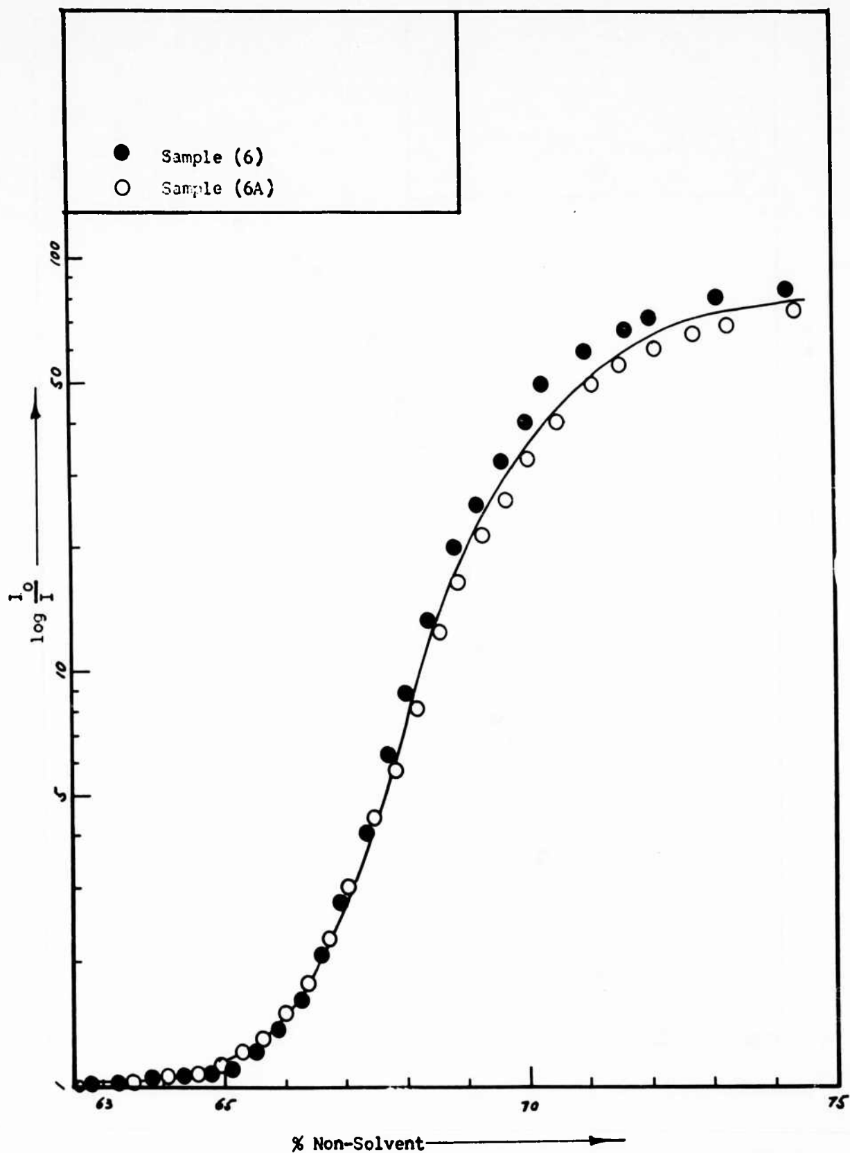
Figure 18. Turbidimetric Titration - 0.0625 \frac{\text{g. solute}}{100 \text{ ml. Solvent}}
