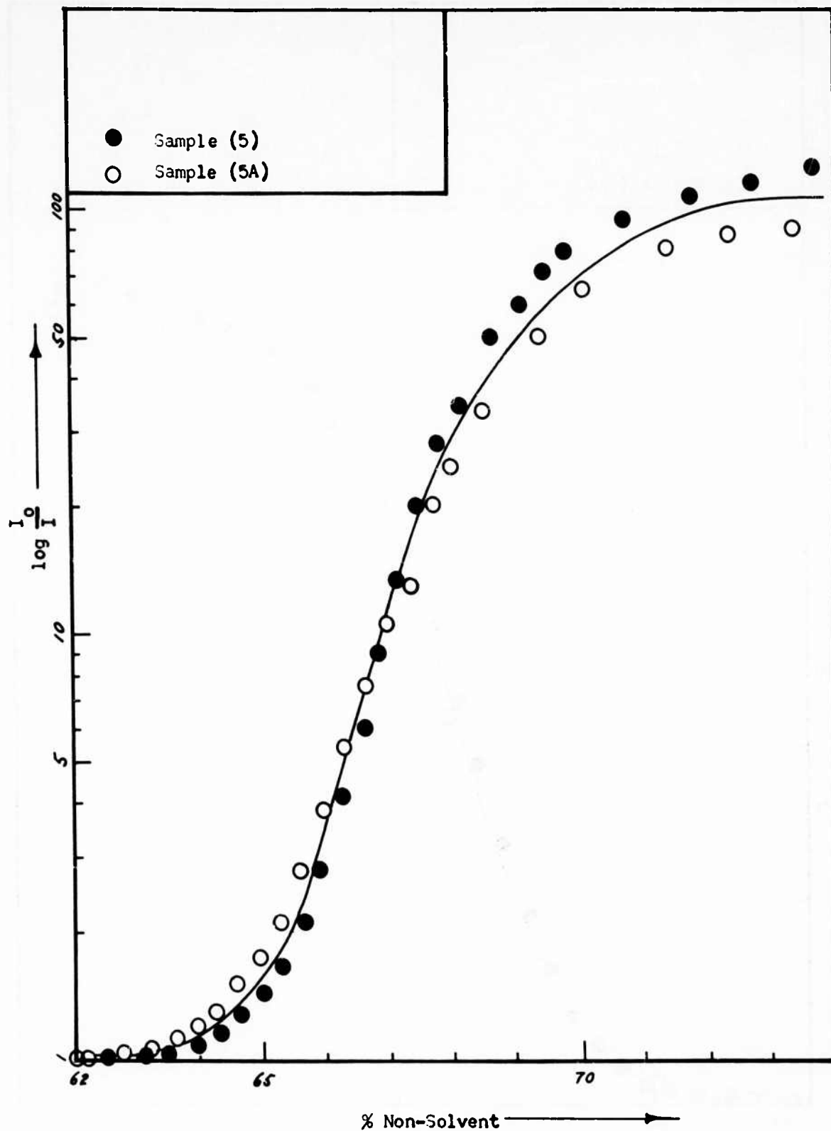
Figure 17. Turbidimetric Titration - 0.0625 \frac{\text{g. solute}}{100 \text{ ml. Solvent}}
