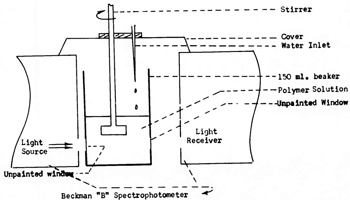
Figure 1 B. Apparatus for Turbidimetric Titration
