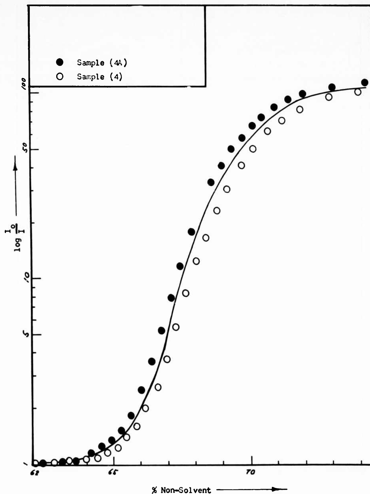
Figure 16. Turbidimetric Titration - 0.0625 \frac{\text{g. solute}}{100 \text{ ml. Solvent}}
