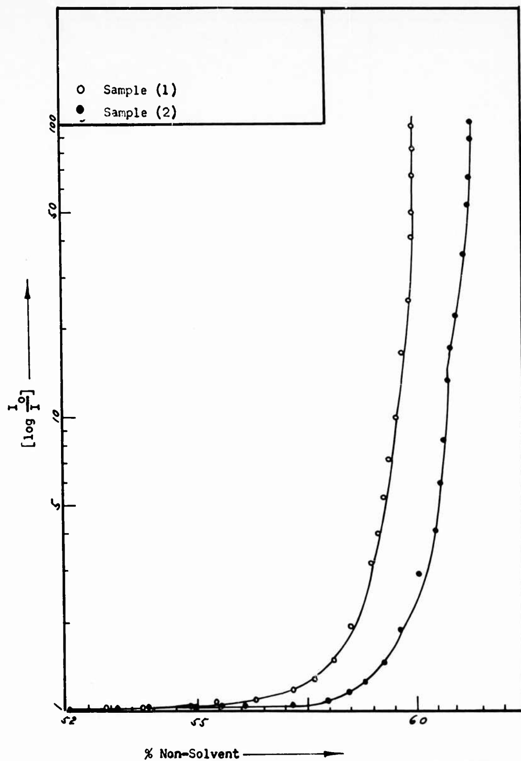
Figure 12. Turbidimetric Titration - 0.25 \frac{\text{g. solute}}{100 \text{ ml. Solvent}}
