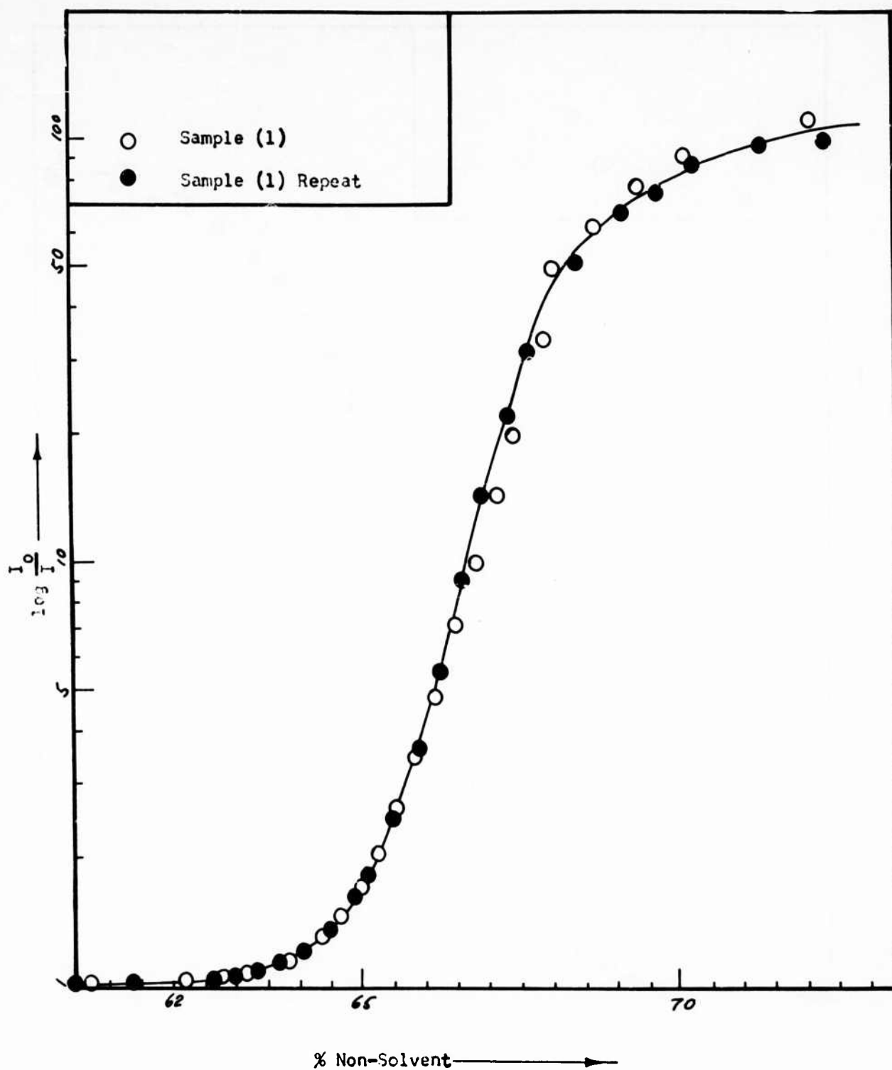
Figure 13. Turbidimetric Titration - 0.0625 \frac{\text{g. solute}}{100 \text{ ml. Solvent}}
