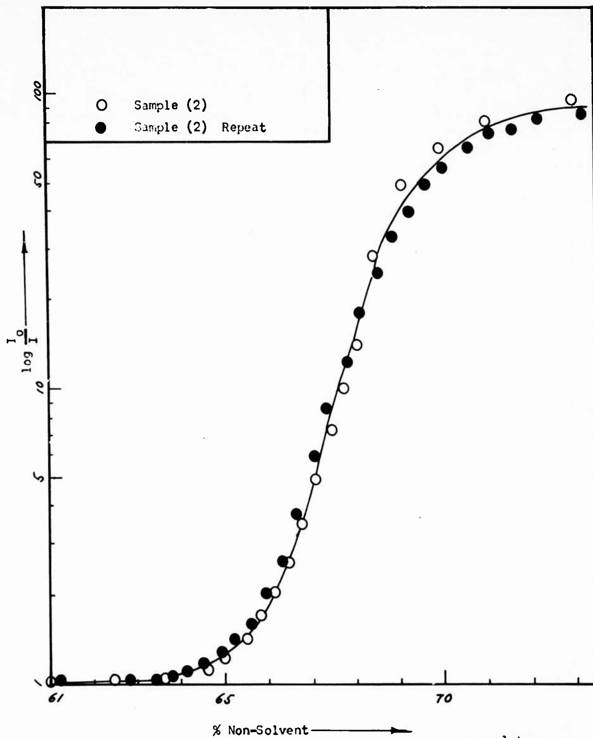
Figure 14. Turbidimetric Titration - 0.0625 \frac{\text{g. solute}}{100 \text{ ml. Solvent}}
