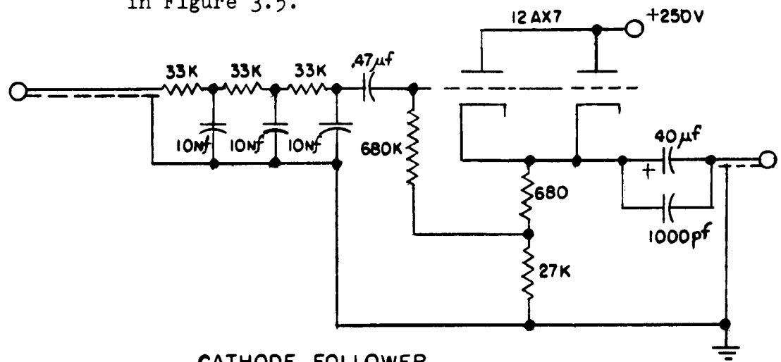
CATHODE FOLLOWER
