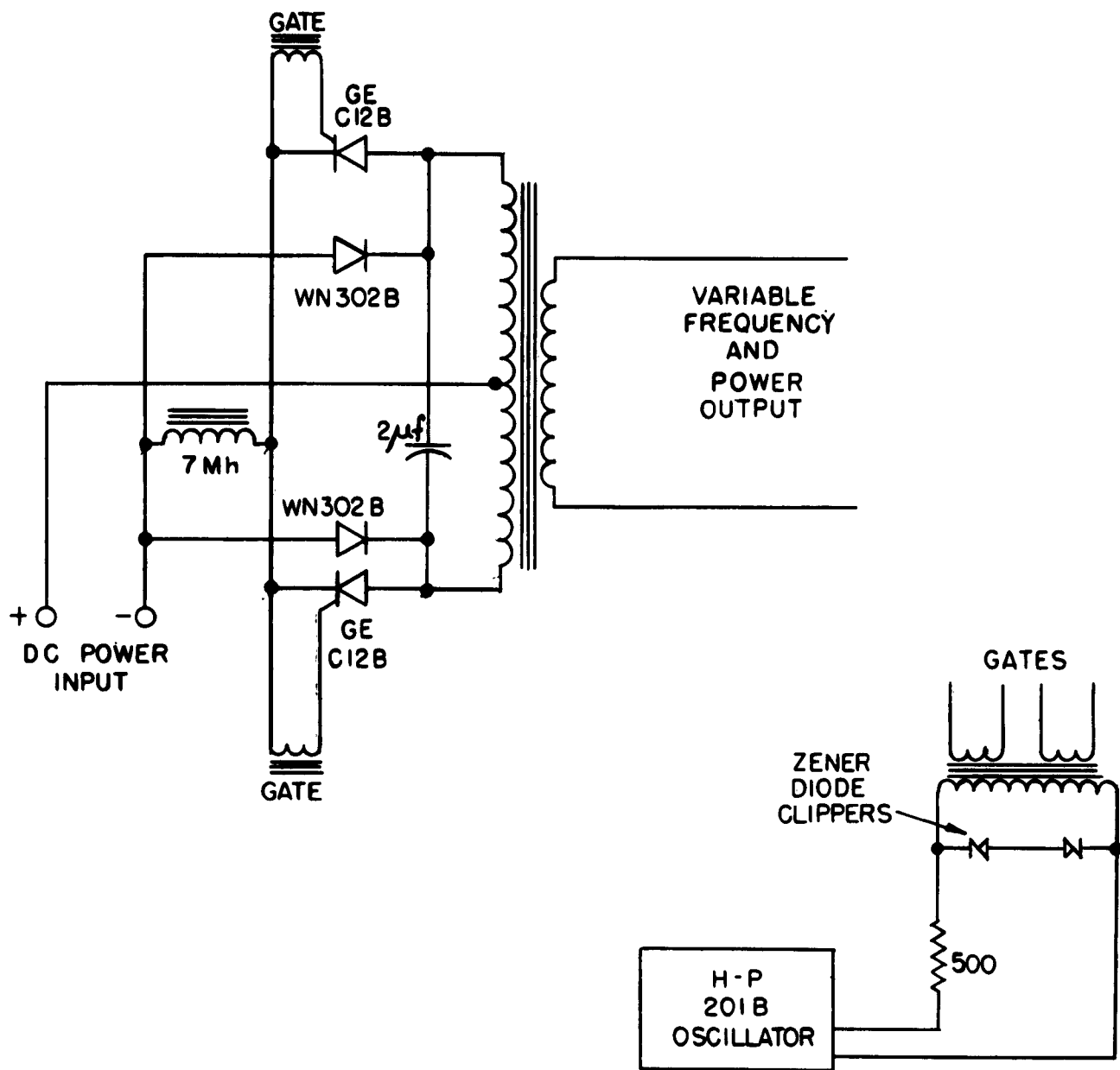
POWER OSCILLATOR
