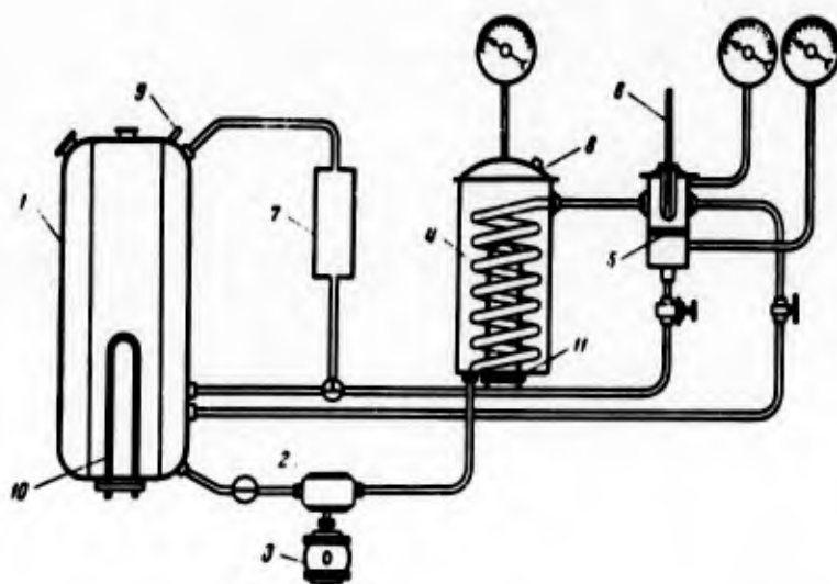
Fig. 49. Diagram of apparatus for determining thermal stability of fuels. 1) Tank; 2) pump; 3) motor; 4) coil; 5) filter; 6) thermometer; 7) fuel flowmeter; 8,9) reducing valves; 10,11) heater or cooler.
