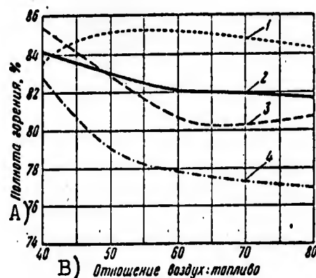
Fig. 72. Influence of chemical composition of fuel and engine operating mode on completeness of combustion. 1) Paraffinic; 2) standard; 3) naphthenic; 4) aromatic. A) Completeness of combustion, %; B) air:fuel ratio.
