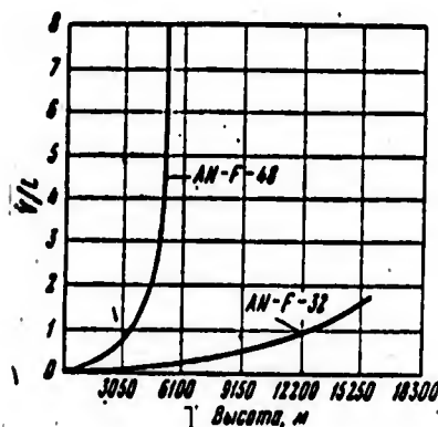
Fig. 35. Ratio of volumes of vapor and liquid phases for fuels of gasoline and kerosene types. 1) Altitude, meters.
