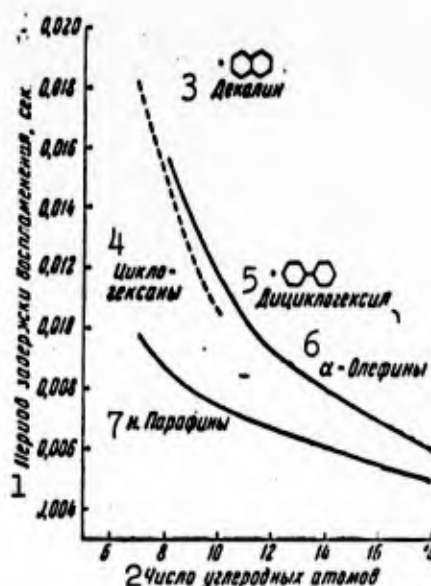
Fig. 107. Ignition lag for hydrocarbons in a bomb at 582° and 21.1 atm. 1) Ignition lag, sec; 2) number of carbon atoms; 3) decalin; 4) cyclohexanes; 5) dicyclohexyl; 6) α-olefins; 7) n. paraffins.
