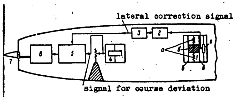
Fig. 22. Block diagram of course control; 1) lateral-acceleration pickup; 2 and 3) integrators; 4) gyroscopic device; 5) command-formation unit; 6) rudder drive; 7) rudder.
