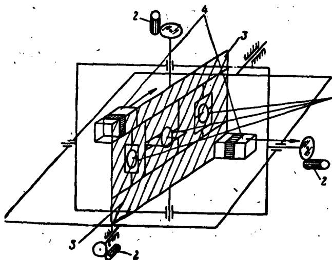
Fig. 27. Block diagram of gyro-stabilized platform: 1 ) stabilizing gyroscopes; 2 ) stabilization gears; 3 ) gyro-stabilized platform; 4 ) acceleration pickup.
