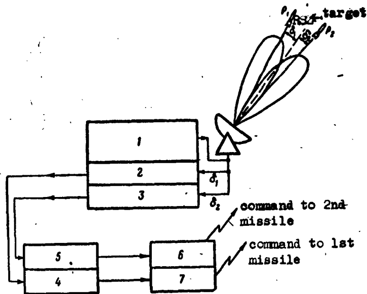
Fig. 31. Block diagram of a radio sight combined with radar target tracking: 1) radar tracking; 2), 3) sighting units for the first and second missiles; 4), 5) command-formation units for the first and second missiles; 6), 7) command-transmission lines.
