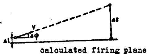
Fig. 25. The components of course error: \Delta l is the lateral deviation of the point of engine cutoff from the calculated firing plane; \Delta \psi the deviation of the velocity vector at the moment of engine cutoff; and \Delta Z the over-all lateral firing error.
