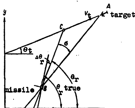
Fig. 34 Homing with course guidance: \theta_t - course of target; C - predicted point of impact; \sigma - prediction angle; \theta_r - required course of missile; \theta_r \text{ true} - true course of missile; \Delta\theta_r - error signal.
