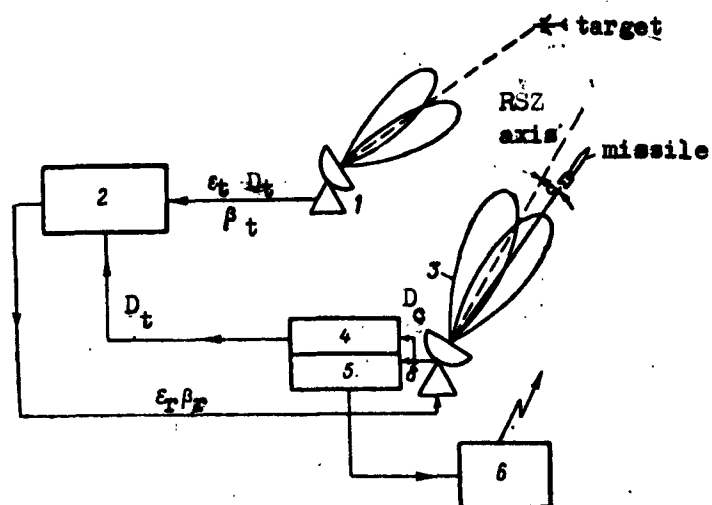
Fig. 30. Block diagram of ground complex for guidance by radio sighting: 1) radar tracking of target ; 2) computer for predicted values of azimuth \beta_r and angle of elevation \delta_r of missile; 3) radio sighter; 4) missile r range finder; 5) command-formation unit; 6) command transmission line.
