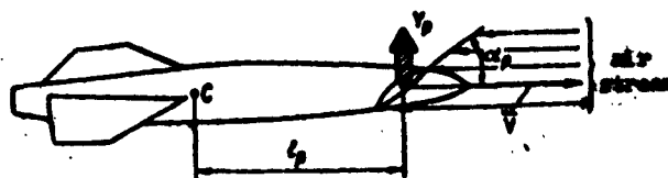
Fig. 16. Missile guidance using an aerodynamic rudder: \alpha_p is the angle of attack of the rudder; V_p the aerodynamic lift force of the rudder; V the direction of the velocity of the missile; C the center of gravity of the missile; and l_p the force arm of the rudder.
