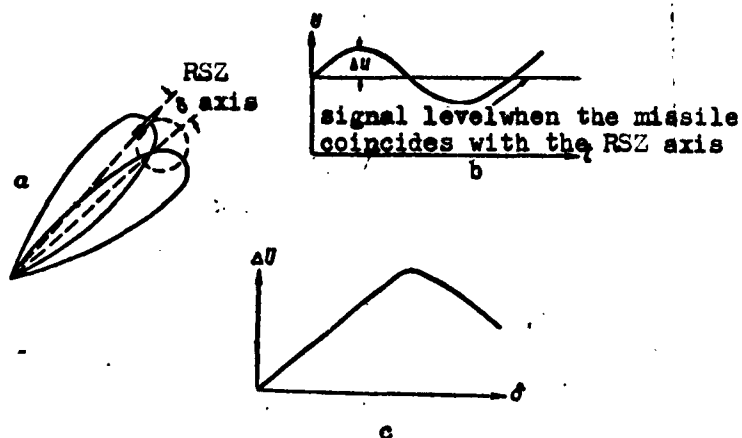
Fig. 28. Formation of an error signal with a scanning beam: a) scanning beam; b) fluctuation of signal at receiving point; c) amplitude \Delta U as a function of deviation \delta .
