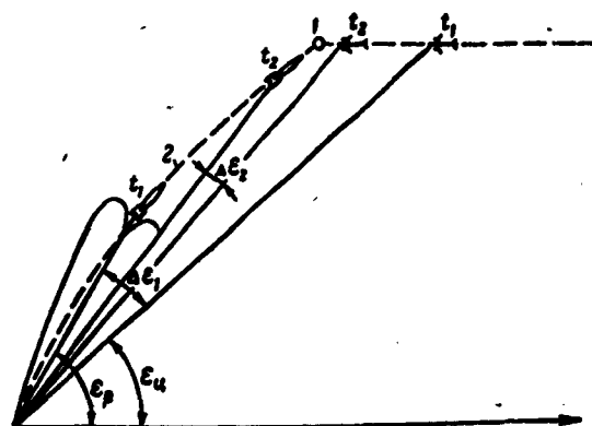
Fig. 29. The positions of the target and missile in guidance to a predicted point: 1) predicted point of impact; 2) trajectory of missile; \Delta \epsilon_1 and \Delta \epsilon_2 are values of the angular prediction at times t_1 and t_2 .
