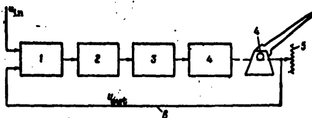
Fig. 1. Block diagram of automatic control system 1) sensitive element; 2) device for command generation; 3) amplifier; 4) barrel drive; 5) potentiometer for measuring the position angle of the barrel; 6) feedback loop.
