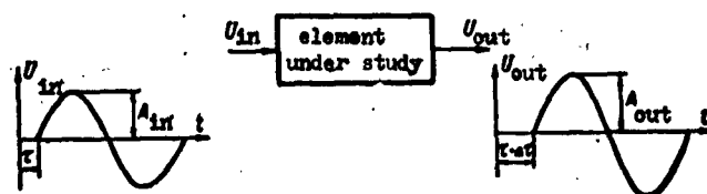
Fig. 4. Input ( U_{in} ) and output ( U_{out} ) signals when taking the frequency characteristic.
