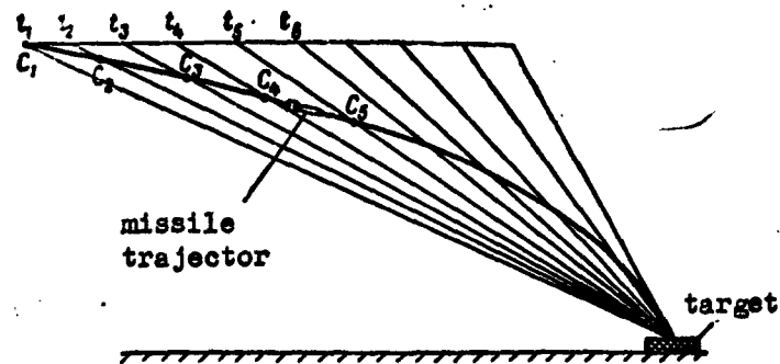
Fig. 44. Trajectory of air-to-ground missile with three-point guidance.
