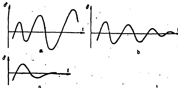
Fig. 2. Processes in various automatic control systems:
