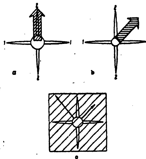
Fig. 14. Lift force in a two-plane aerodynamic plan: a) angle of attack in plane 2-2; b) angle of attack in planes 1-1 and 2-2; c) region of possible lift forces for various combinations of angles of attack.
