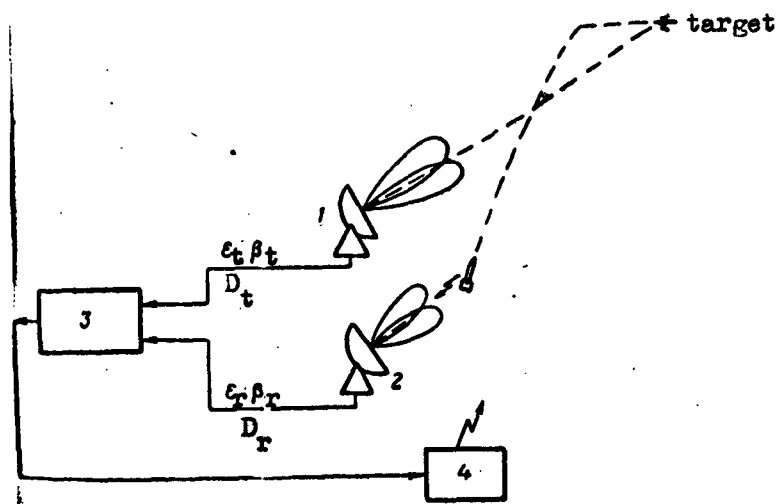
Fig. 32. Block diagram of ground complex for guidance by two radar signals: 1) radar tracking of target; 2) radar tracking of missile; 3) command-forming computer; 4) transmission line for commands.
