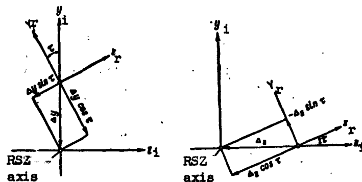
Fig. 40. Redistribution of commands taking the skew angle into account.
