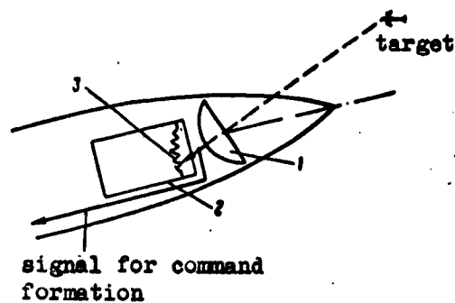
Fig. 49. Diagram of homing-head with gyroplatform: 1) homing-head; 2) gyroplatform; 3) potentiometer for measuring the position of the antenna axis relative to the gyroplatform.
