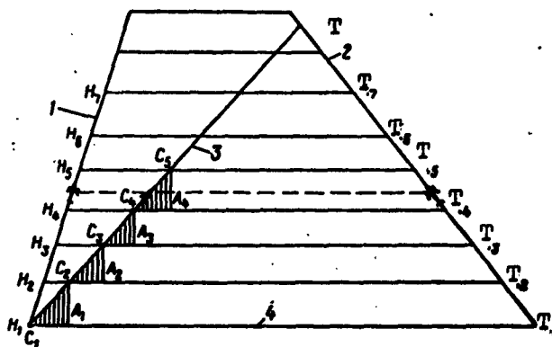
Fig. 45. Trajectory of air-to-air missile with three-point guidance: 1) carrier aircraft (control point) trajectory; 2) target trajectory; 3) missile trajectory; 4) guidance line.
