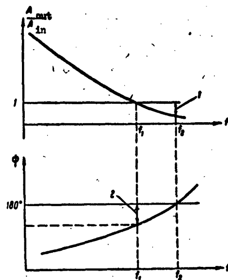
Fig. 7. Frequency characteristics of an open system: 1) amplitude stability margin; 2) phase stability margin.
