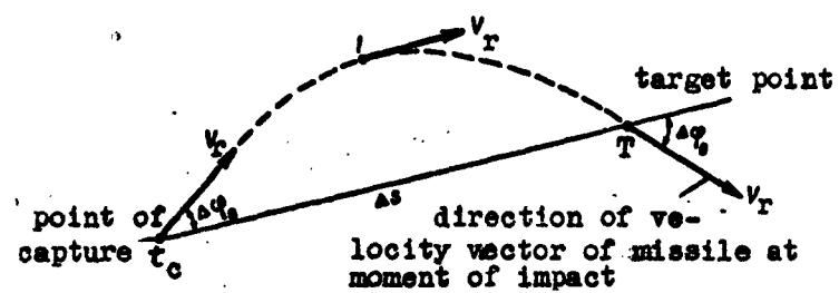
Fig. 51. Limiting trajectory which ensures guidance to the target.
