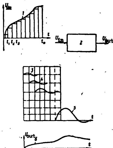
Fig. 9. Finding the output signal with an input signal of arbitrary shape: 1) input signal; 2) system under study; 3) action of system on first pulse; 4) action on system on second pulse; 5) action of system on n -th pulse; 6) output signal, found as sum of all elementary signals.
