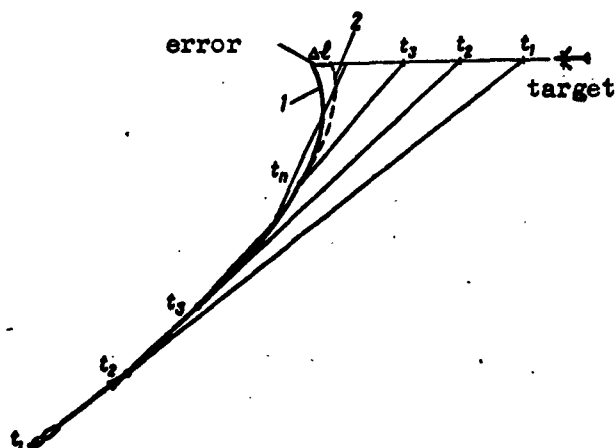
Fig. 48. Required (1) and real (2) trajectories in guidance on a pursuit curve.
