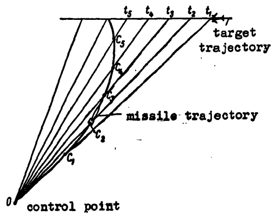
Fig. 43. Trajectory of surface-to-air missile in three-point guidance.
