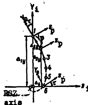
Fig. 39. Initial deviation \Delta_{ly} in the presence of skew.
