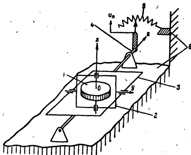
Fig. 19. Diagram of three-degree-of-freedom gyroscope: 1--rotor; 2--inner frame of gimbal; 3--outer frame of gimbal; 4--measuring axis; 5--measuring potentiometer; 6--body of missile.
