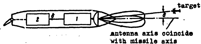
Fig. 46. Homing with target sighting (the homing-head antenna is rigidly mounted on the body of the missile): \delta - is the error signal; 1) unit for error signal separation and command formation; 2) rudder drive.
