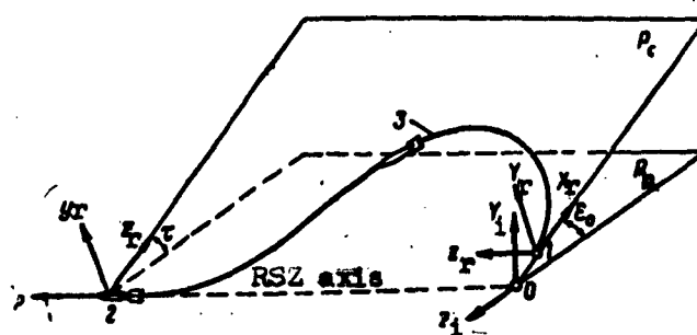
Fig. 38. Formation of skew angle \tau : P_h is the plane of the horizon; P_c the firing plane; 1) the initial position of the axes of the missile; 2) the final position of the missile; 3) trajectory; Y_1, Z_1 is the final position of measuring the radio-sight axes.
