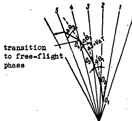
Fig. 42. Additional bending of trajectory during transition to the free-flight phase.
