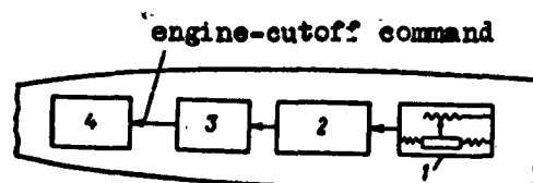
Fig. 23. Block diagram of engine-cutoff device: 1) axial-acceleration pickup; 2) integrator-determiner of velocity; 3) comparison unit; 4) engine-cutoff control.
