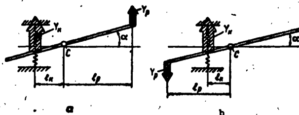
Fig. 17. Mechanical analogs of two control plans: a) "canard" plan; b) normal plan; \alpha is the angle of attack; Y_k the lift force of the wing; Y_p the lift force of the rudder; l_k the force arm of the wing; l_p the force arm of the rudder; C the center of gravity.
