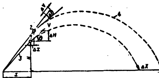
Fig. 24. The components of range error: 1 ) calculated point of engine cutoff; 2 ) actual point of engine cutoff; 3 ) guidance phase; 4 ) ballistic trajectory phase; X , H , \theta , V are the calculated values of the range, altitude, deflection angle and the velocity at the moment of engine cutoff; \Delta X , \Delta H , \Delta \theta , \Delta V are the errors in range, altitude, deflection angle and velocity at the actual point of engine cutoff; and \Delta X is the over-all range error.
