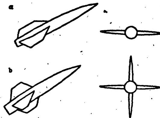
Fig. 12. Two configurations for aerodynamic surfaces: a) single-plane aerodynamic plan; b) two-plane symmetrical aerodynamic plan.
