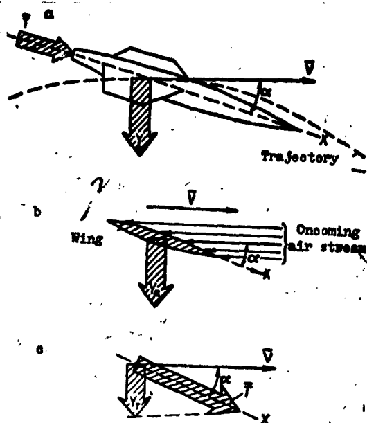
Fig. 11. Lift force diagrams: a) over-all diagram; b) aerodynamic lift; c) lift due to thrust; V is the velocity vector; X the longitudinal axis of the missile; the angle of attack; T the thrust; Y the total lift force; Y_a the aerodynamic lift; Y_T the lift component due to thrust.
