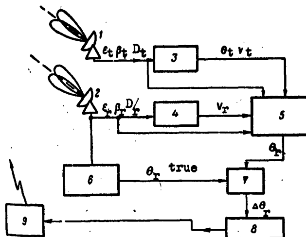
Fig. 33. Block diagram of course control method. 1) radar tracking of target; 2) radar tracking of missile; 3) device for determining the course and velocity of target; 4) device for determining the velocity of the missile; 5) device for solving the predicted triangle and forming the required course \theta_r ; 6) device for determining the true course of the missile \theta_r \text{ true} ; 7) comparison unit and unit for formation of error signal \Delta\theta_r ; 8) command-formation unit; 9) transmission line for commands.
