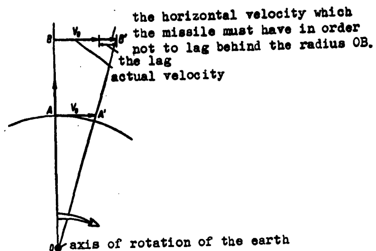
Fig. 26. Relative displacement of missile due to the earth's rotation.
