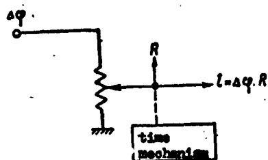
Fig. 37. Block diagram of converter of angular error to linear used in the Oerlikon-54 system.
