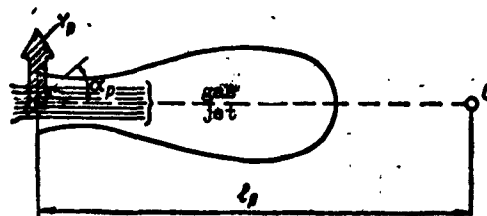
Fig. 18. Diagram of action of gas rudder: Y_p is the gas dynamic lift force of the rudder; \alpha_p the angle of attack of the rudder; C the center of gravity of the missile; and l_p the force arm of the gas rudder.
