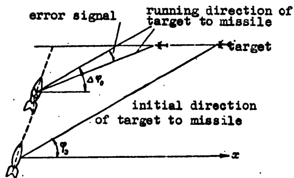
Fig. 50. The error signal in the method of parallel engagement.
