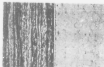
Mo-0.5Ti R-41 A3402-Y3429 250X
