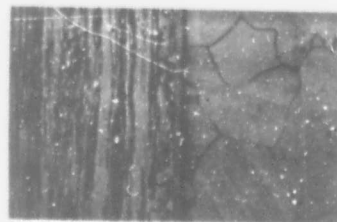
Mo-0.5Ti R-41 A83-Y186 250X
