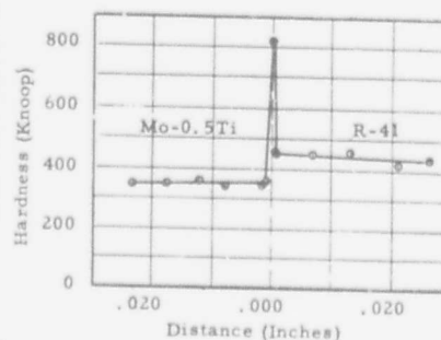
C. Mo-0.5Ti/Cr/R-41 : 1800°F/4 hrs.
