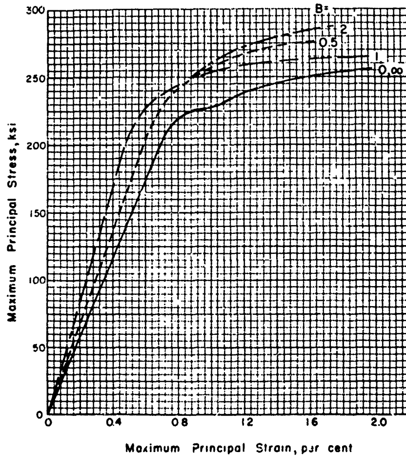
FIGURE 5. TYPICAL BIAXIAL STRESS-STRAIN CURVES AT ROOM TEMPERATURE FOR AISI 4340 ALLOY-STEEL CYLINDERS, F_{tu} = 260 \text{ KSI}
