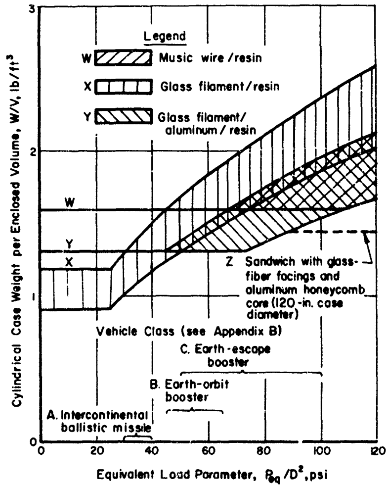
FIGURE 16. WEIGHT OF CYLINDRICAL PORTION OF ROCKET-MOTOR CASE PER UNIT OF ENCLOSED VOLUME VERSUS AN EQUIVALENT EXTERNAL LOAD PARAMETER FOR VARIOUS COMPOSITE CONSTRUCTIONS
