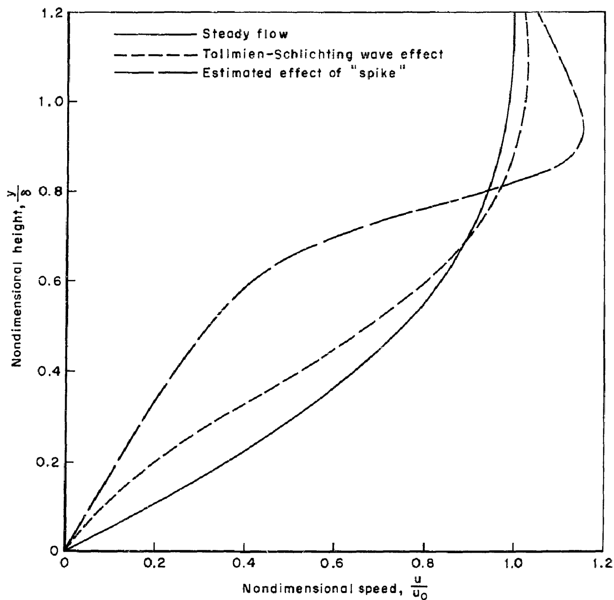
Fig.2—Speed distribution in the laminar boundary layer on a flat plate
