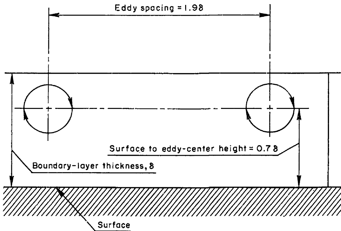
Fig. 3 — Flow pattern of the high-frequency instability at its origin in the laminar boundary layer
