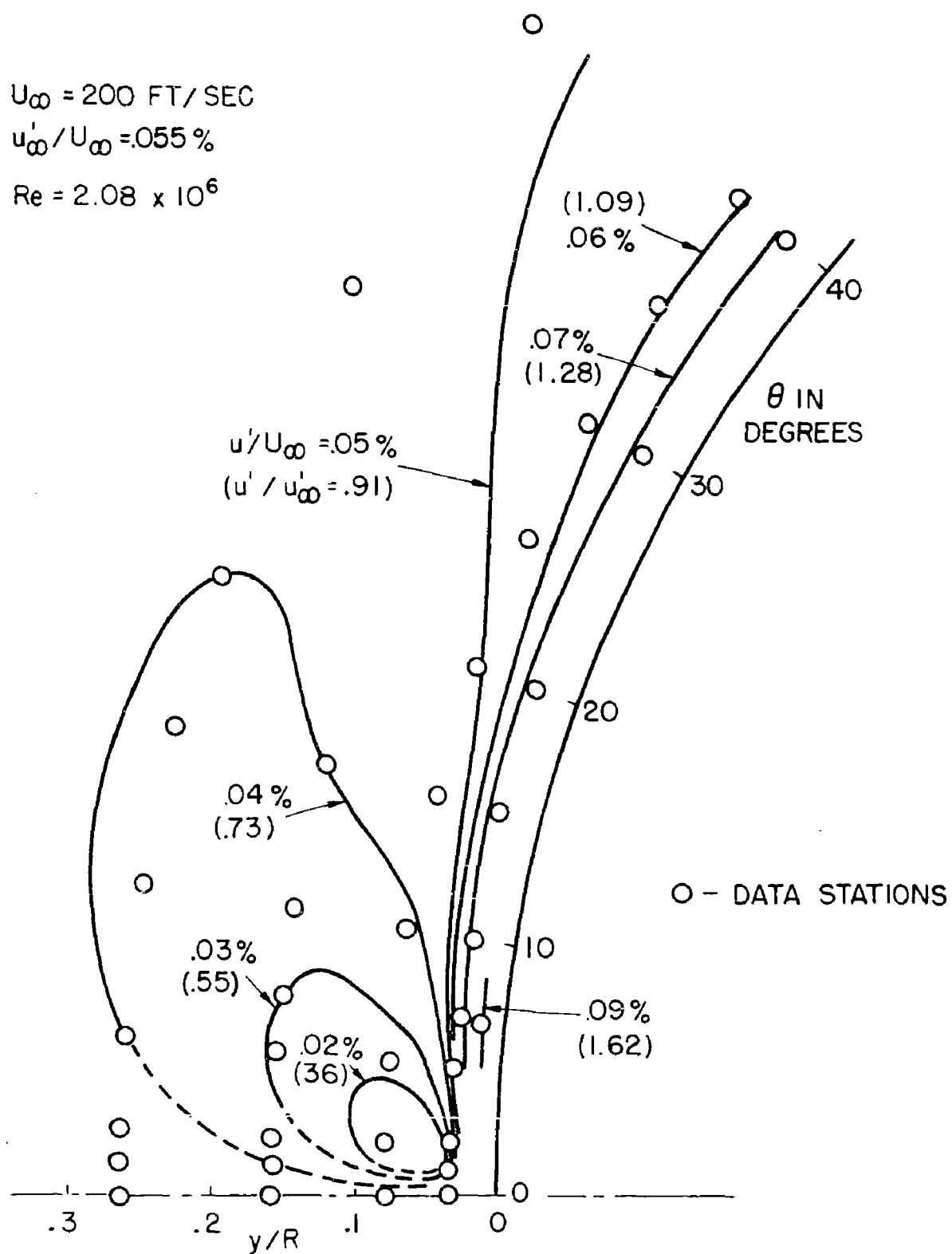
Fig.5 Turbulence contours near nose of 20-inch diameter body at Re = 2.08 \times 10^6 (Numbers in parentheses are u' / u'_{\infty} )
