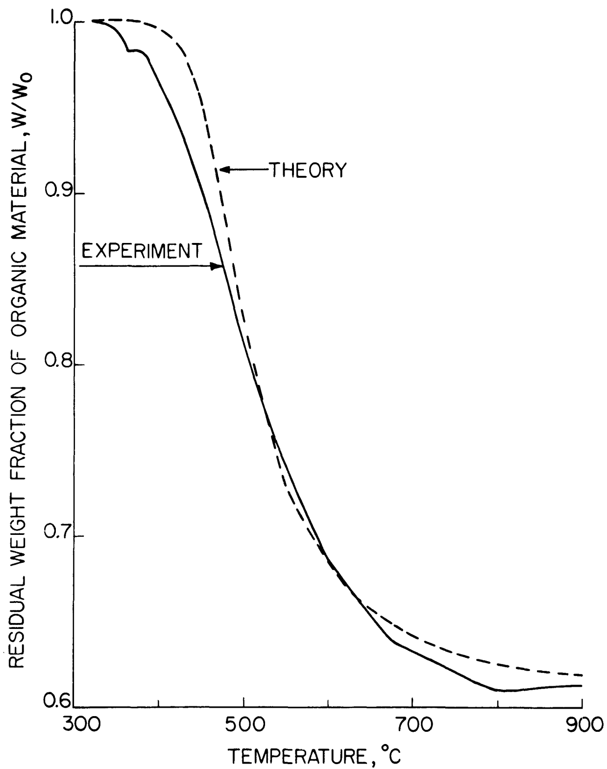
Figure 9. Experimental and Theoretical TGA Curves for the 50 ^{\circ}\text{C/hr.} Heating Rate.
