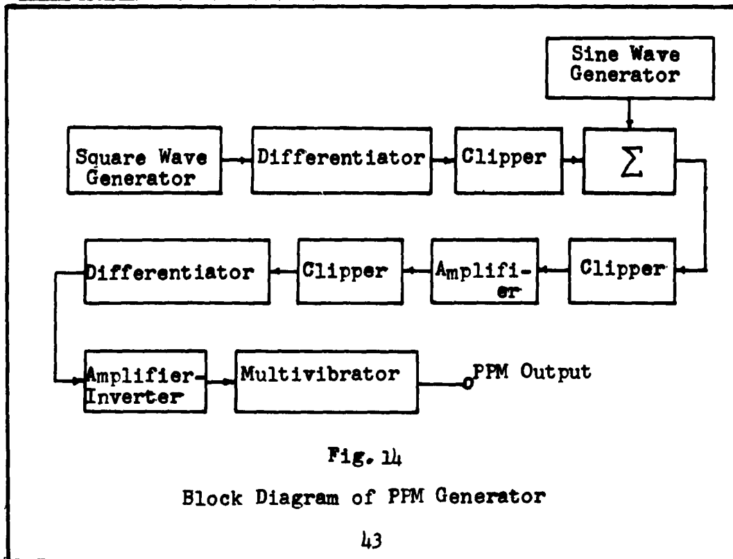
Block Diagram of PPM Generator
