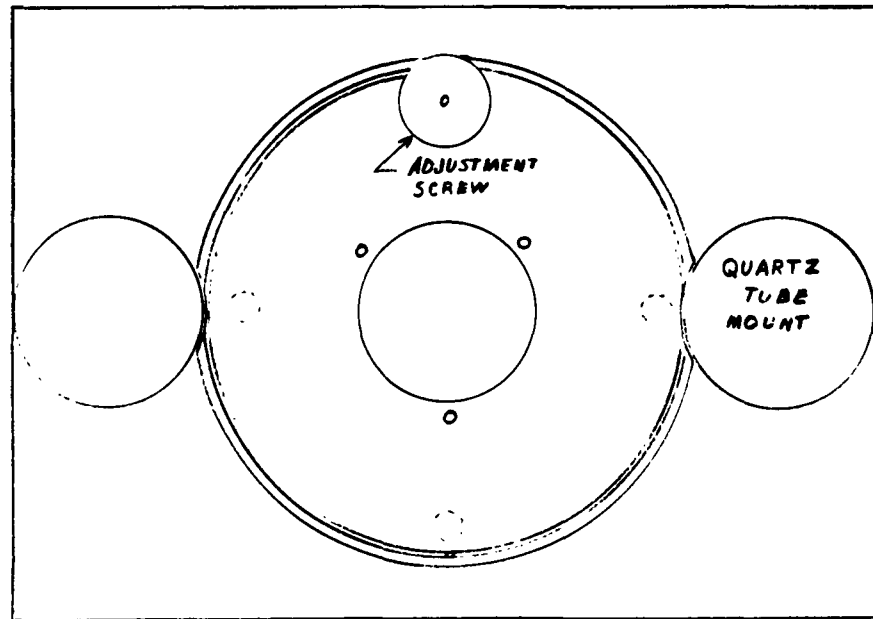
MIRROR GIMBAL MOUNT, END VIEW
