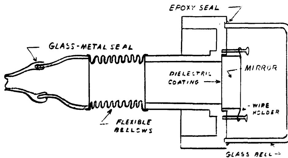
MIRROR HOLDER AND END BELL
