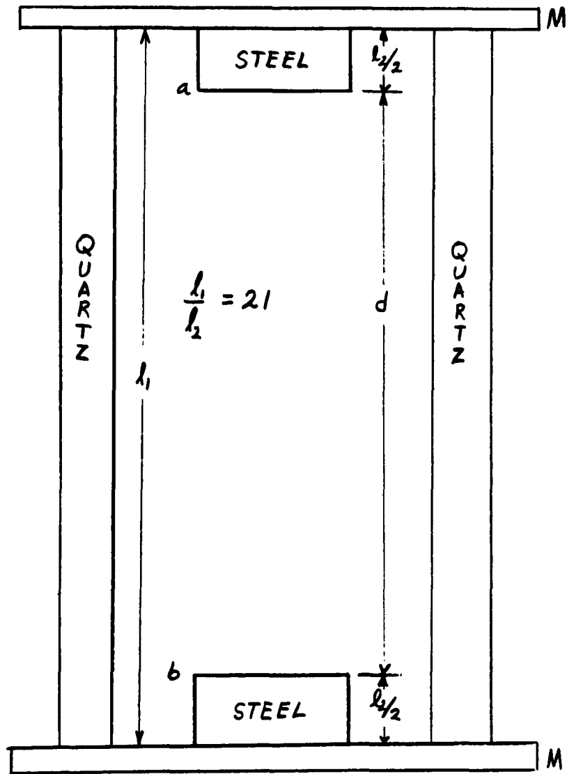
TEMPERATURE COMPENSATION ARRANGEMENT
