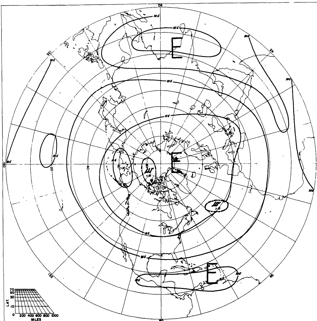
SPEED OF PREVAILING ZONAL WINDS JUNE 50 MB
