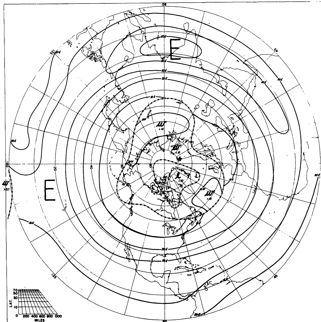
SPEED OF PREVAILING ZONAL WINDS AUGUST 50 MB
