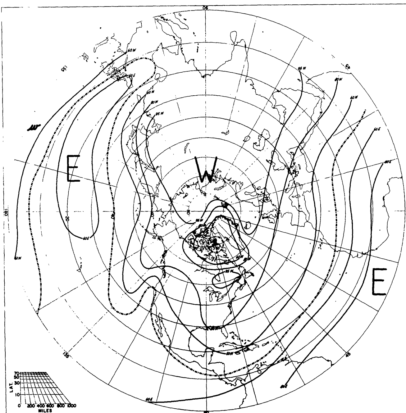
FREQUENCY OF PREVAILING ZONAL WINDS JANUARY 30 MB
