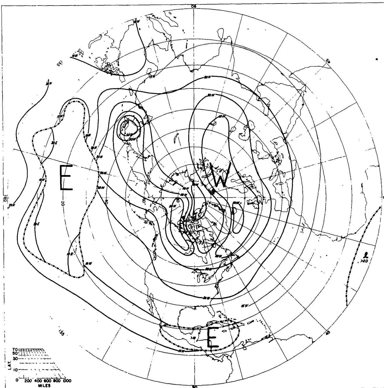
SPEED OF PREVAILING ZONAL WINDS JANUARY 50 MB
