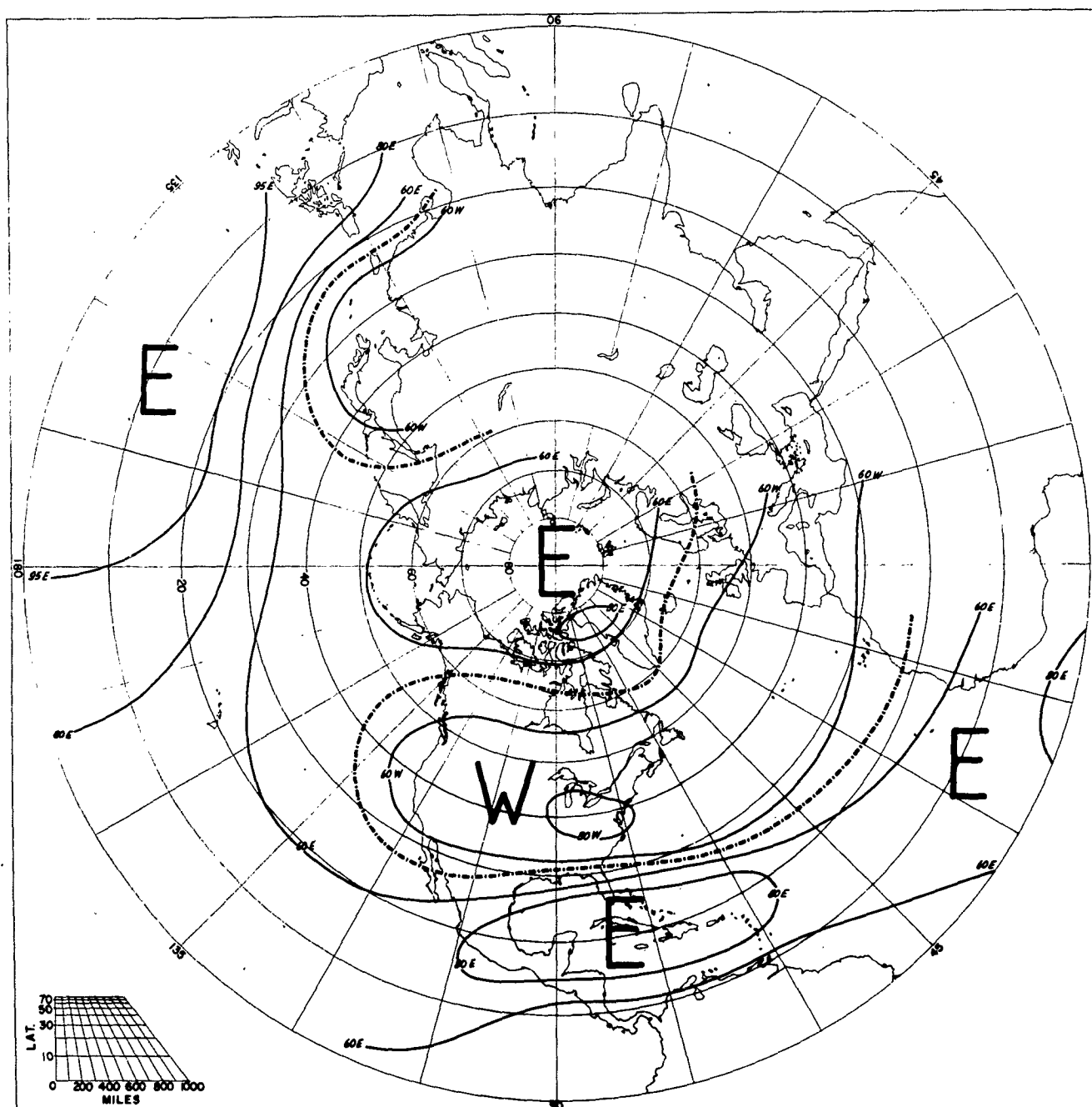
FREQUENCY OF PREVAILING ZONAL WINDS APRIL 10 MB
