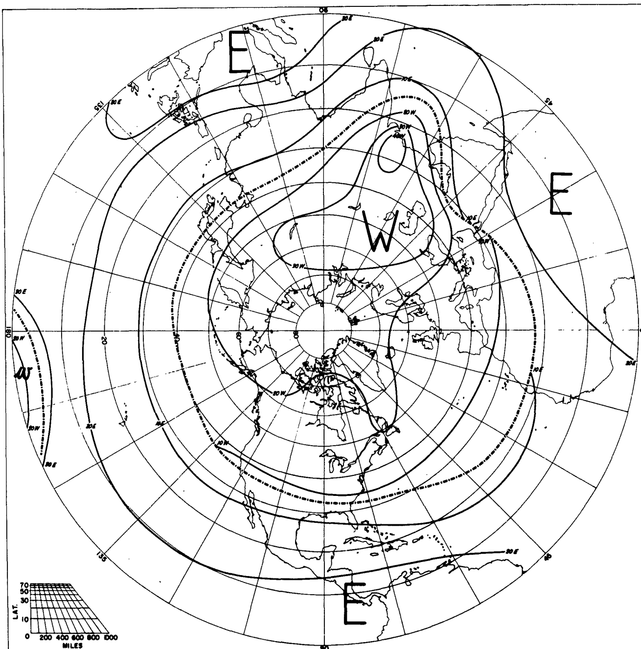
SPEED OF PREVAILING ZONAL WINDS OCTOBER 50 MB
