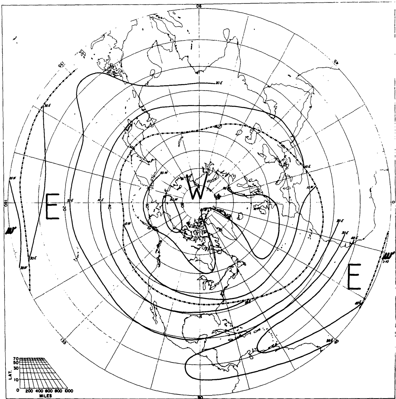
SPEED OF PREVAILING ZONAL WINDS OCTOBER 30 MB
