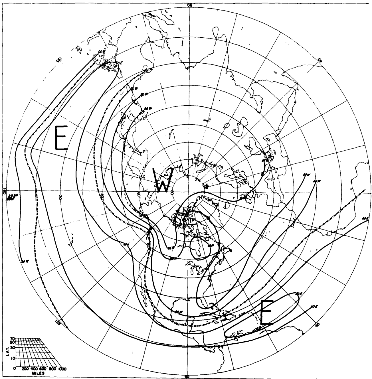
FREQUENCY OF PREVAILING ZONAL WINDS DECEMBER 30 MB
