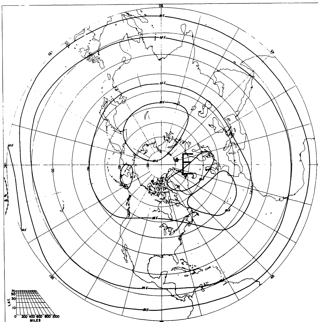
FREQUENCY OF PREVAILING ZONAL WINDS JULY 30 MB
