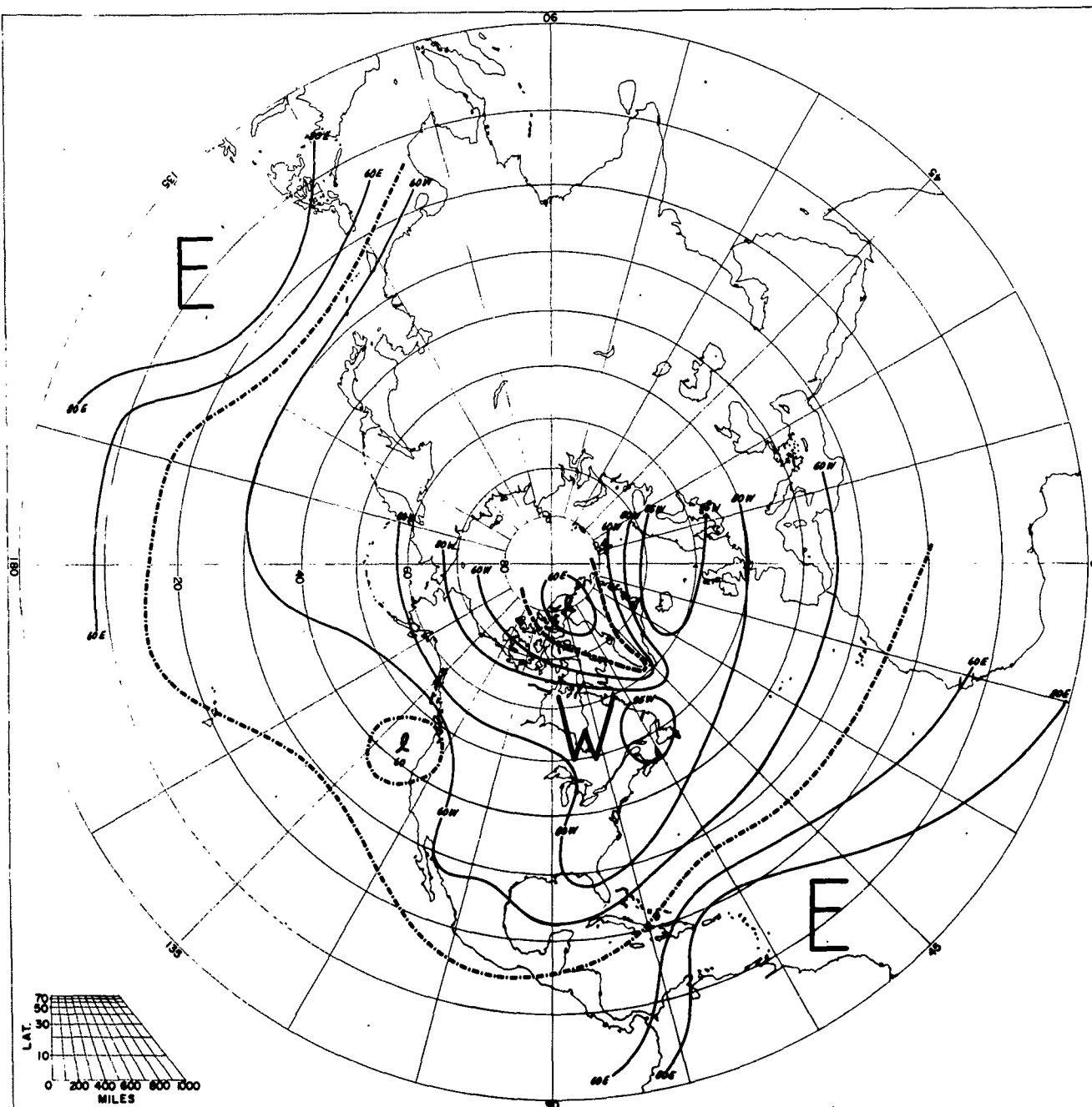
FREQUENCY OF PREVAILING ZONAL WINDS JANUARY 10 MB
