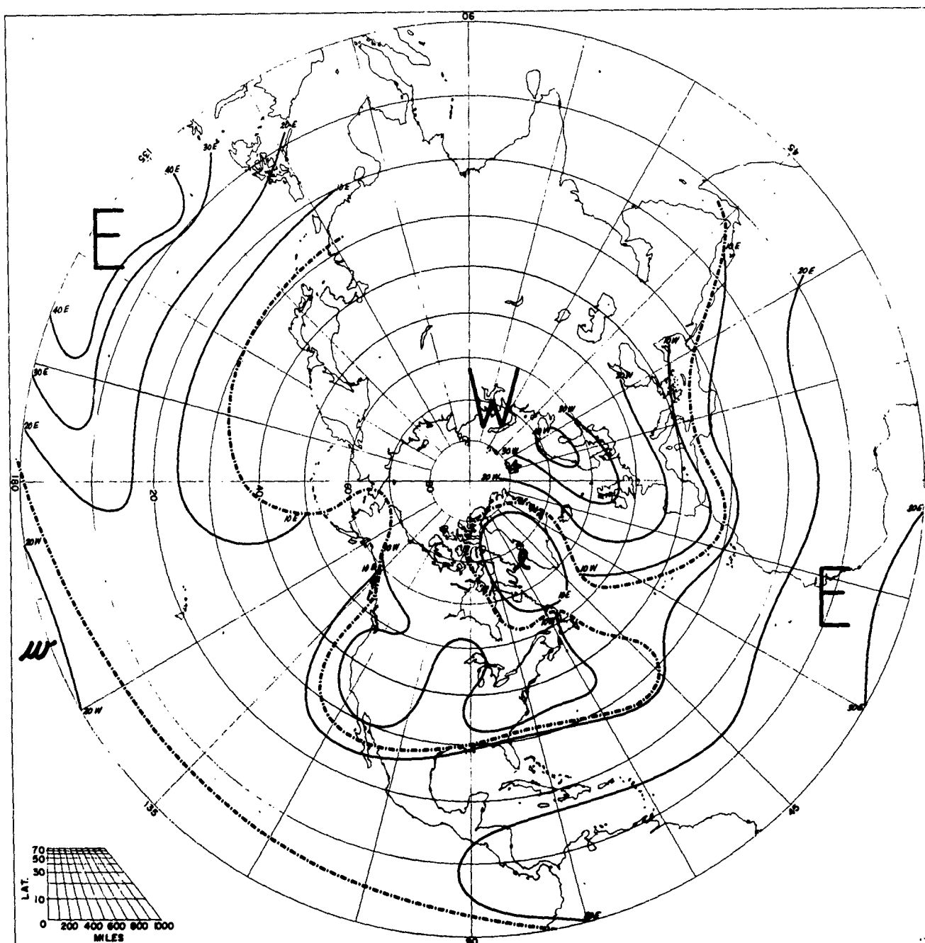
SPEED OF PREVAILING ZONAL WINDS APRIL 30 MB
