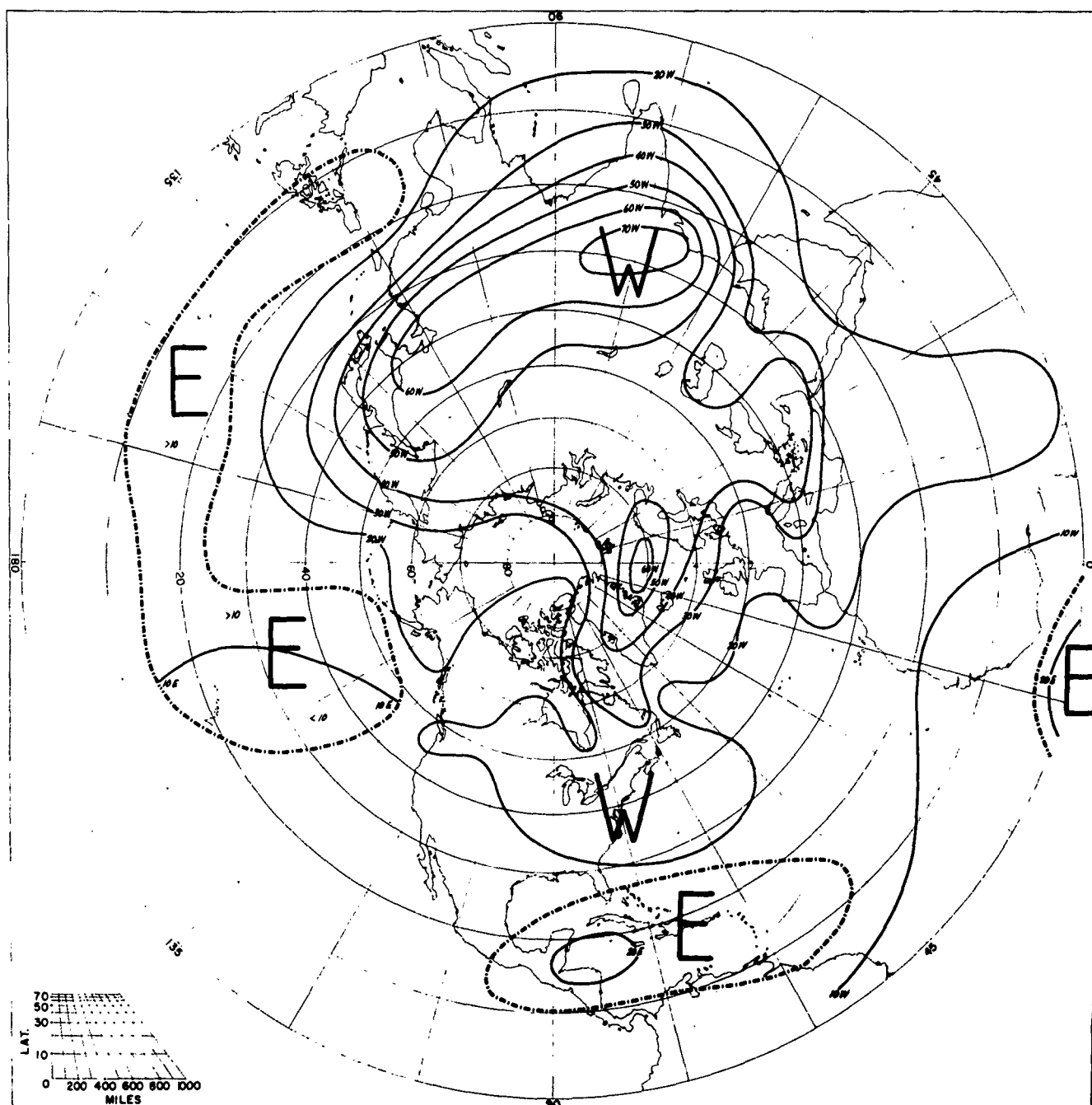
SPEED OF PREVAILING ZONAL WINDS FEBRUARY 50 MB
