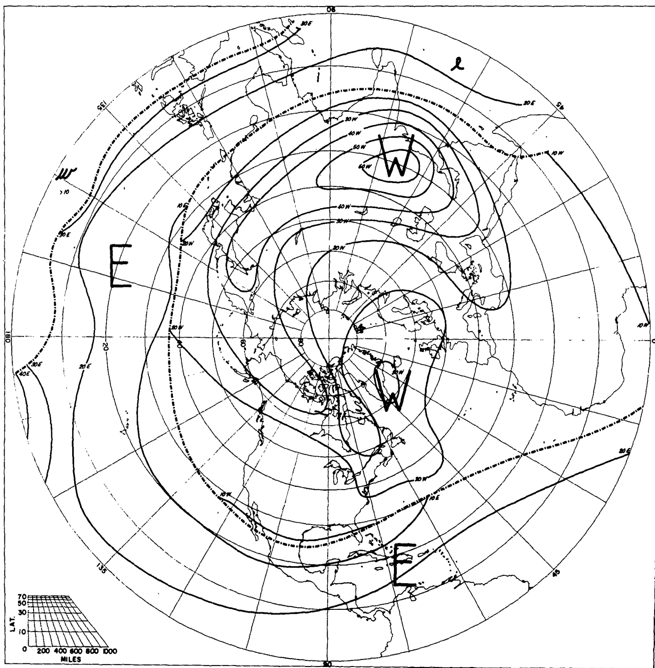
SPEED OF PREVAILING ZONAL WINDS NOVEMBER 50 MB
