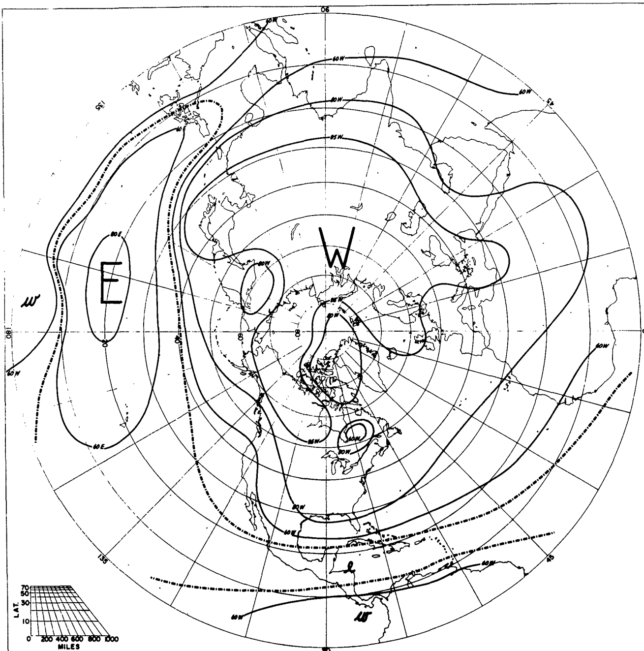
FREQUENCY OF PREVAILING ZONAL WINDS DECEMBER 50 MB
