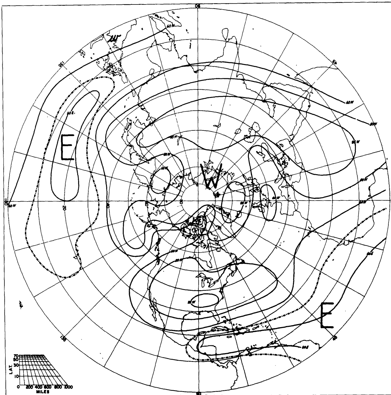
FREQUENCY OF PREVAILING ZONAL WINDS MARCH 50 MB
