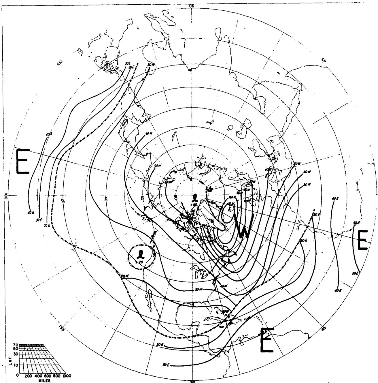
SPEED OF PREVAILING ZONAL WINDS JANUARY 10 MB
