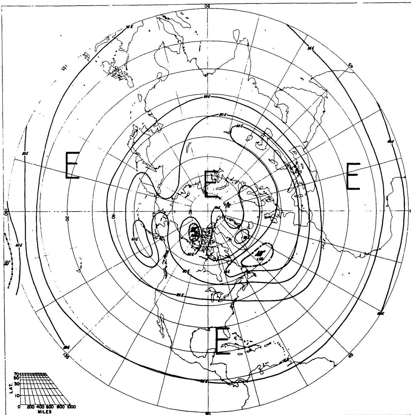
FREQUENCY OF PREVAILING ZONAL WINDS JULY 50 MB
