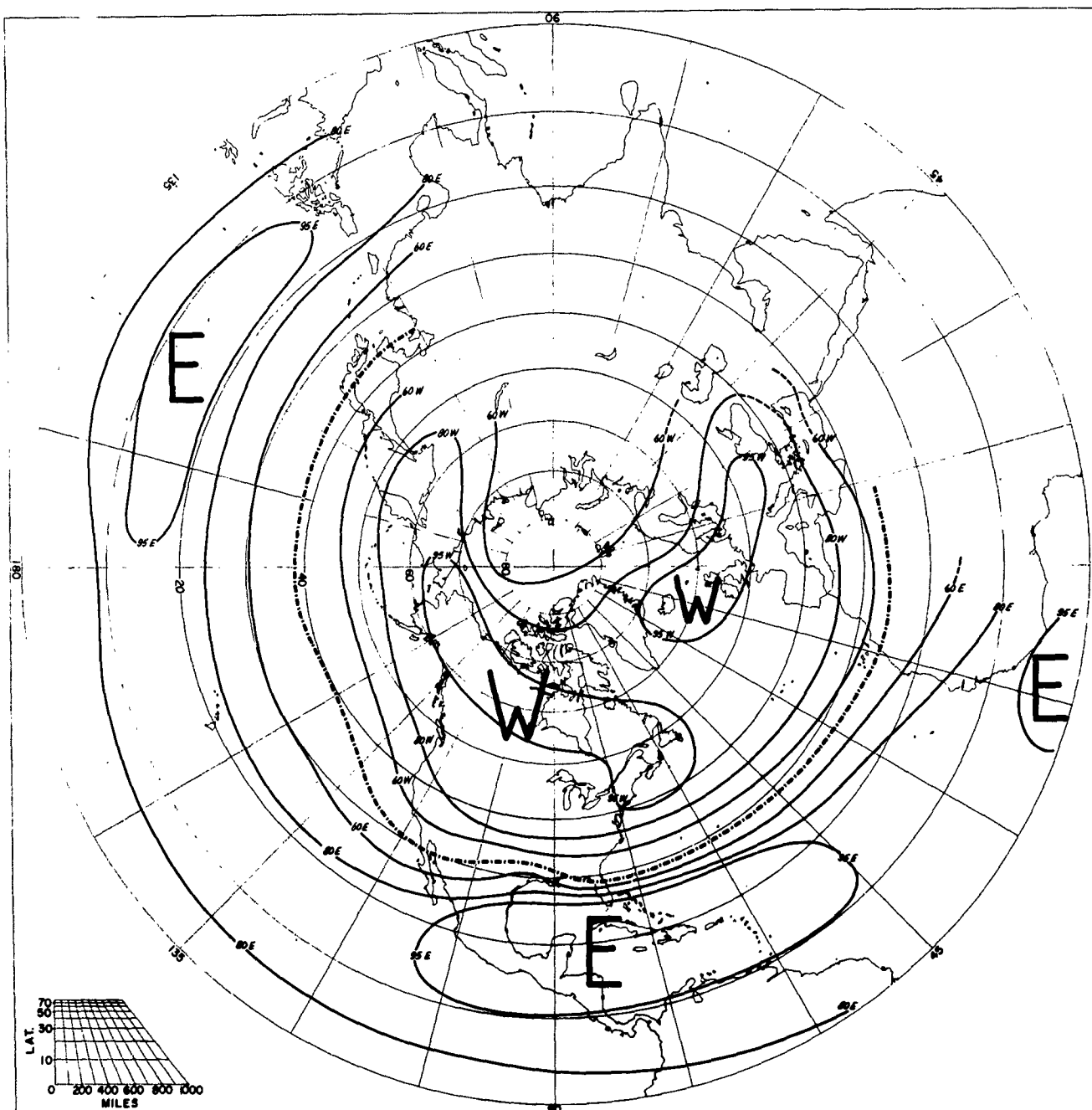
FREQUENCY OF PREVAILING ZONAL WINDS OCTOBER 10 MB
