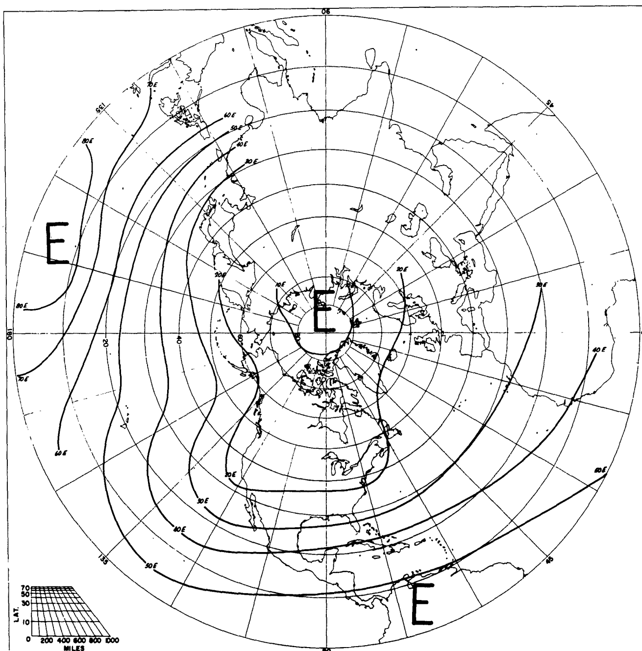
SPEED OF PREVAILING ZONAL WINDS JUNE 10 MB
