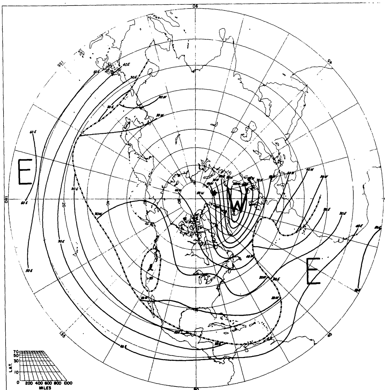
SPEED OF PREVAILING ZONAL WINDS FEBRUARY 10 MB
