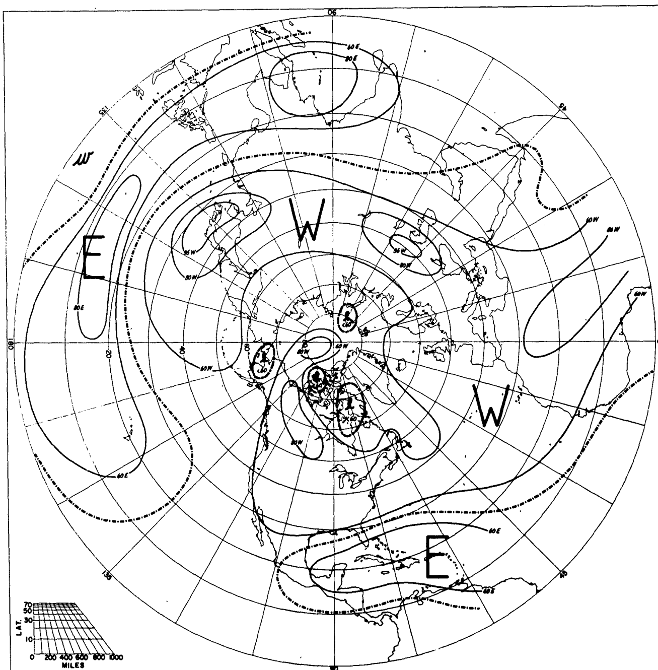
FREQUENCY OF PREVAILING ZONAL WINDS APRIL 50 MB
