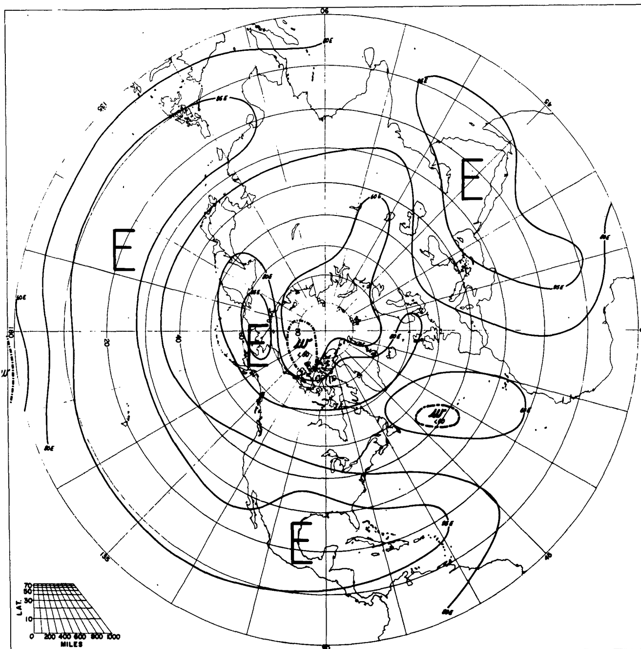
FREQUENCY OF PREVAILING ZONAL WINDS JUNE 50 MB
