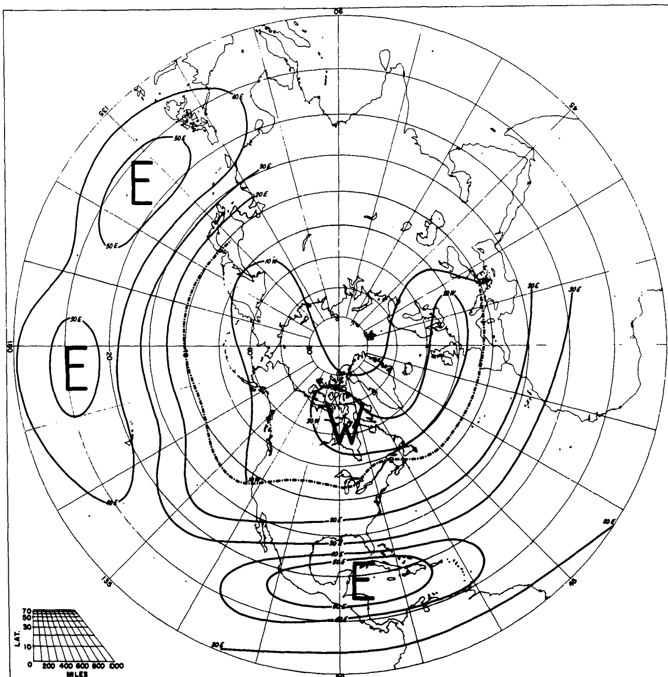
SPEED OF PREVAILING ZONAL WINDS SEPTEMBER 10 MB
