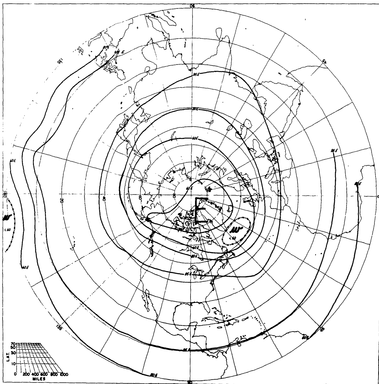
FREQUENCY OF PREVAILING ZONAL WINDS AUGUST 30 MB
