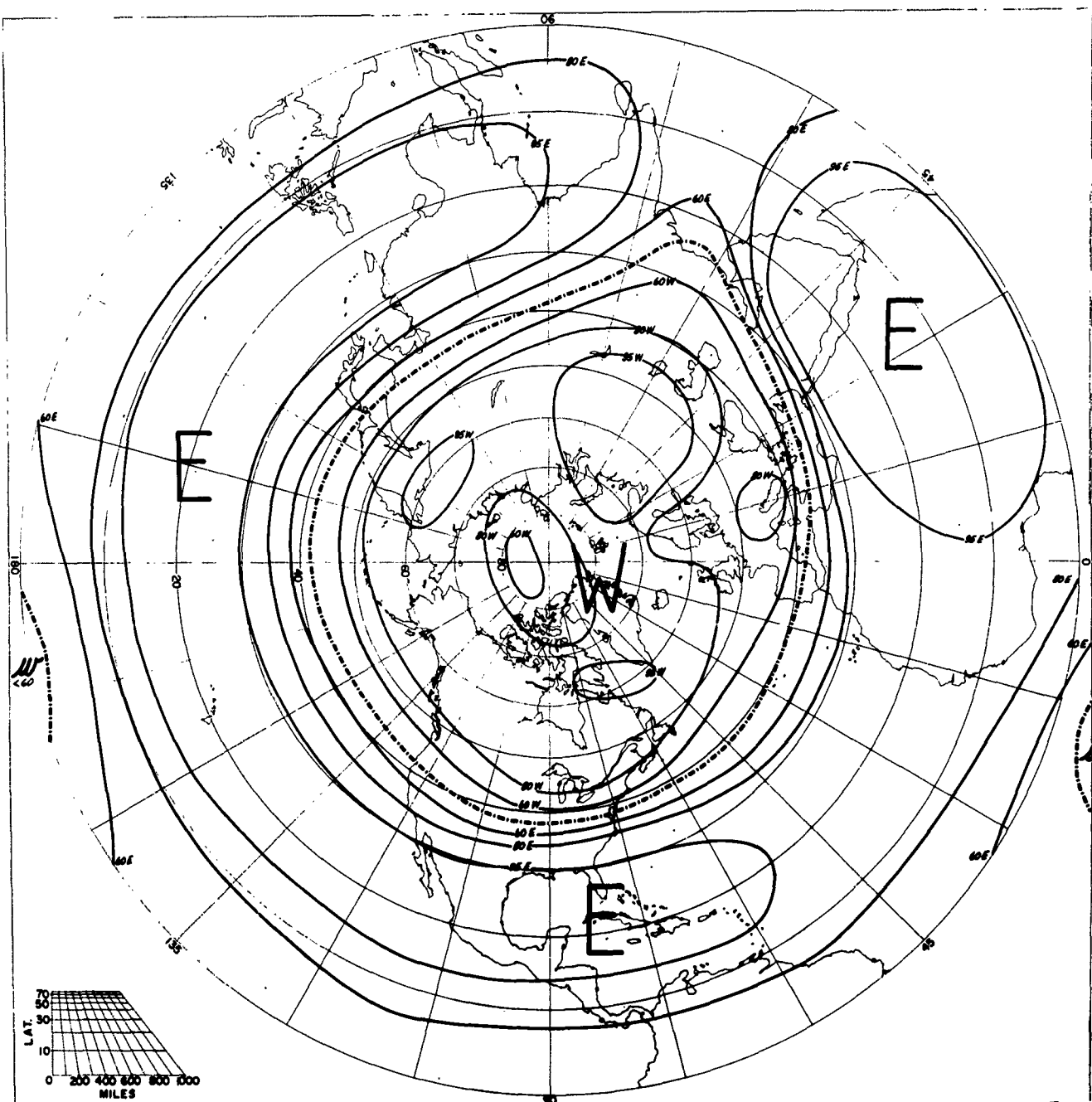
FREQUENCY OF PREVAILING ZONAL WINDS SEPTEMBER 50 MB
