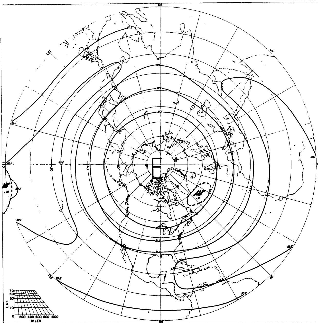
SPEED OF PREVAILING ZONAL WINDS AUGUST 30 MB
