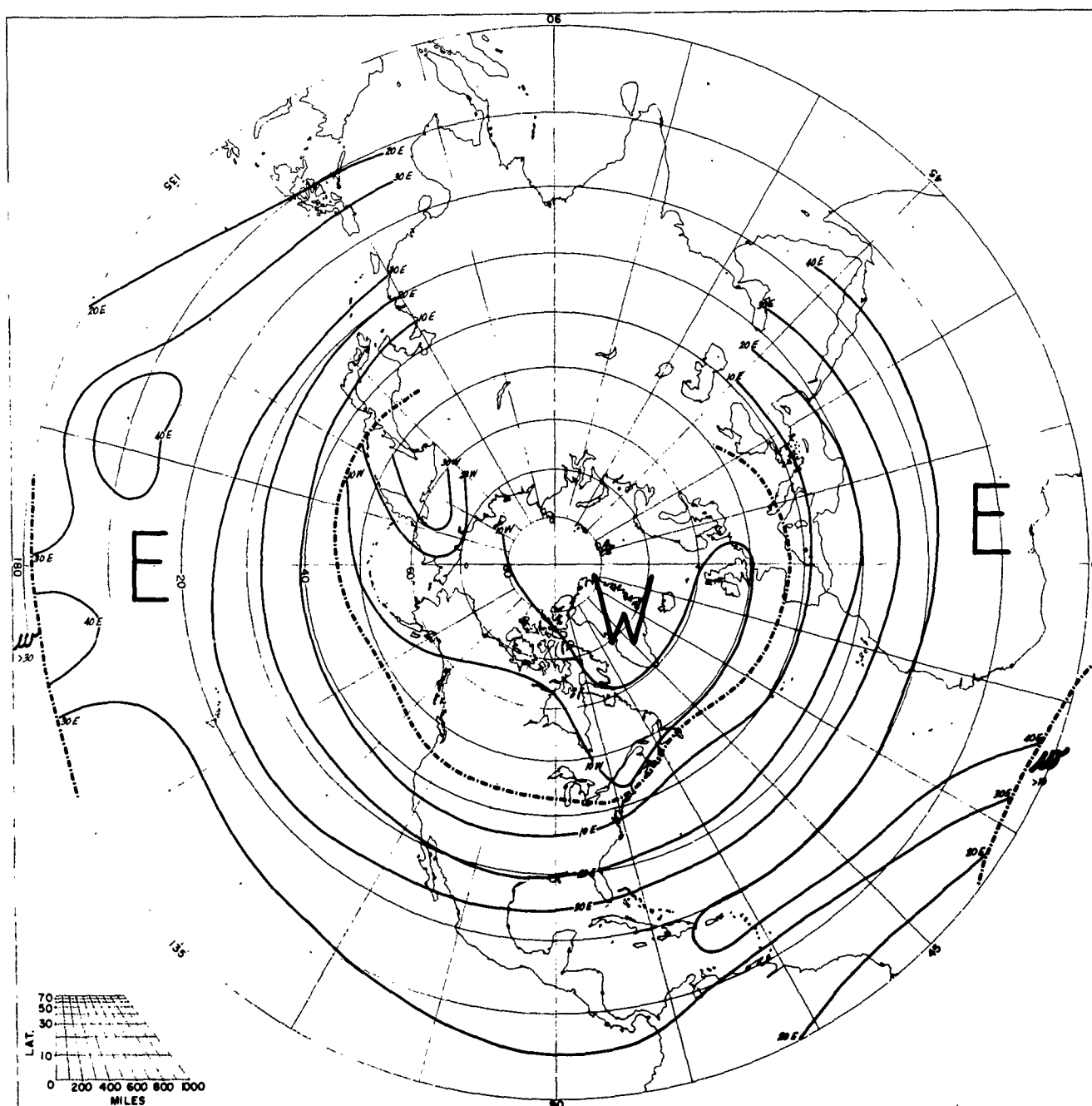
SPEED OF PREVAILING ZONAL WINDS SEPTEMBER 30 MB
