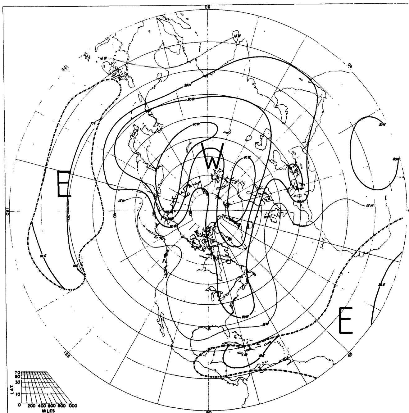
SPEED OF PREVAILING ZONAL WINDS MARCH 50 MB
