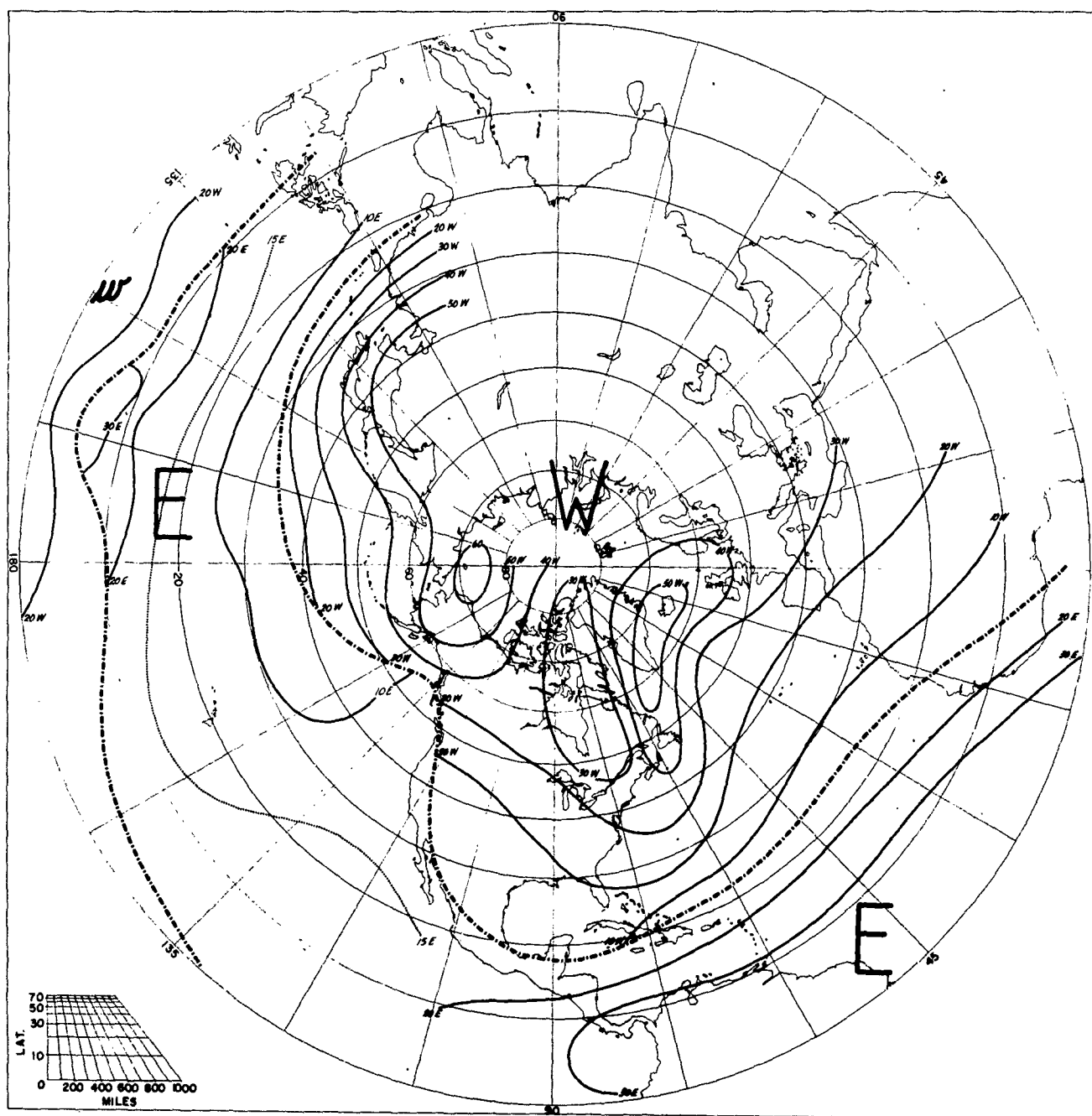
SPEED OF PREVAILING ZONAL WINDS DECEMBER 30 MB
