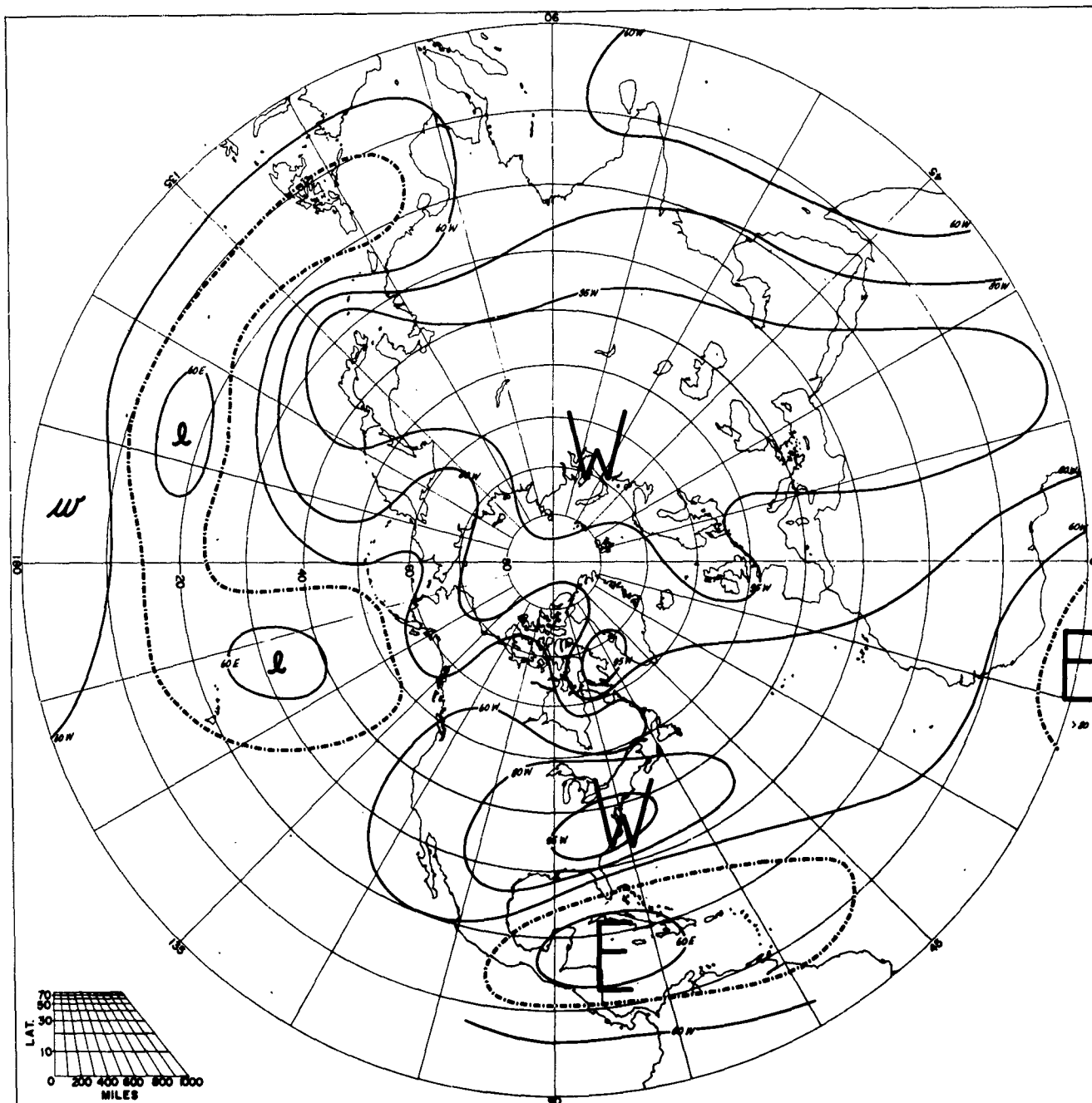
FREQUENCY OF PREVAILING ZONAL WINDS FEBRUARY 50 MB
