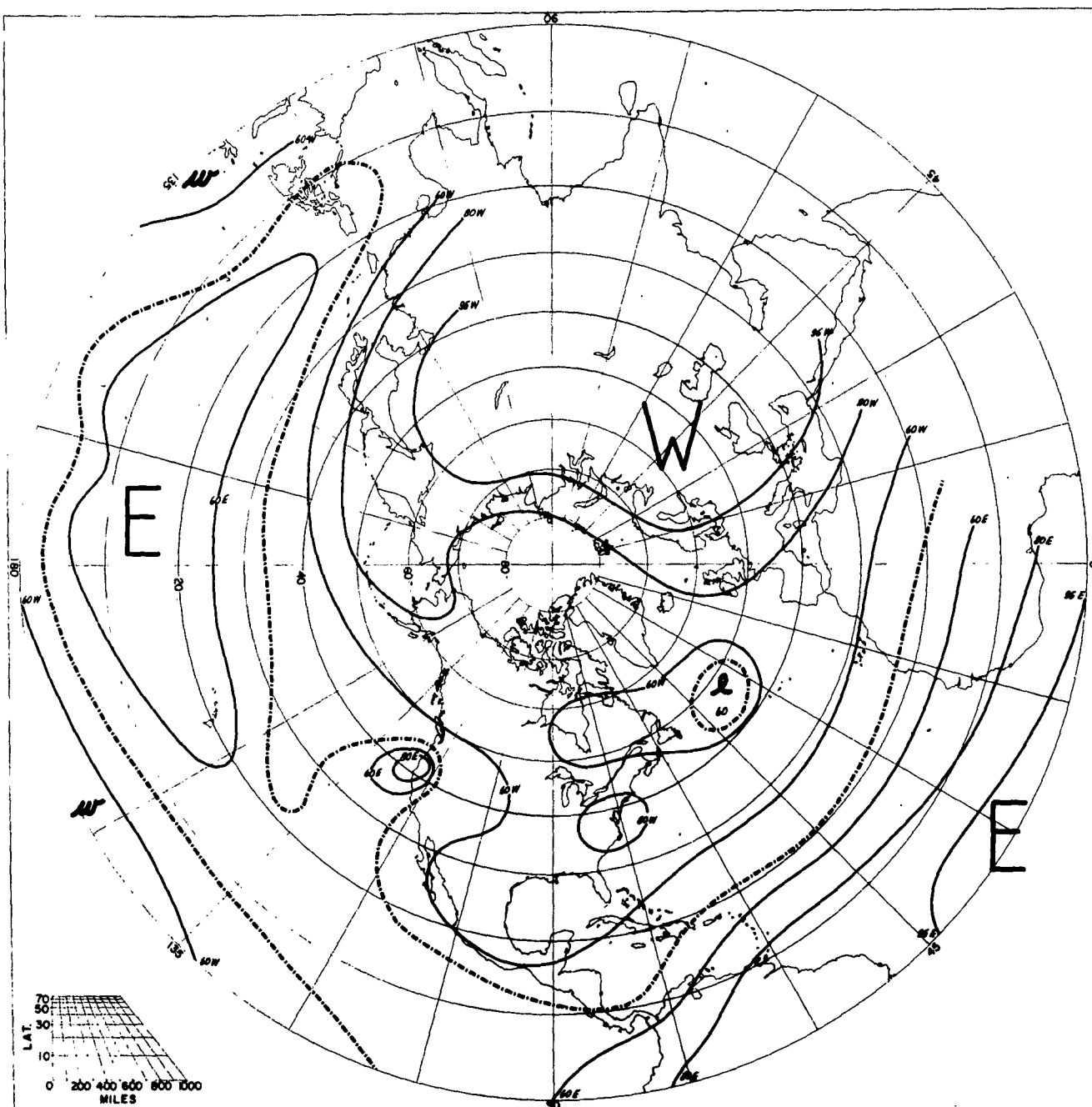
FREQUENCY OF PREVAILING ZONAL WINDS FEBRUARY 30 MB
