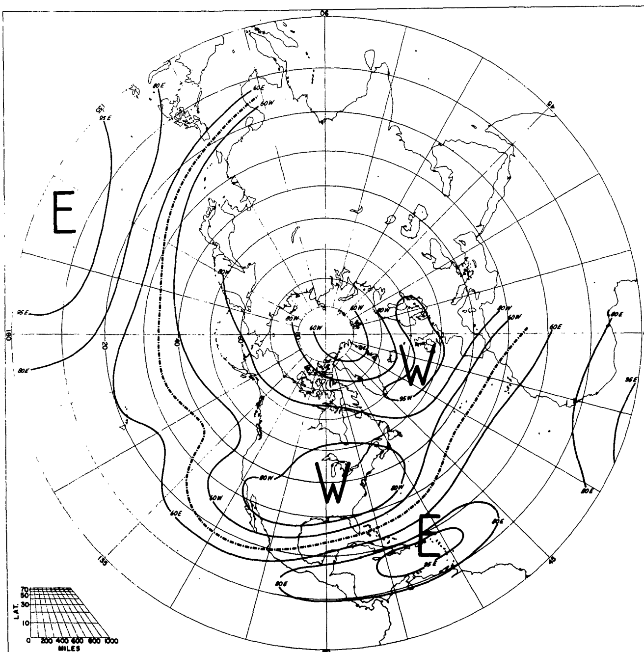
FREQUENCY OF PREVAILING ZONAL WINDS MARCH 10 MB
