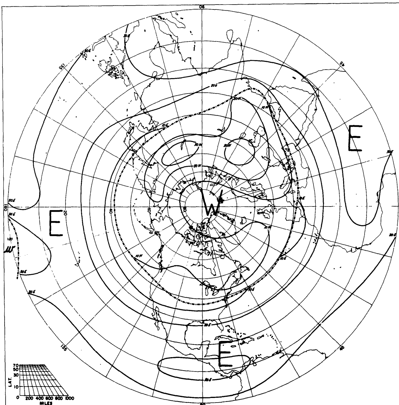
SPEED OF PREVAILING ZONAL WINDS SEPTEMBER 50 MB
