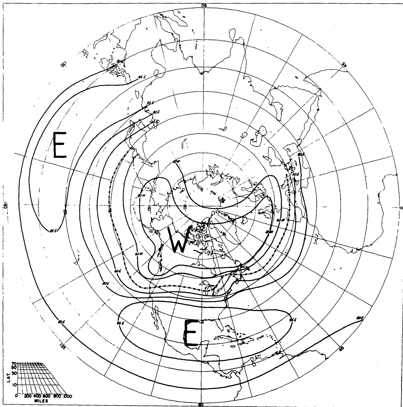
FREQUENCY OF PREVAILING ZONAL WINDS SEPTEMBER 10 MB
