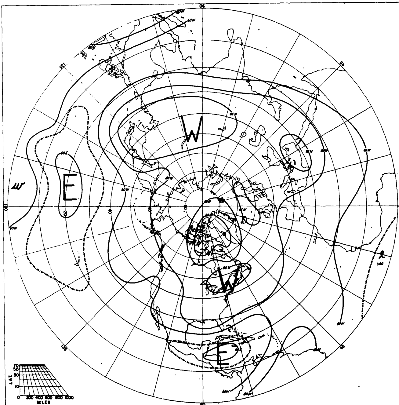
FREQUENCY OF PREVAILING ZONAL WINDS JANUARY 50 MB
