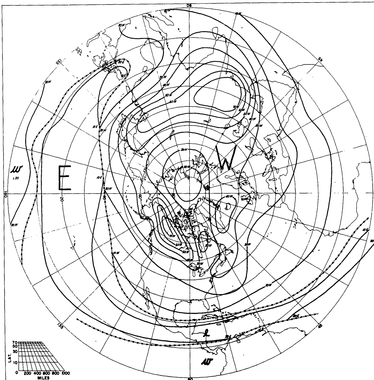
SPEED OF PREVAILING ZONAL WINDS DECEMBER 50 MB
