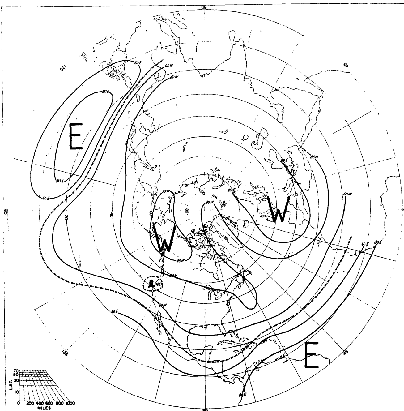
FREQUENCY OF PREVAILING ZONAL WINDS DECEMBER 10 MB
