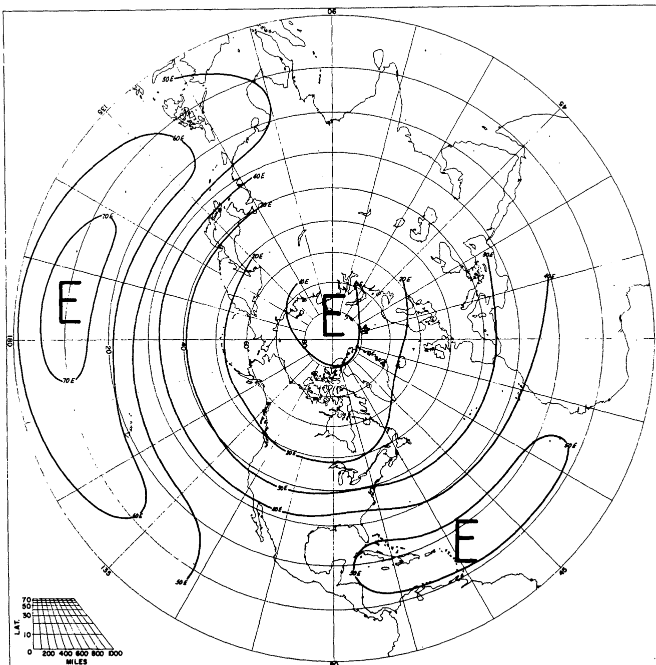
SPEED OF PREVAILING ZONAL WINDS JULY 10 MB
