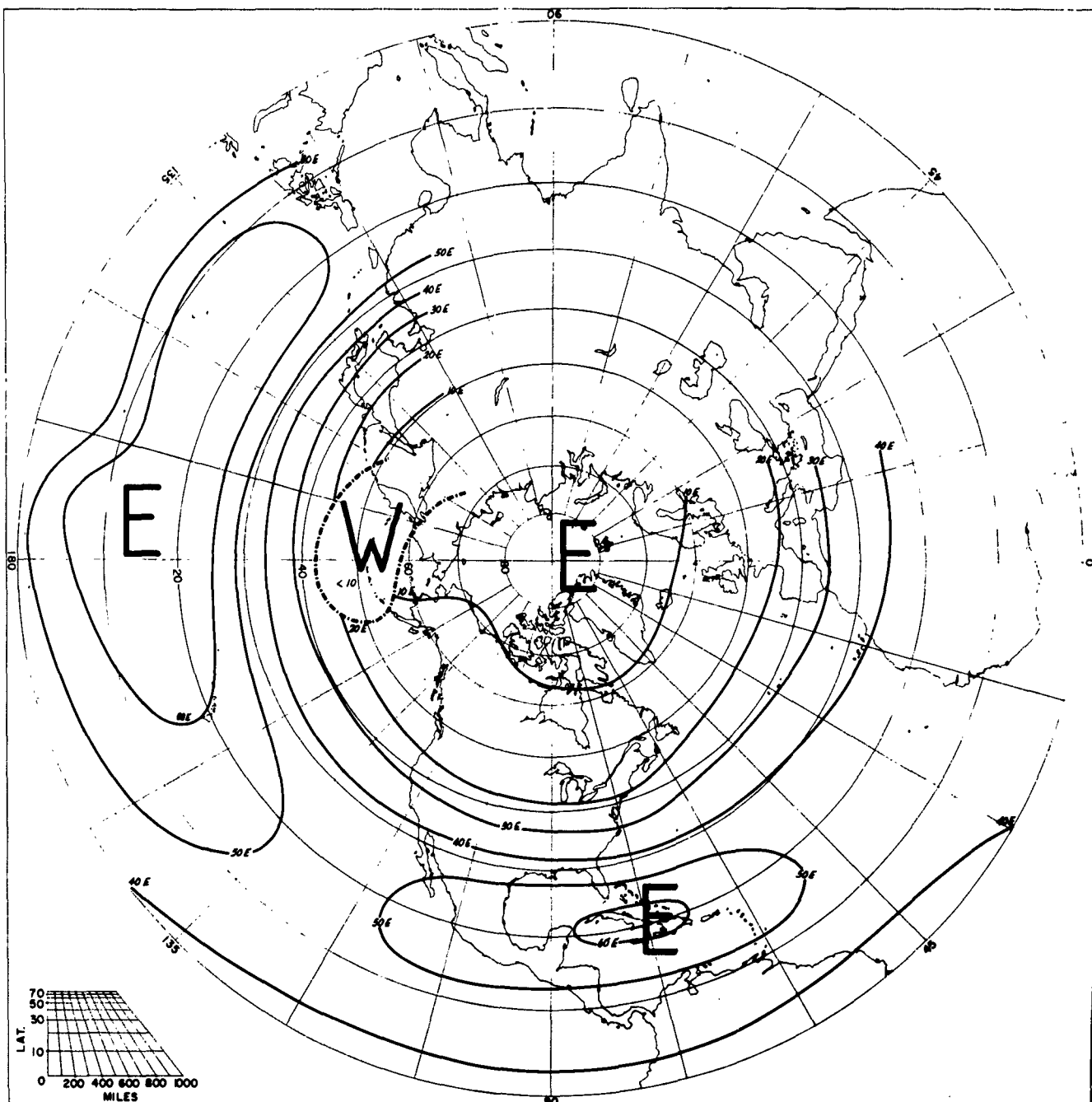
SPEED OF PREVAILING ZONAL WINDS AUGUST 10 MB
