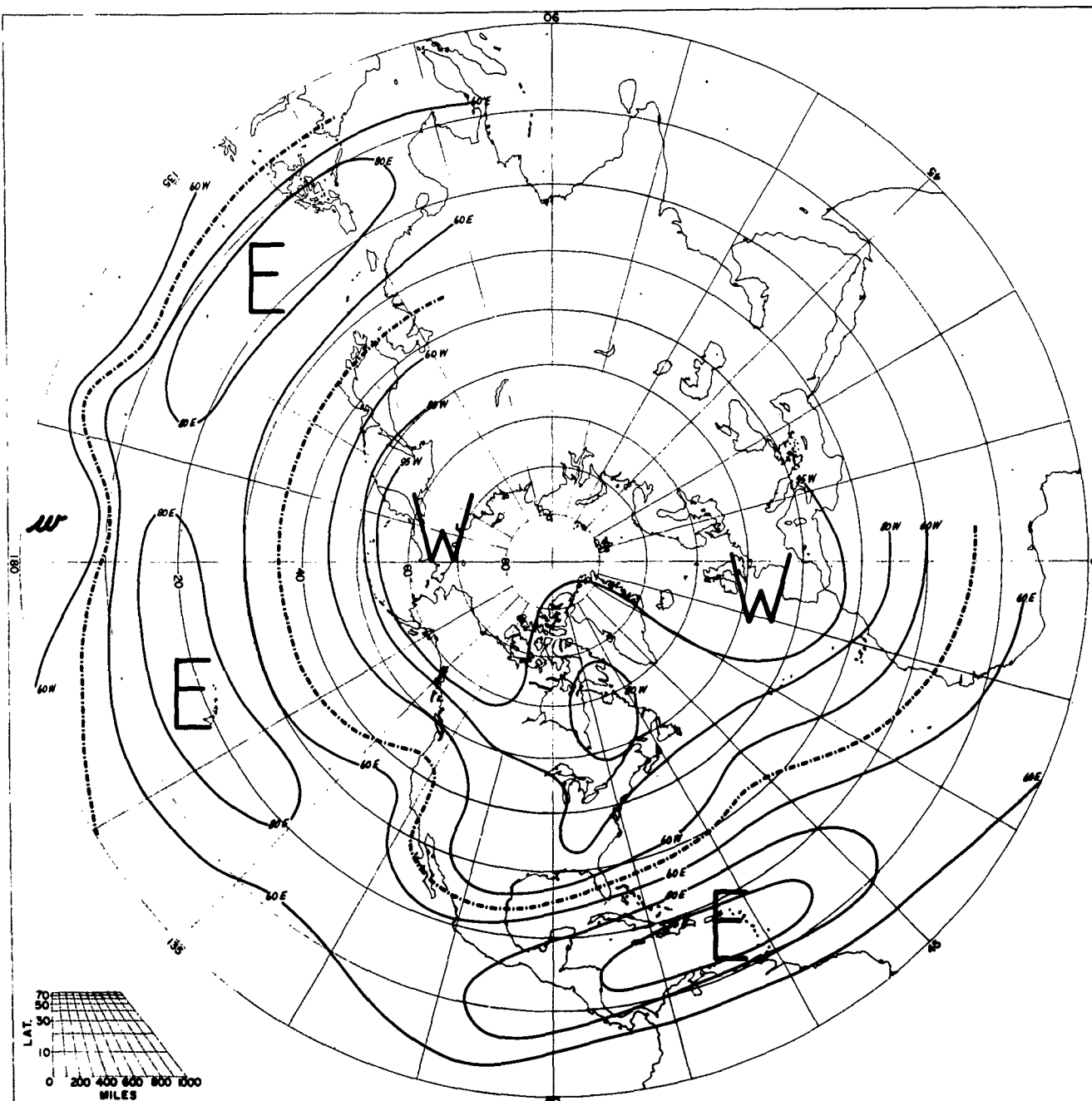
FREQUENCY OF PREVAILING ZONAL WINDS NOVEMBER 30 MB
