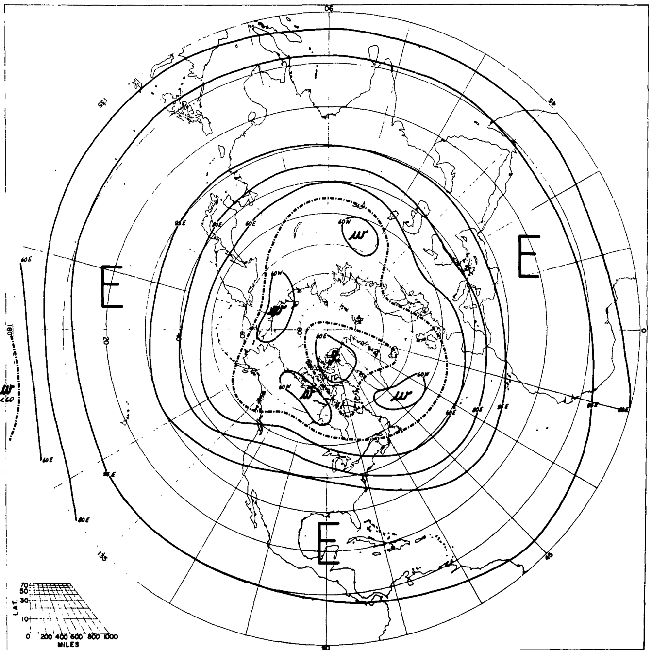
FREQUENCY OF PREVAILING ZONAL WINDS AUGUST 50 MB
