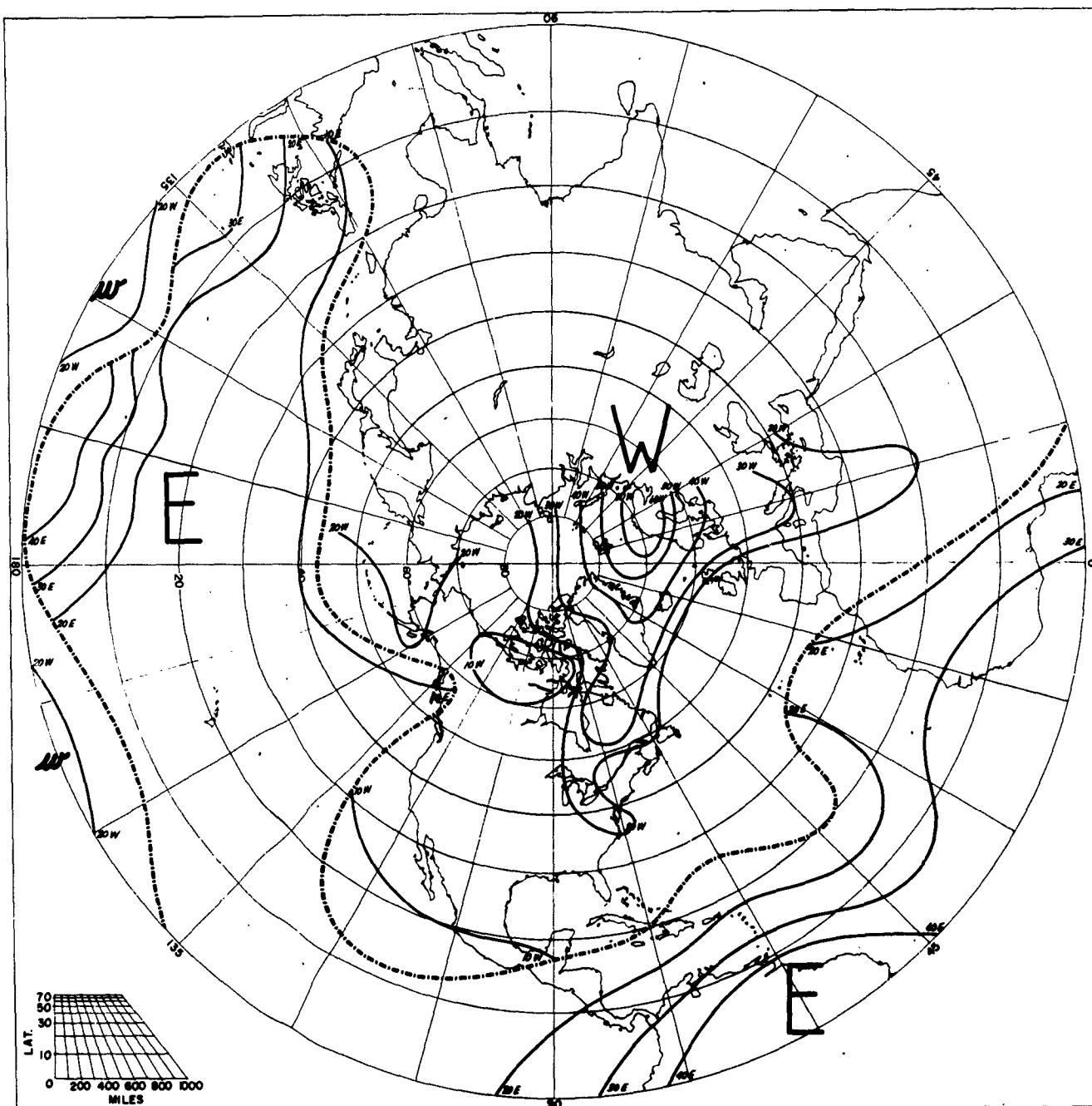
SPEED OF PREVAILING ZONAL WINDS MARCH 30 MB
