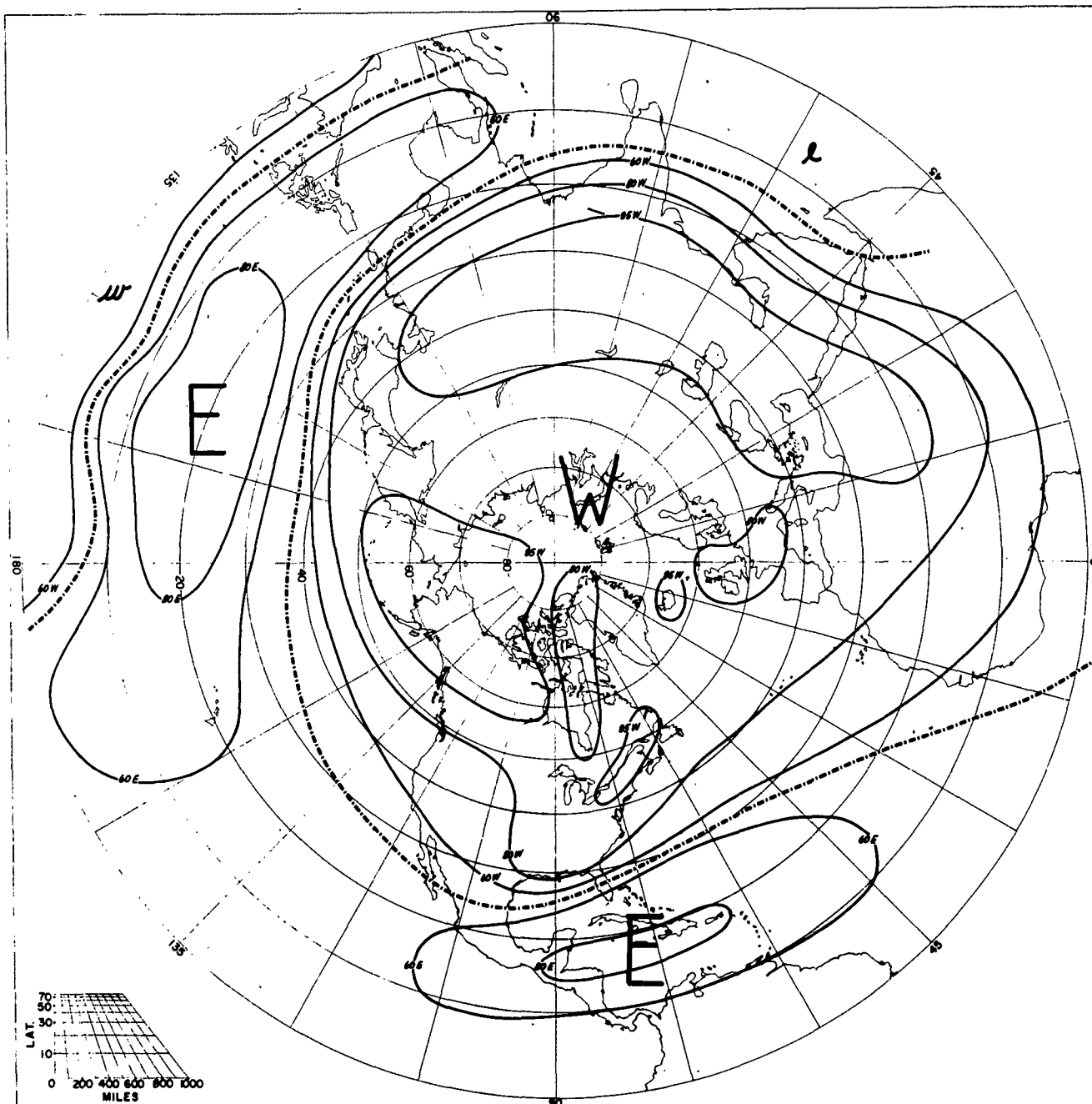
FREQUENCY OF PREVAILING ZONAL WINDS NOVEMBER 50 MB
