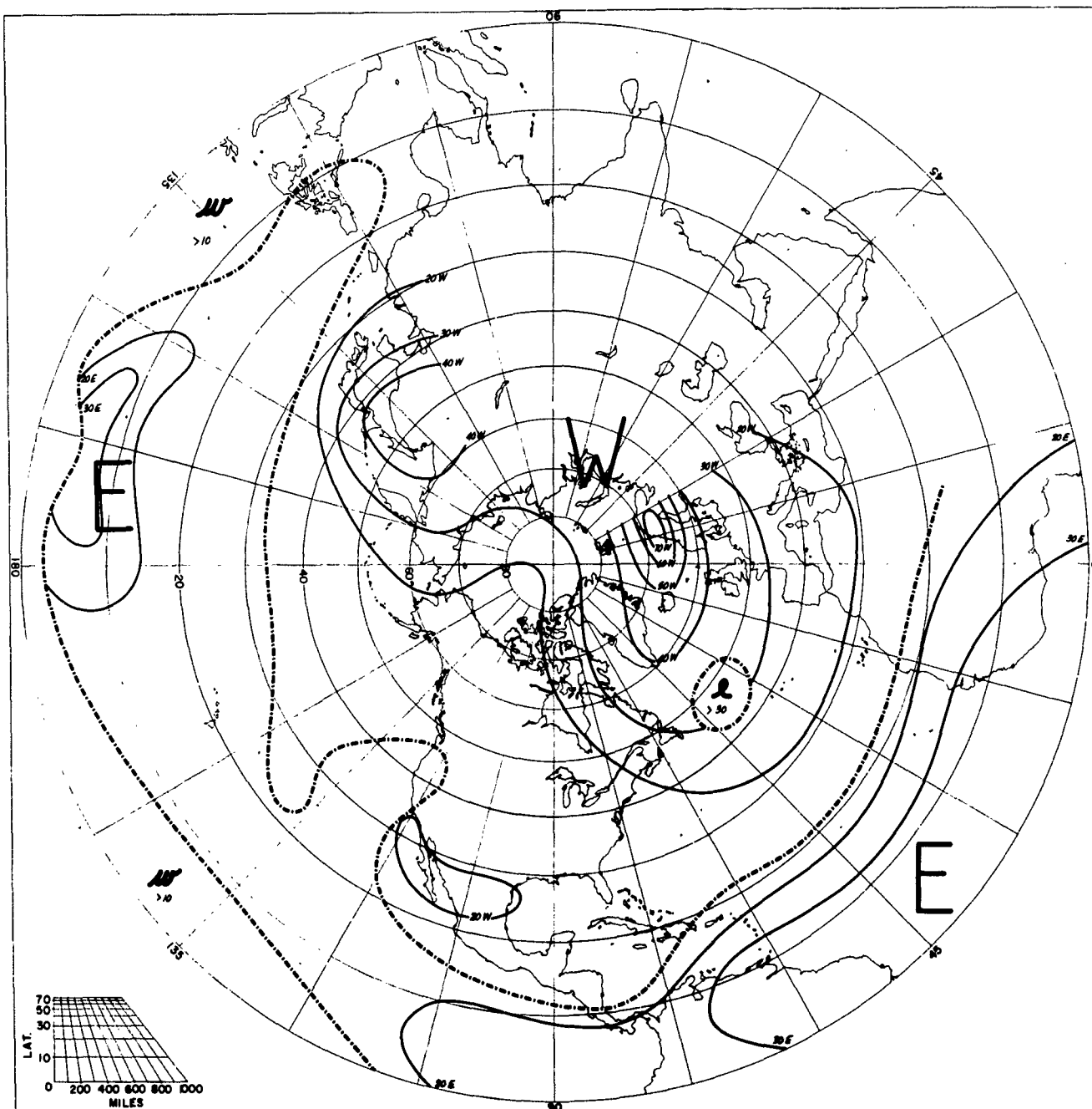
SPEED OF PREVAILING ZONAL WINDS FEBRUARY 30 MB
