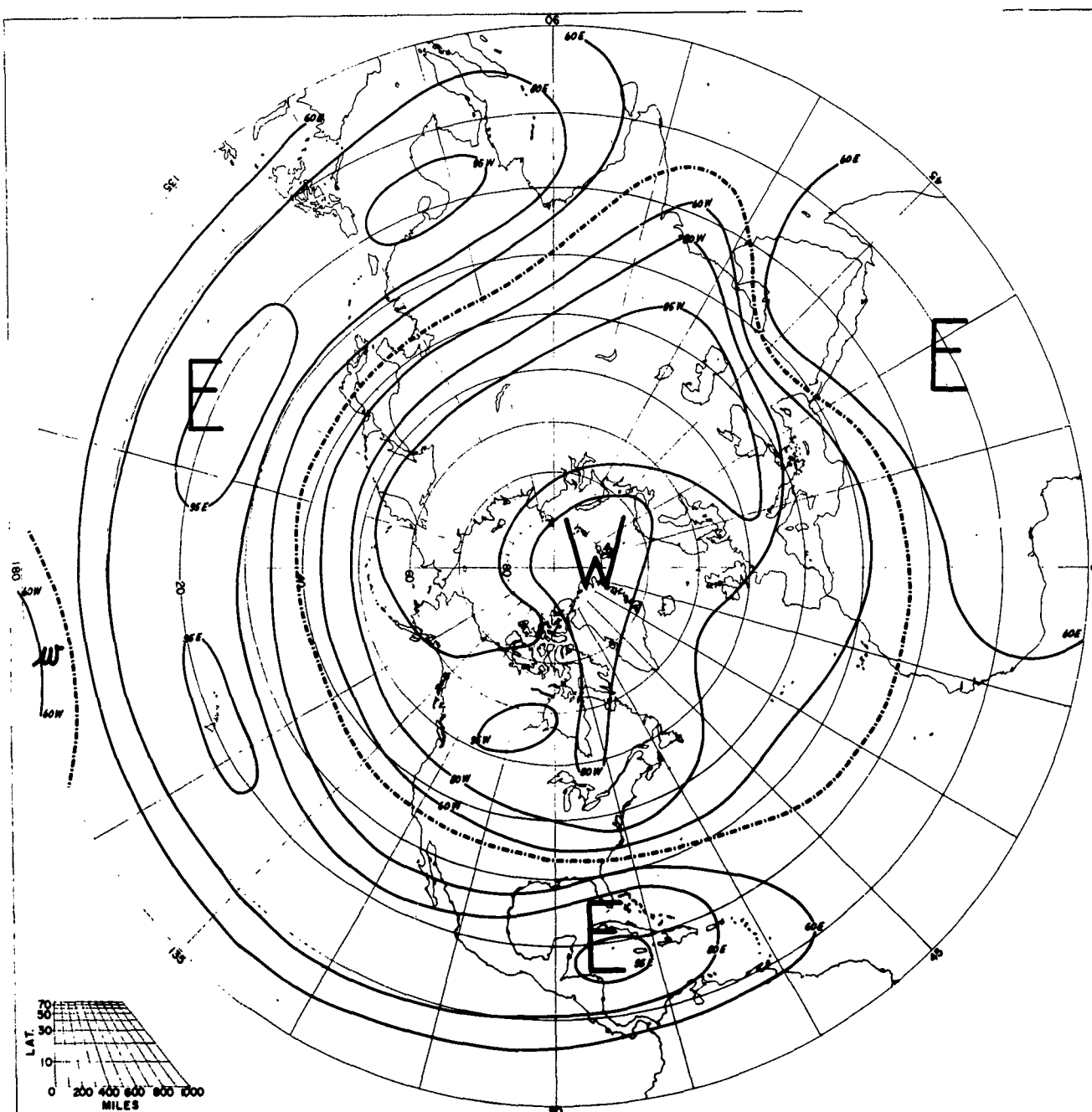
FREQUENCY OF PREVAILING ZONAL WINDS OCTOBER 50 MB
