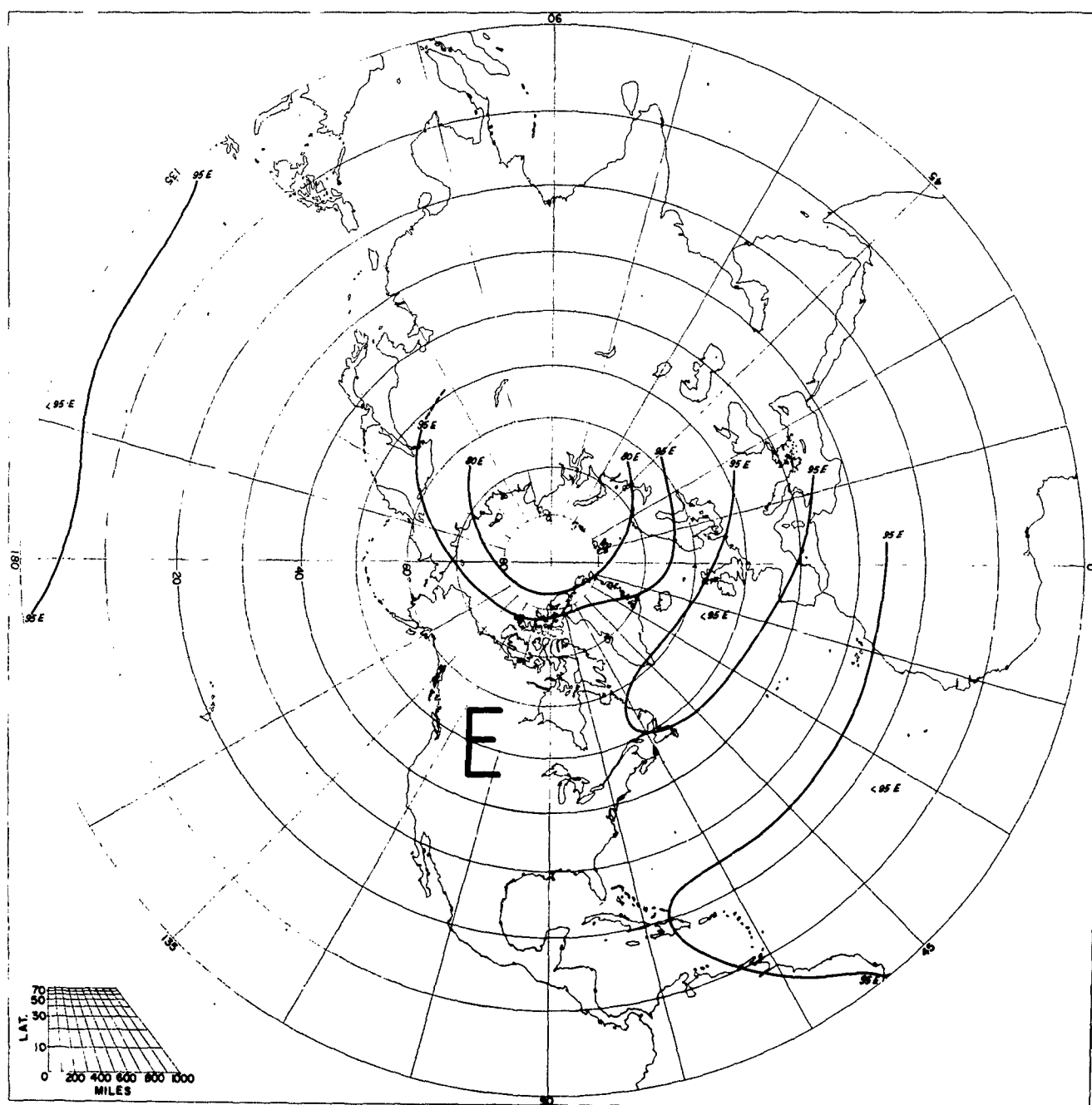
FREQUENCY OF PREVAILING ZONAL WINDS JULY 10 MB
