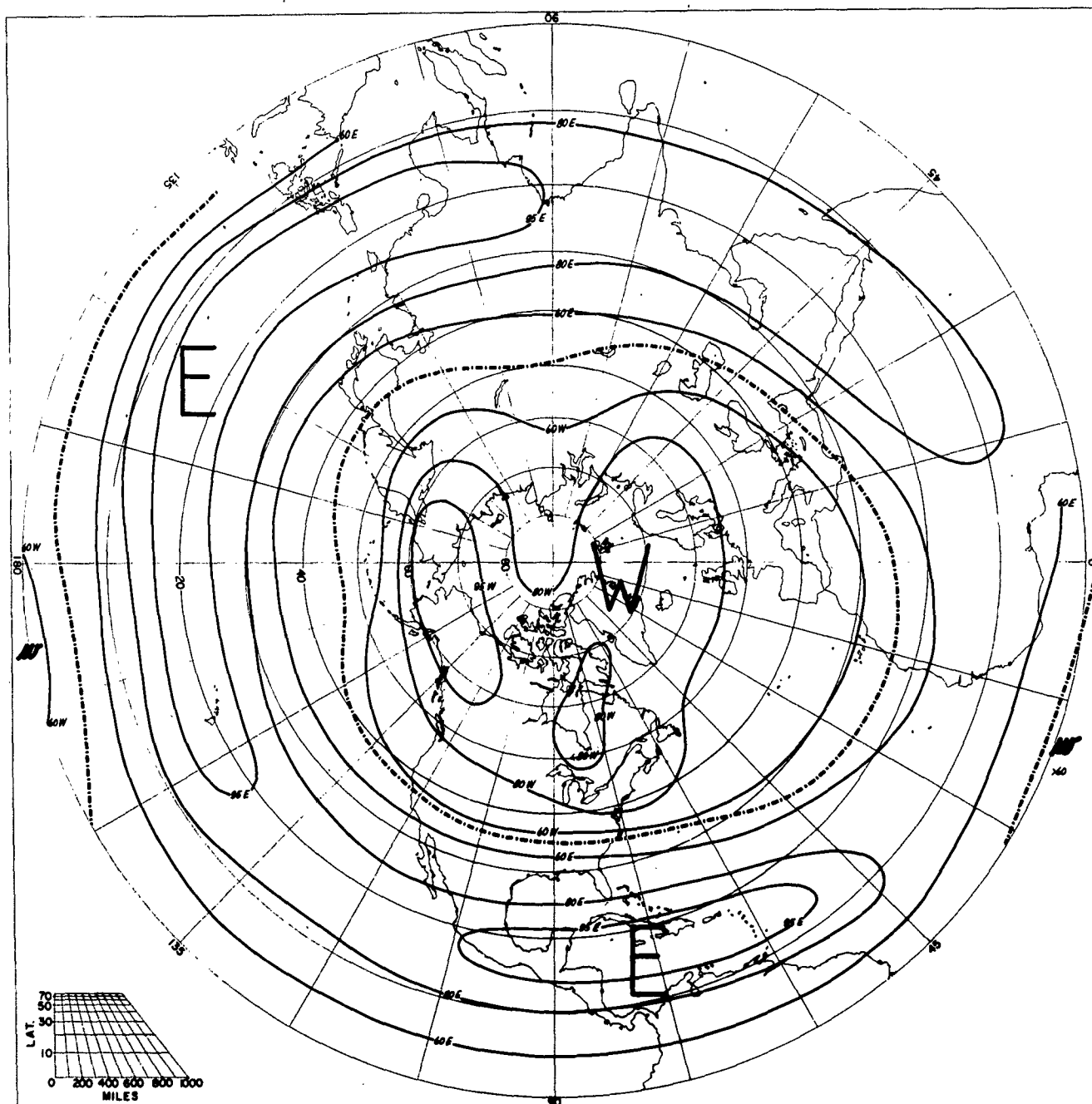
FREQUENCY OF PREVAILING ZONAL WINDS OCTOBER 30 1948
