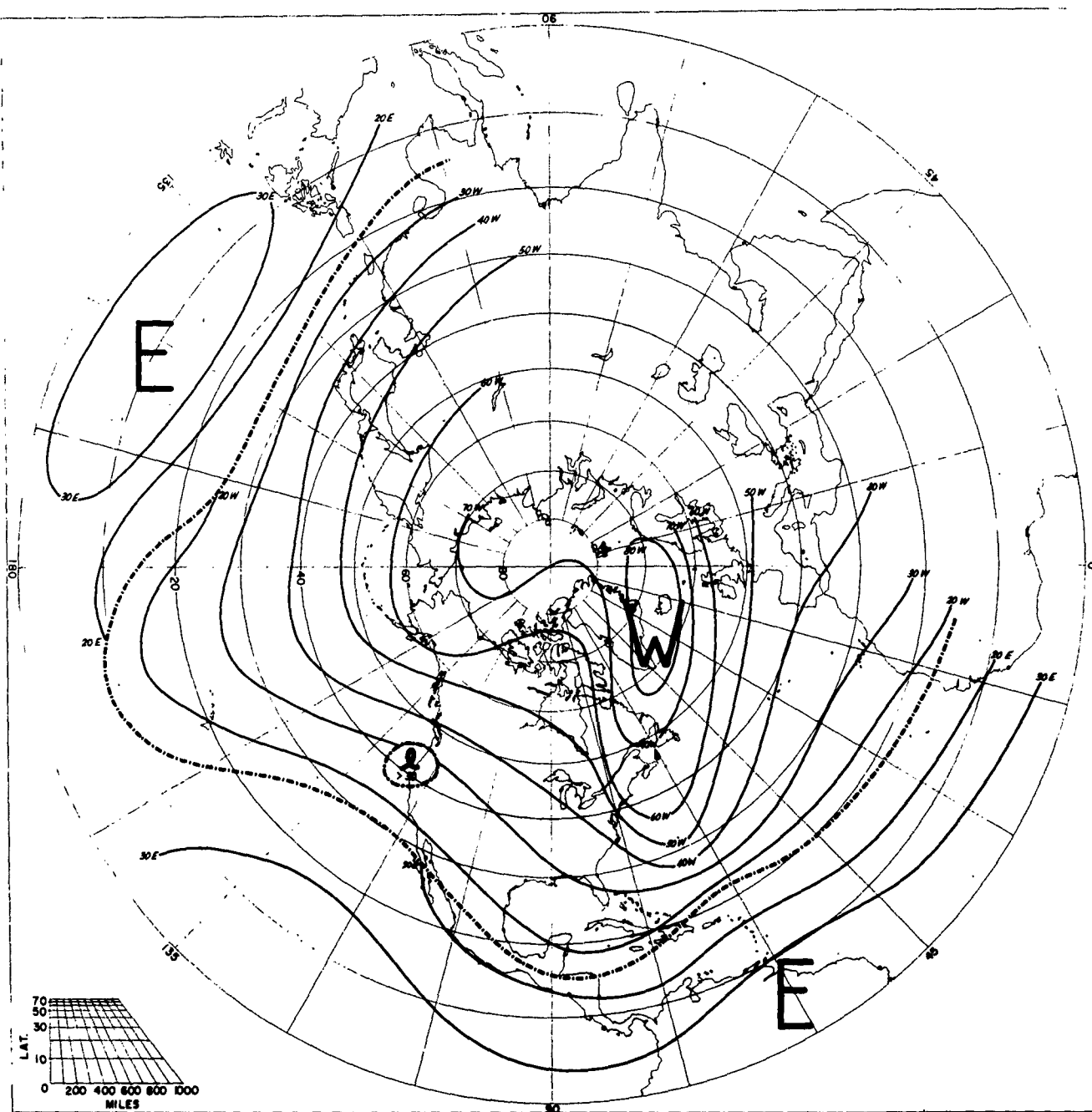
SPEED OF PREVAILING ZONAL WINDS DECEMBER 10 MB
