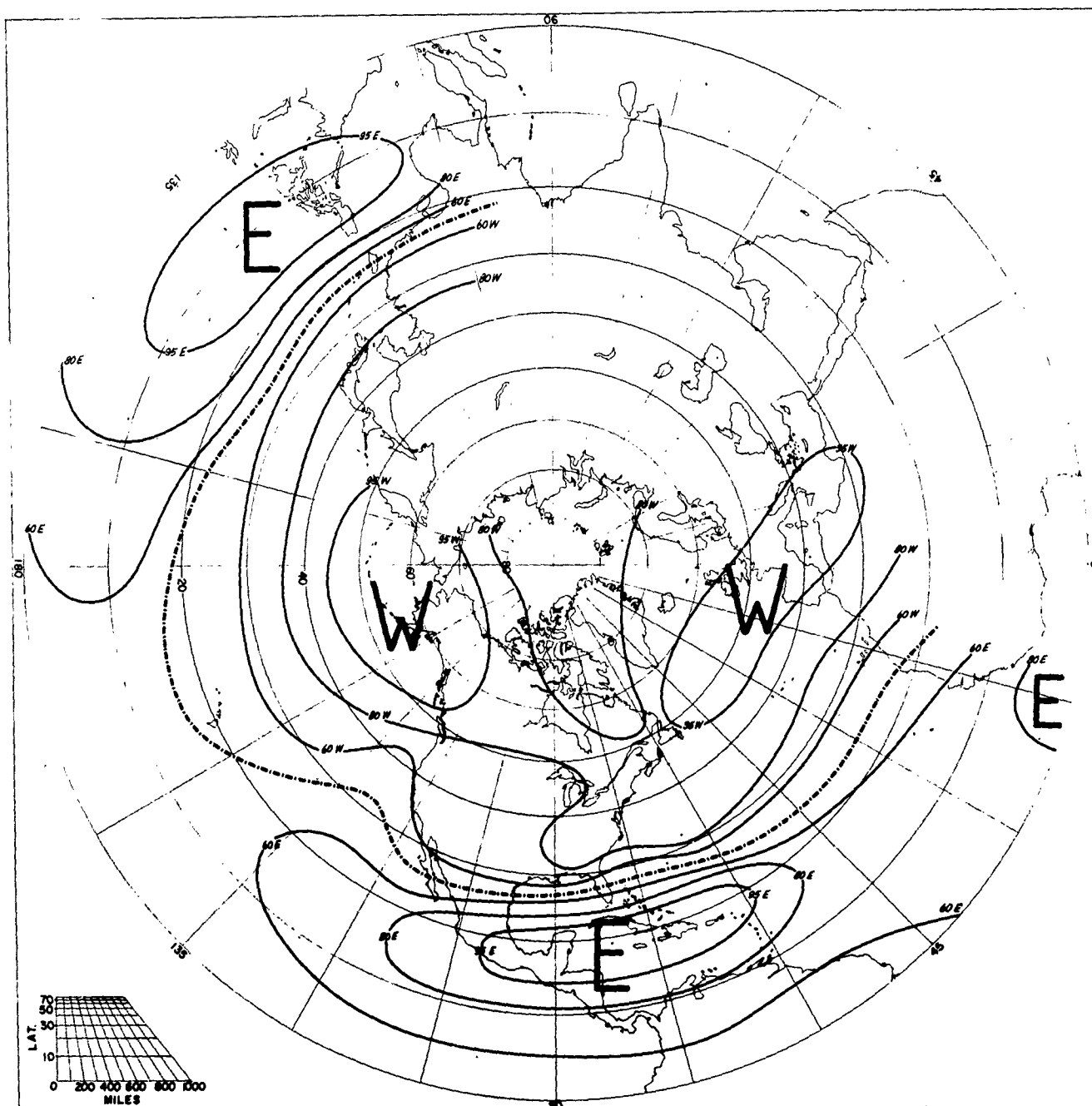
FREQUENCY OF PREVAILING ZONAL WINDS NOVEMBER 10 MB
