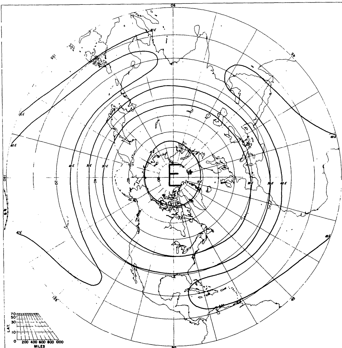
SPEED OF PREVAILING ZONAL WINDS JULY 30 MB
