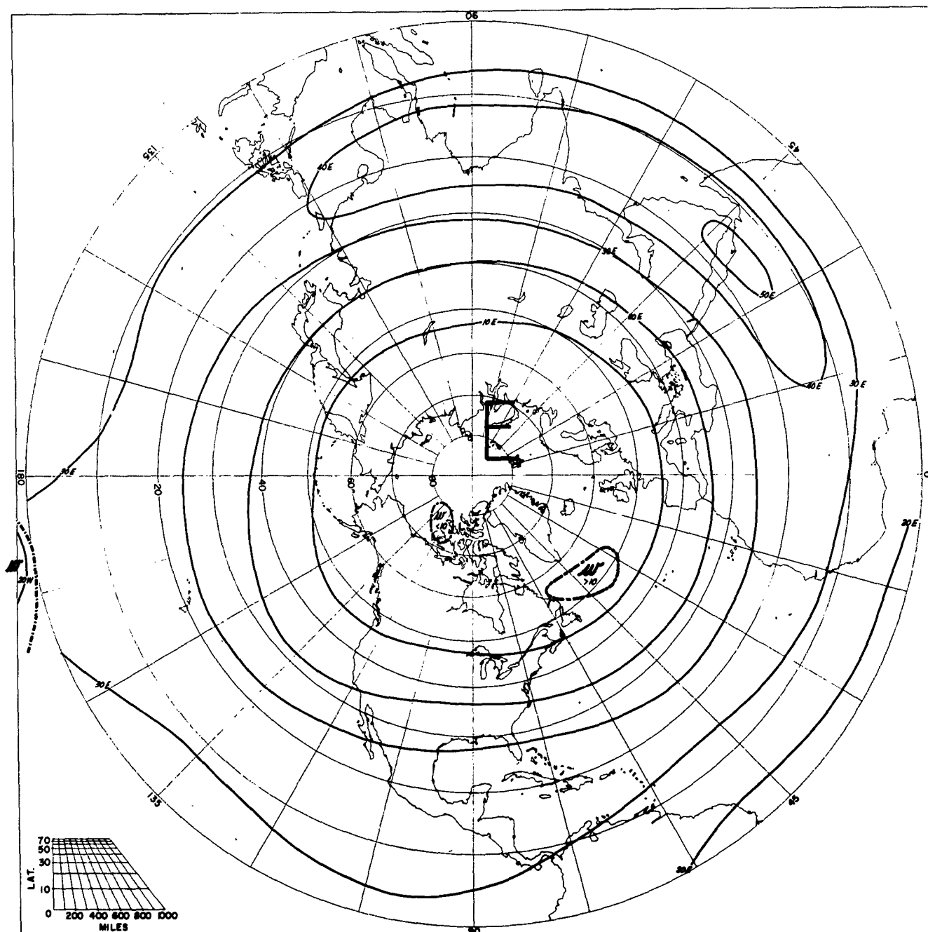
SPEED OF PREVAILING ZONAL WINDS JULY 50 MB
