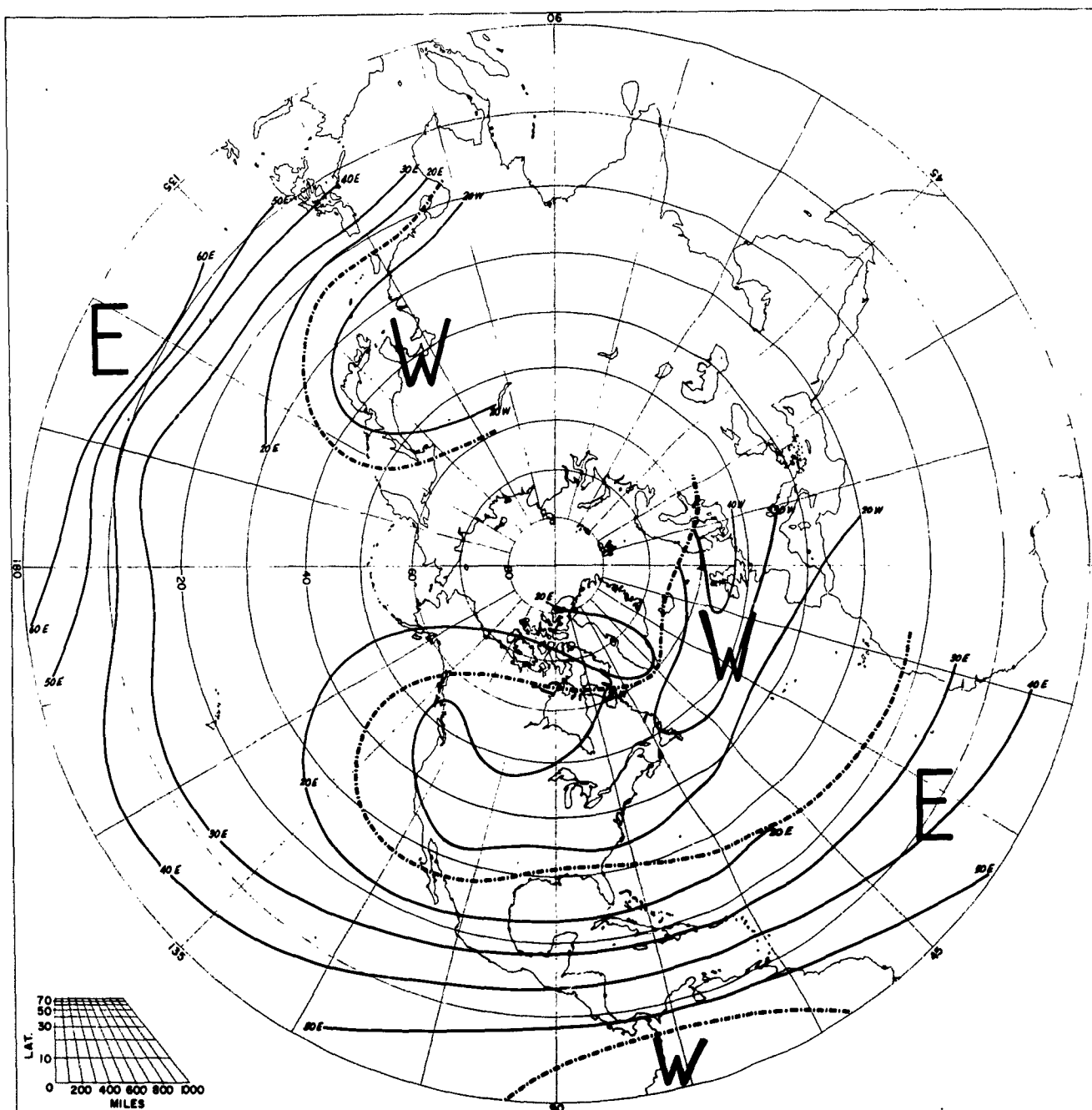
SPEED OF PREVAILING ZONAL WINDS APRIL 10 MB
