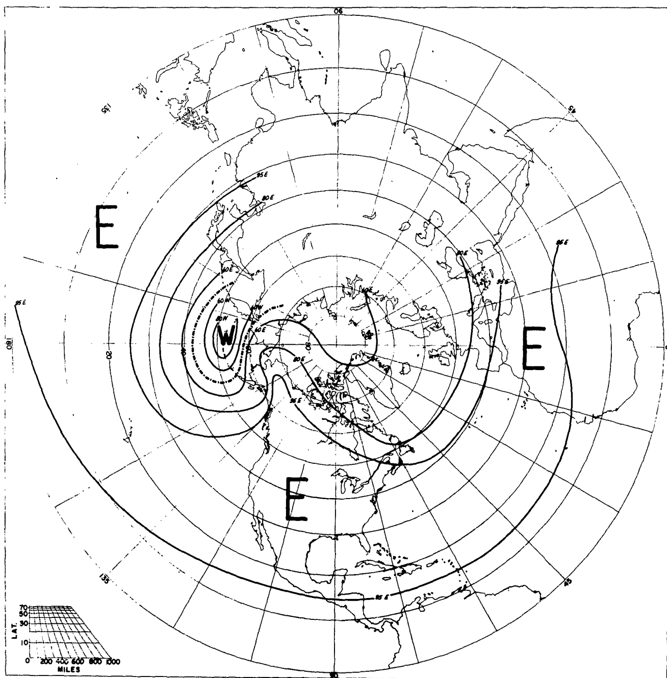
FREQUENCY OF PREVAILING ZONAL WINDS AUGUST 10 MB
