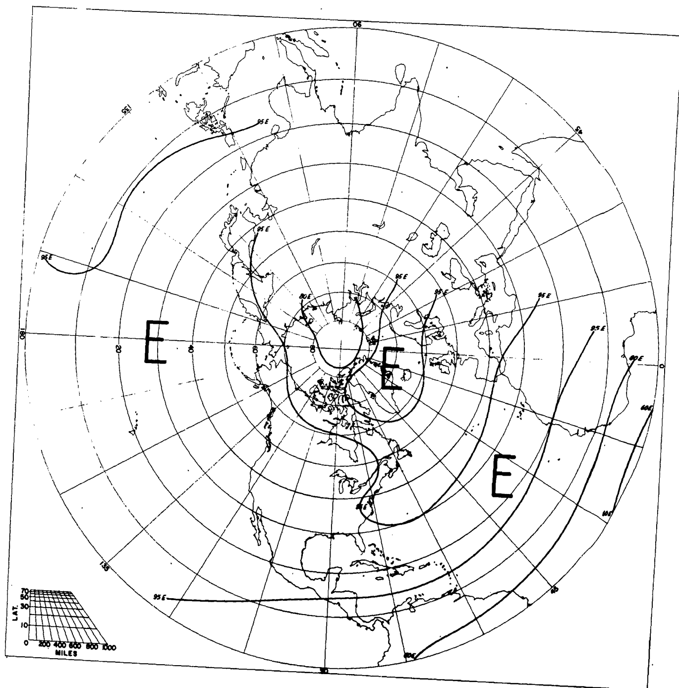
FREQUENCY OF PREVAILING ZONAL WINDS JUNE 10 MB
