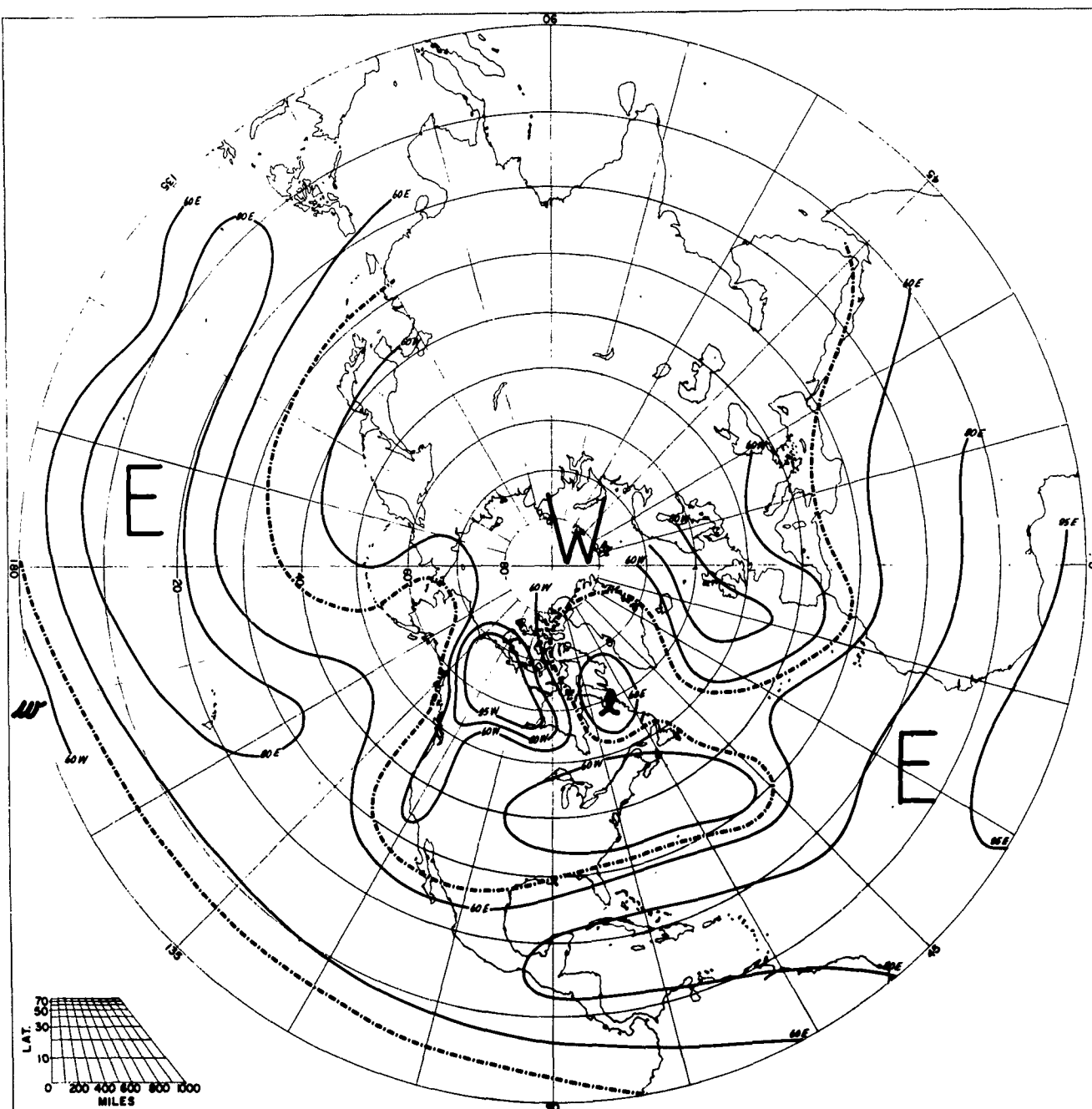
FREQUENCY OF PREVAILING ZONAL WINDS APRIL 30 MB
