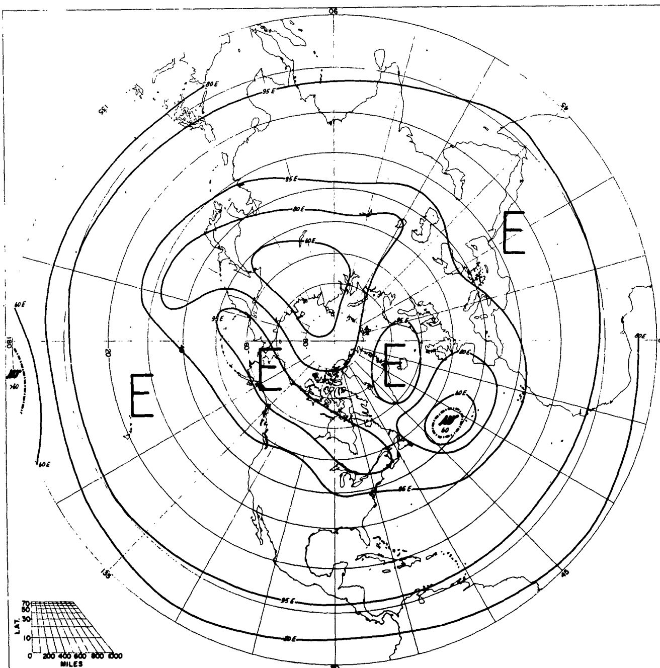
FREQUENCY OF PREVAILING ZONAL WINDS JUNE 30 MB
