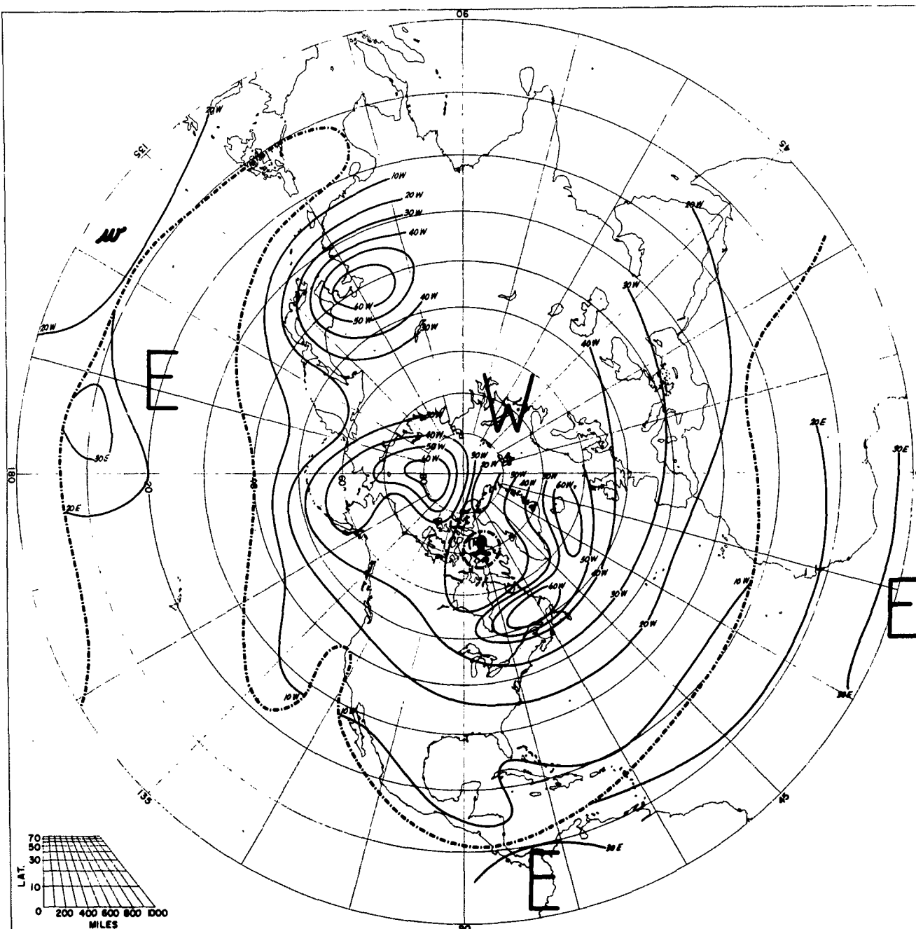
SPEED OF PREVAILING ZONAL WINDS JANUARY 30 MB
