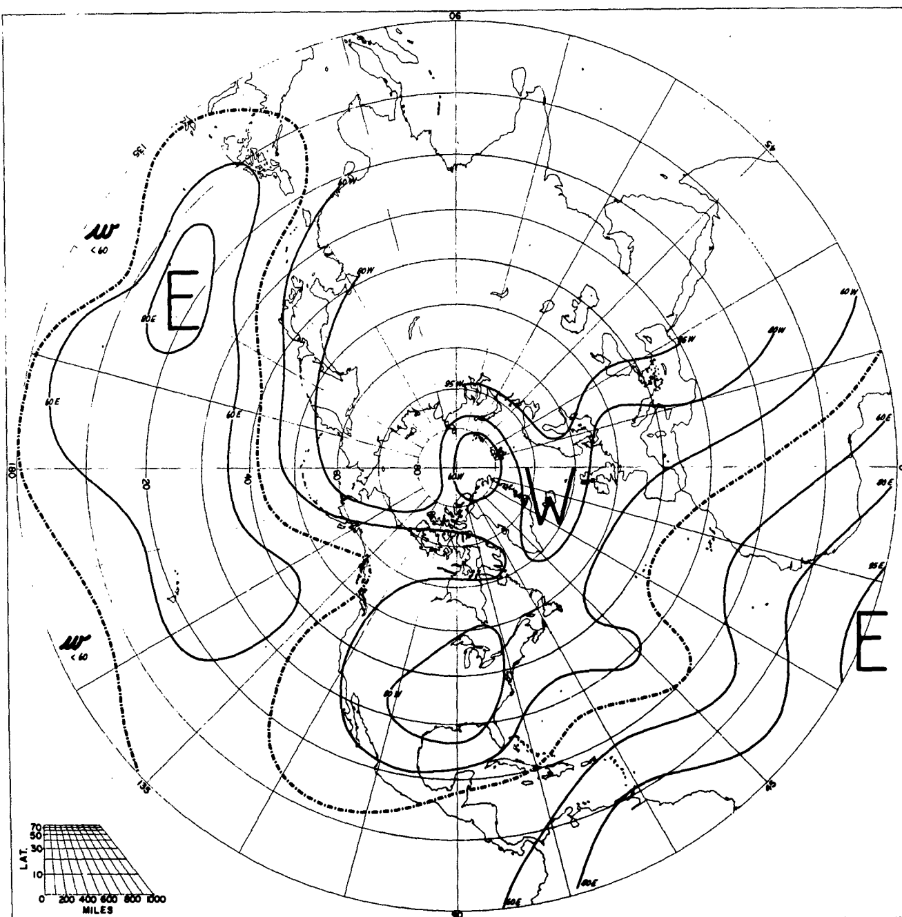
FREQUENCY OF PREVAILING ZONAL WINDS MARCH 30 MB
