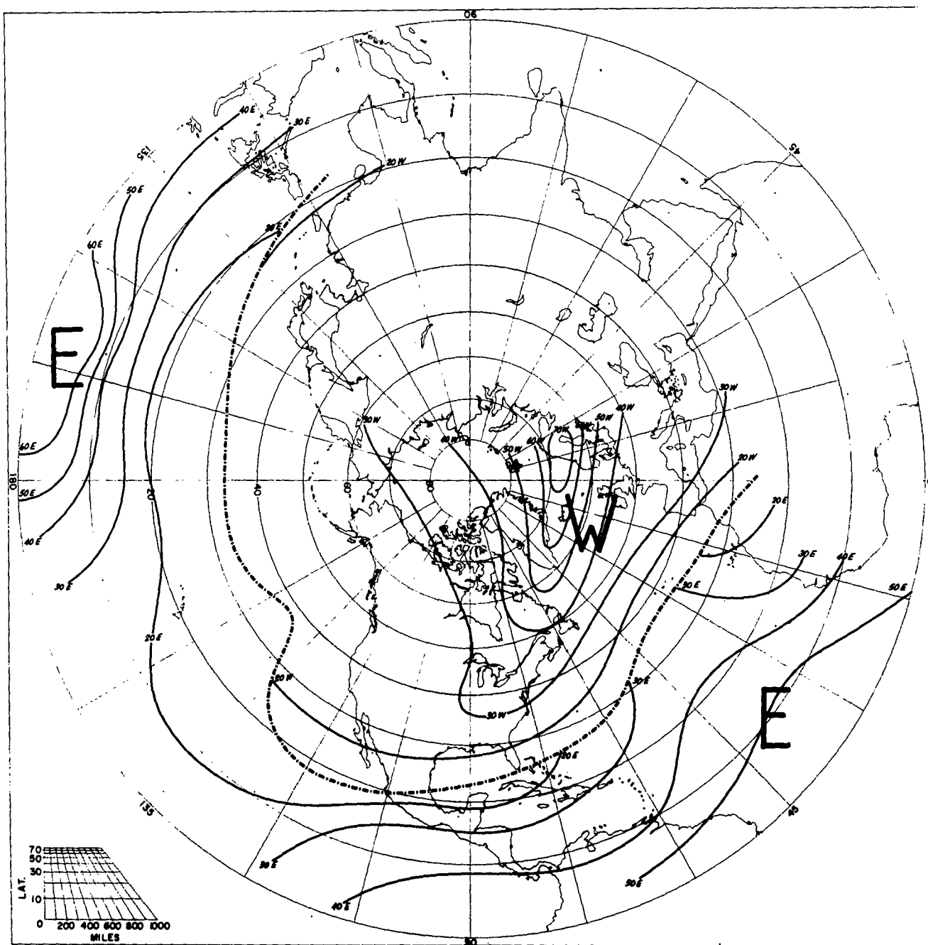
SPEED OF PREVAILING ZONAL WINDS MARCH 10 MB
