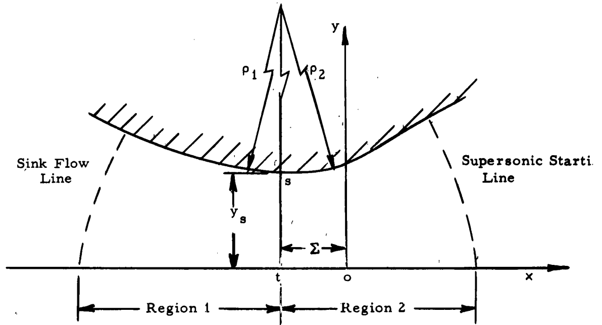
Figure 2. Constant-Lag Transonic Flow Model
