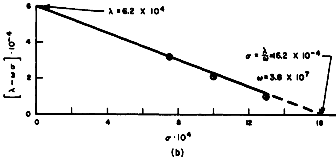
Figure 7. Strength-time-temperature behavior of aluminum (References 22 and 24) (a) Dependence of time to fracture on the absolute temperature (b) Dependence of \lambda - \omega \sigma on \sigma .
