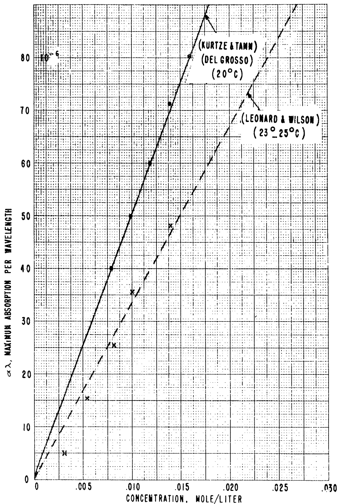
FIGURE 2. DEPENDENCE OF ABSORPTION ON CONCENTRATION OF \text{MgSO}_4 SOLUTIONS
