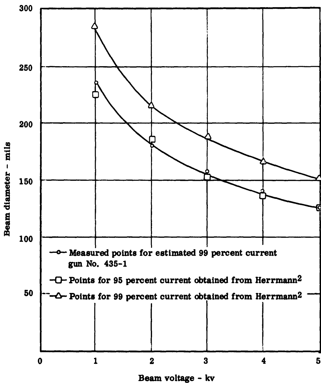
Fig. 4 - Beam diameter as a function of beam voltage for gun 435-1. The agreement between calculated and measured diameters is good. The 99 percent current points were only estimated from the measured beam profiles.
