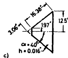
FIG. 2 DIMENSIONS OF TYPICAL CONICAL SHELLS
