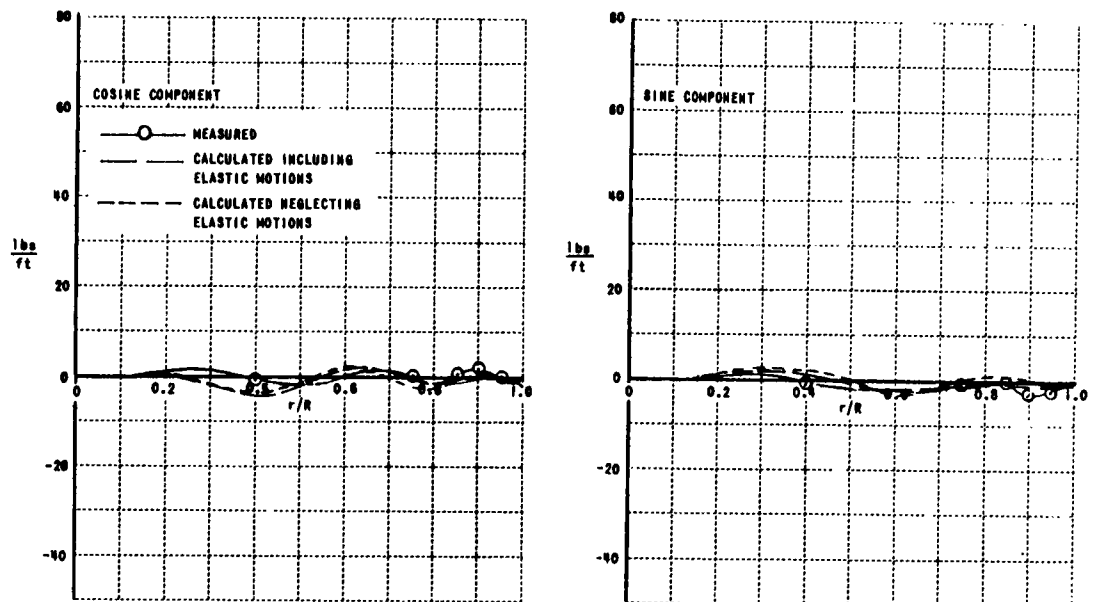
Figure 6j. 9th HARMONIC AIRLOADS; HU-1A; \mu = 0.26
