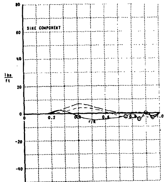
Figure 6g. 6th HARMONIC AIRLOADS; HU-1A; \mu = 0.26
