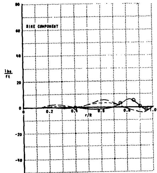
Figure 6h. 7th HARMONIC AIRLOADS; HU-1A; \mu = 0.26
