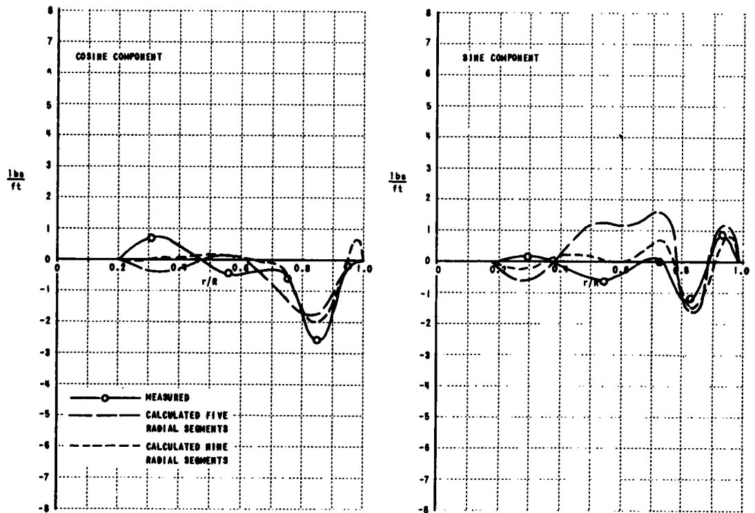
Figure 4j. 9th HARMONIC AIRLOADS; NASA MODEL; \mu = 0.15
