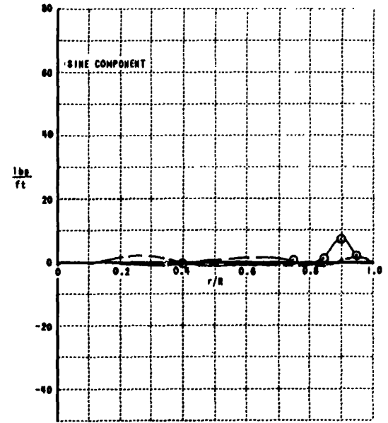
Figure 6l. 11th HARMONIC AIRLOADS; HU-1A; \mu = 0.26
