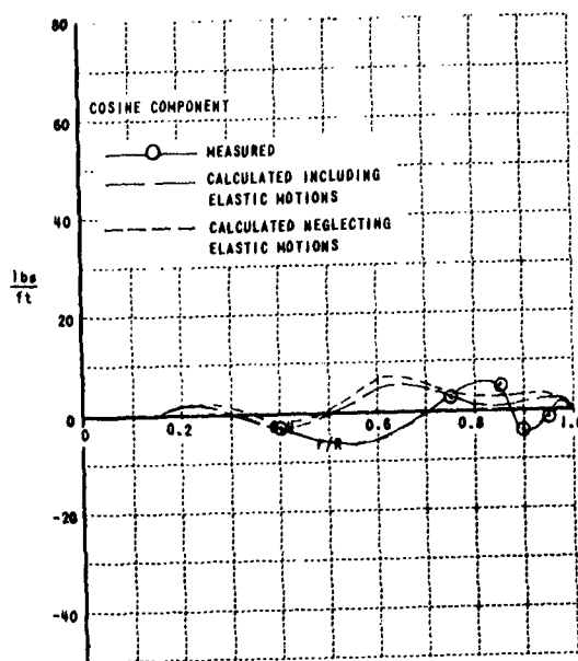
Figure 6g. 6th HARMONIC AIRLOADS; HU-1A; \mu = 0.26
