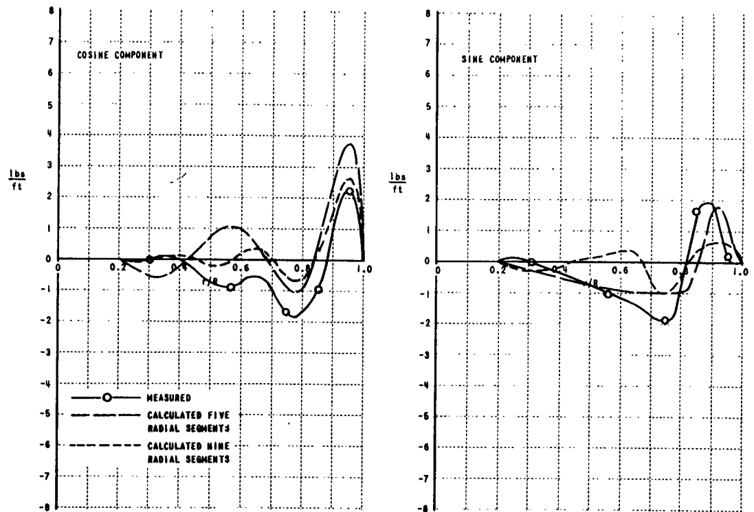
Figure 4i. 8th HARMONIC AIRLOADS; NASA MODEL; \mu = 0.15
