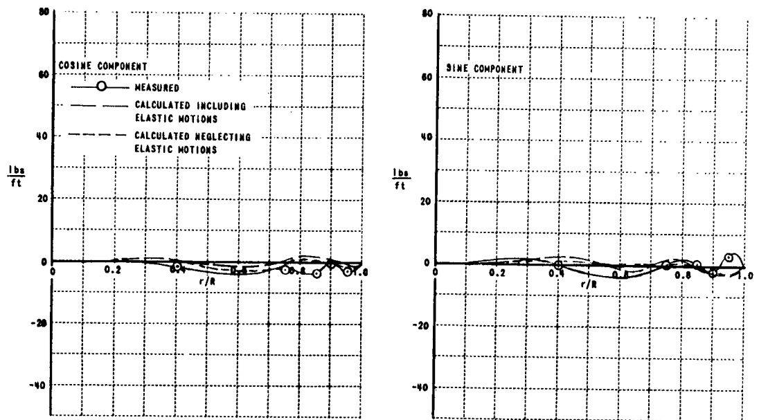
Figure 6i. 8th HARMONIC AIRLOADS; HU-1A; \mu = 0.26
