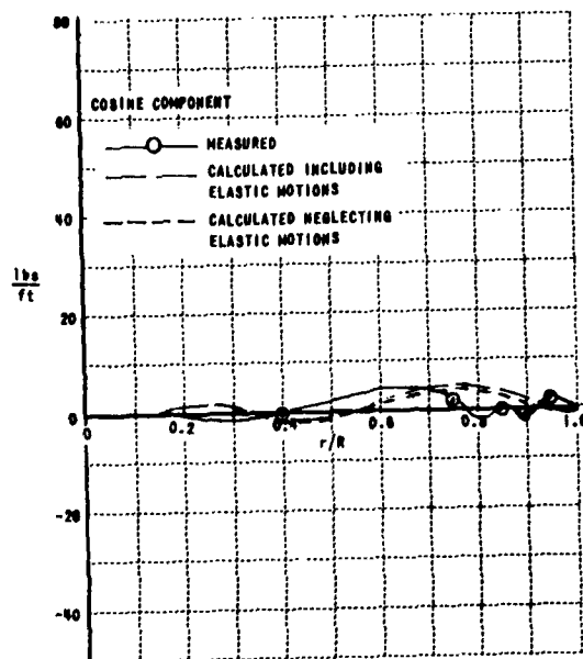
Figure 6h. 7th HARMONIC AIRLOADS; HU-1A; \mu = 0.26
