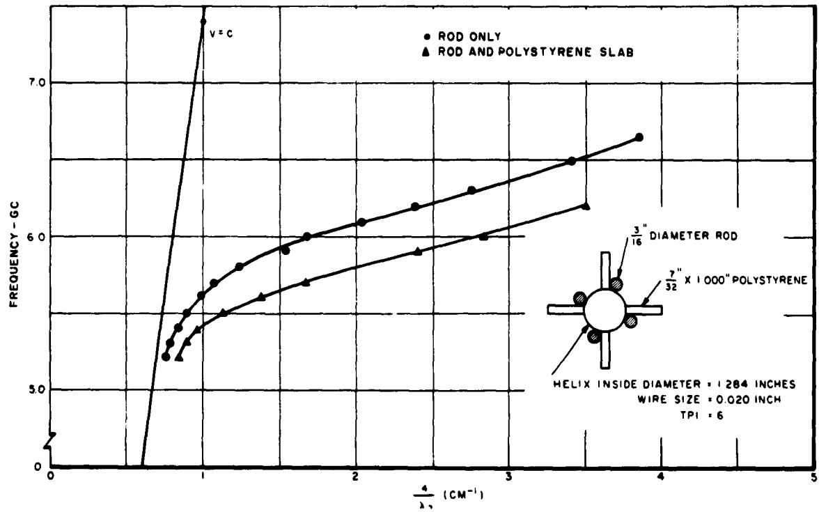
FIGURE 33. \omega - \beta CHARACTERISTICS OF A QUADRIFILAR HELIX
