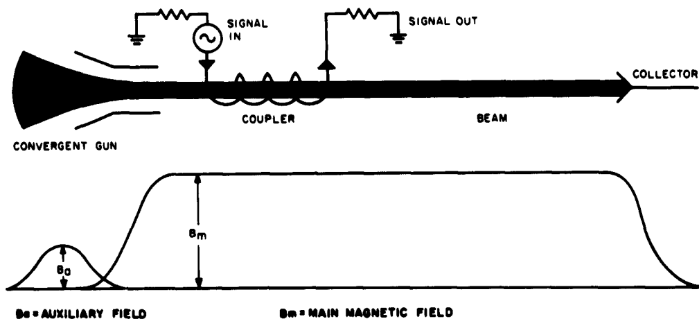
FIGURE 16. KUMPFNER DIP EXPERIMENTAL MEASUREMENT
