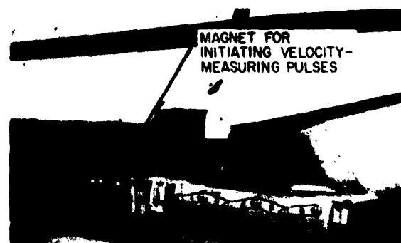
FIG. 13. Double-Hung Slipper Installation With Magnet Mounting.
