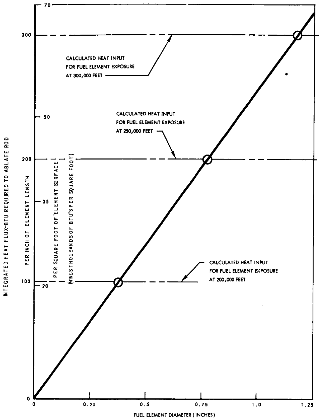
Figure 24. Heat Input Required for Fuel Element Heating and Ablation Versus Diameter
