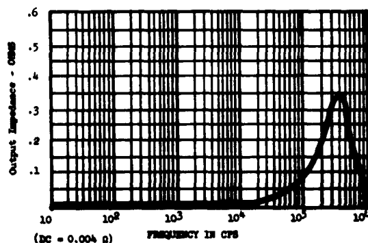
Fig. 1 Output Impedance vs Frequency ZA-724
