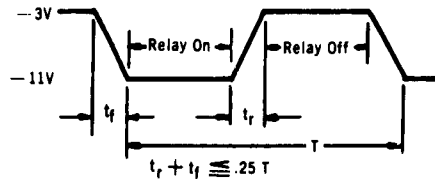
INPUT WAVEFORM
