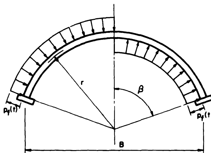
(a) Uniform Compression Loading. ( See Fig. 5-6 For Variation With Time.)
