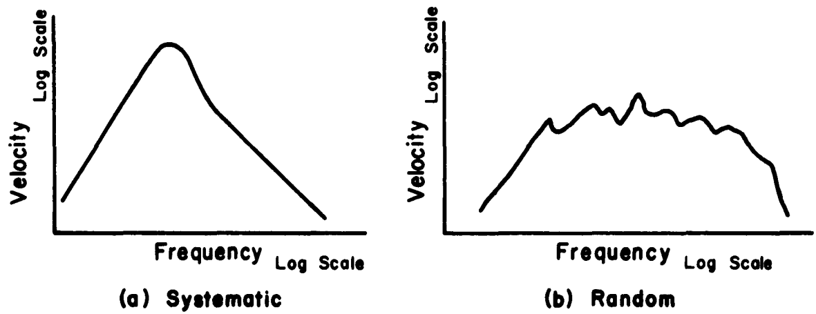
FIG. 10-3 RESPONSE SPECTRA
