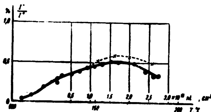
Fig. 30. Coefficient of conversion H_1^+ \rightarrow H_1^- as a function of thickness of vapor-jet target for protons with 30-kev energy.
