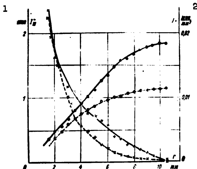
Fig. 38. I_{\text{III}} and f as function of focusing position in transformation H_1^+ \rightarrow H_1^- : (●●●) I ; (xxx) f ; (—) E_{H_1^+} = 22.4 kev; (---) E_{H_2^+} = 32.4 kev. 1) \mu\text{a} ; 2) \mu\text{a}/\text{mm}^2 .
