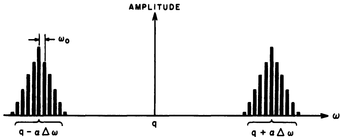
FIG. 10 SPECTRUM OF A SQUARE WAVE OF FREQUENCY \omega_0 AFTER FREQUENCY MODULATION WITH CARRIER FREQUENCY q
