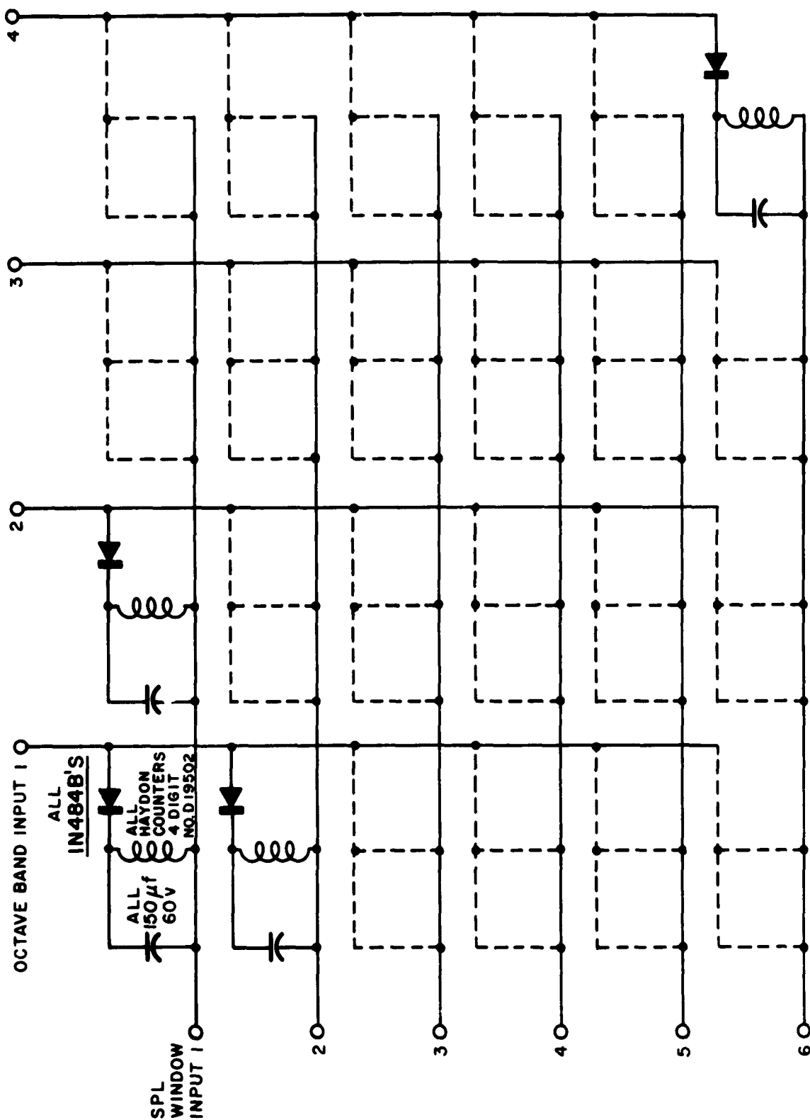
FIG. A-II COUNTER MATRIX
