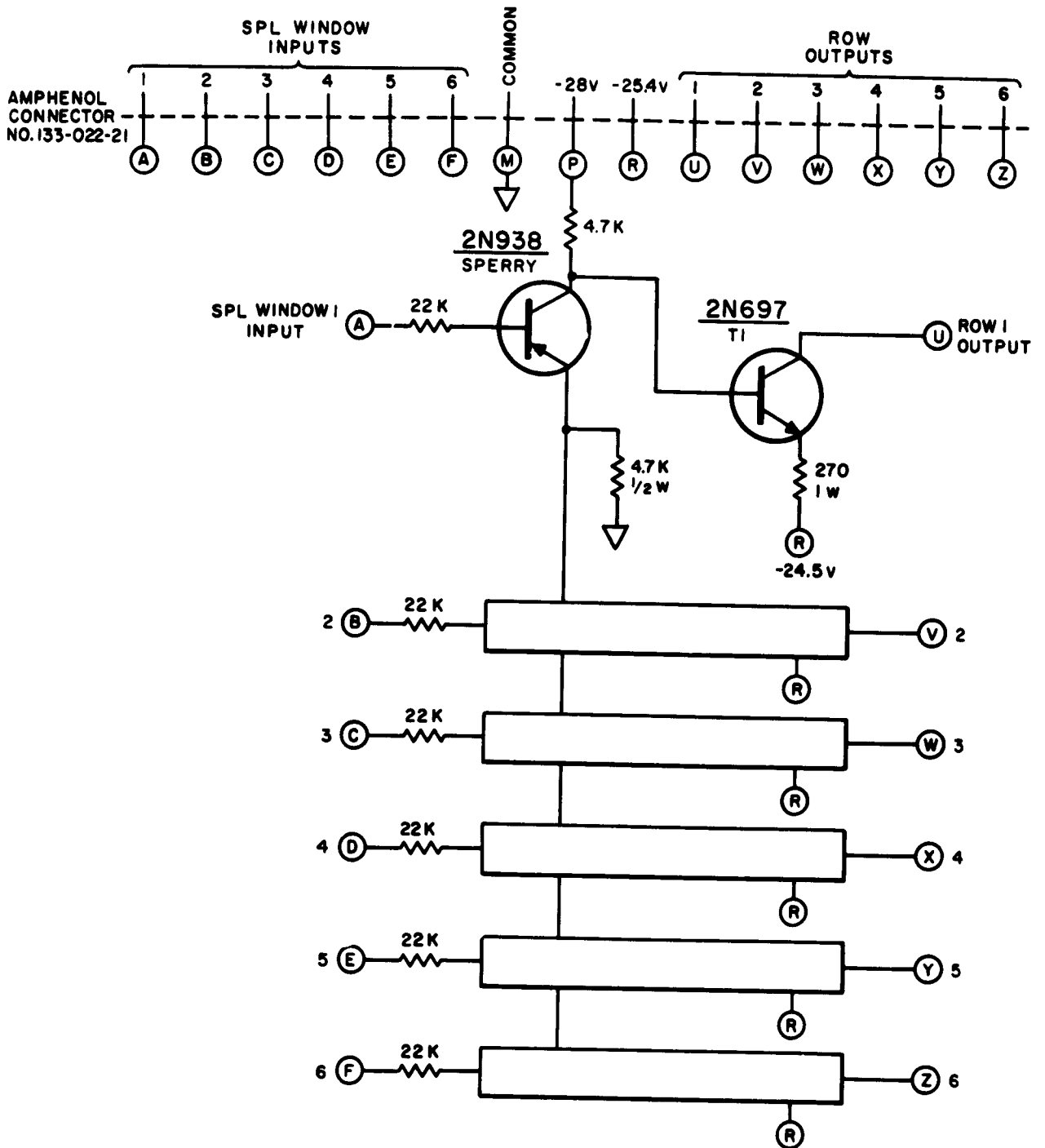
FIG. A-9 COUNTER ROW DRIVERS
