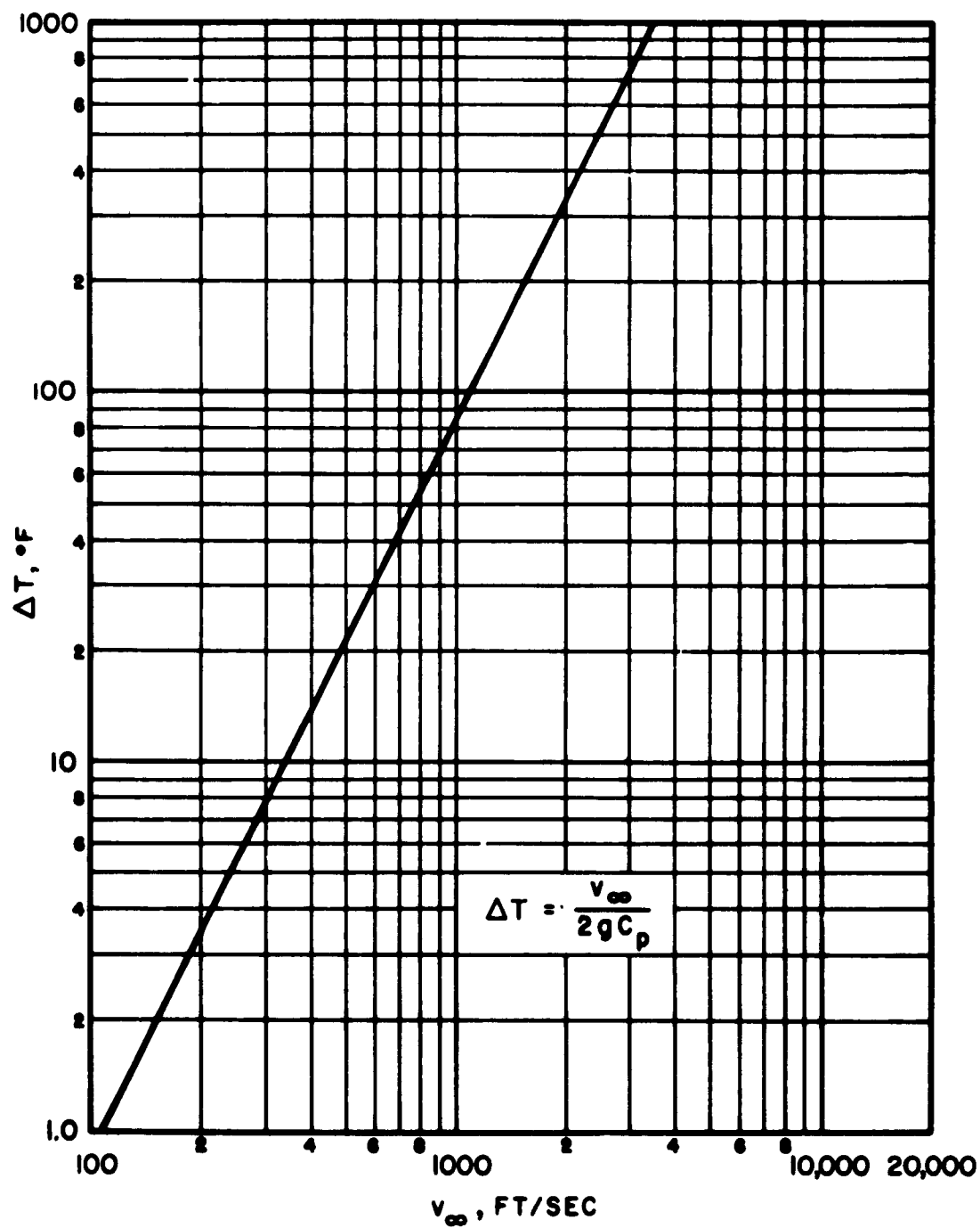
FIG. 8 TEMPERATURE RISE FOR ADIABATIC DECELERATION OF FLOW
