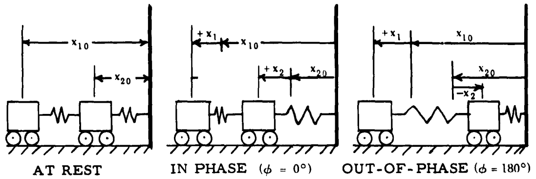
Figure 87a - Two-Mass, Two-Degree-of-Freedom System
