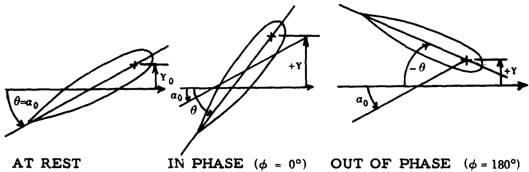
Figure 87b - Hydrofoil of TMB Control Surface Flutter Apparatus
