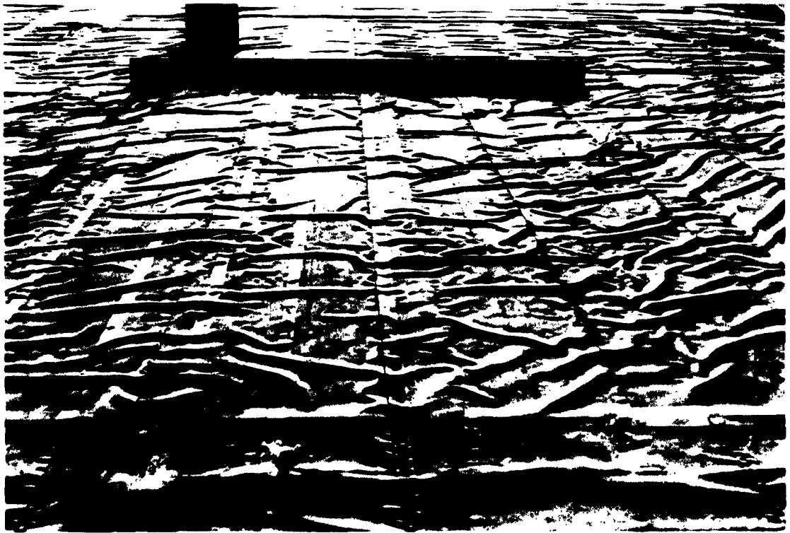
Photograph 19. Section 5, lane 1, prior to start of traffic tests
