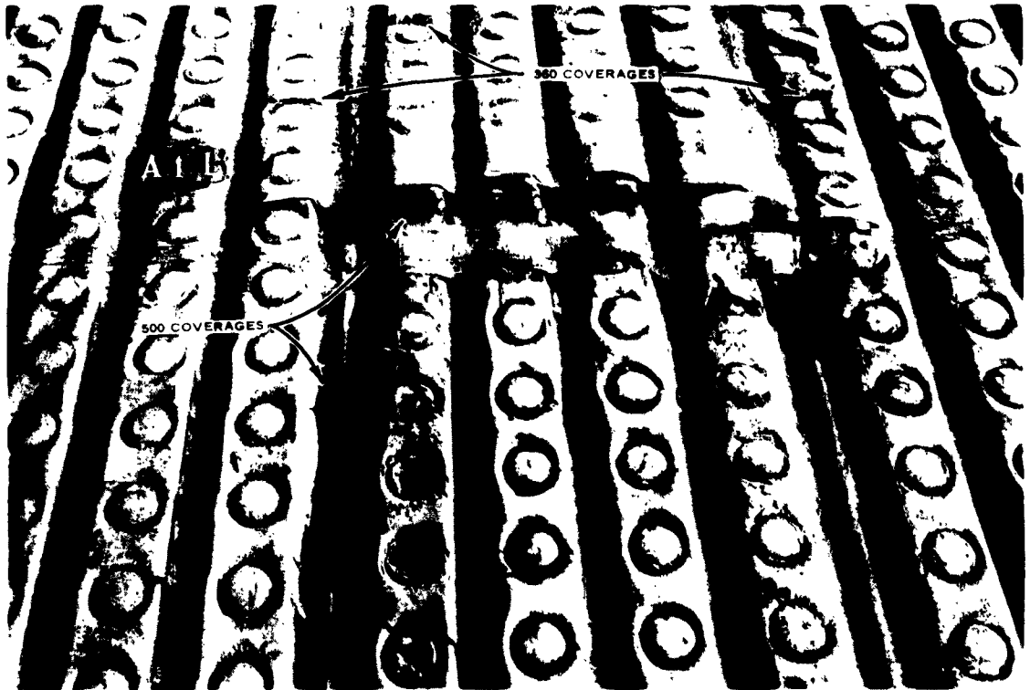
Photograph 24. Section A, lane 2. Note failures of T1 cotton duck membrane caused by tubular holes (360 coverages) and end of mat panel (500 coverages)
