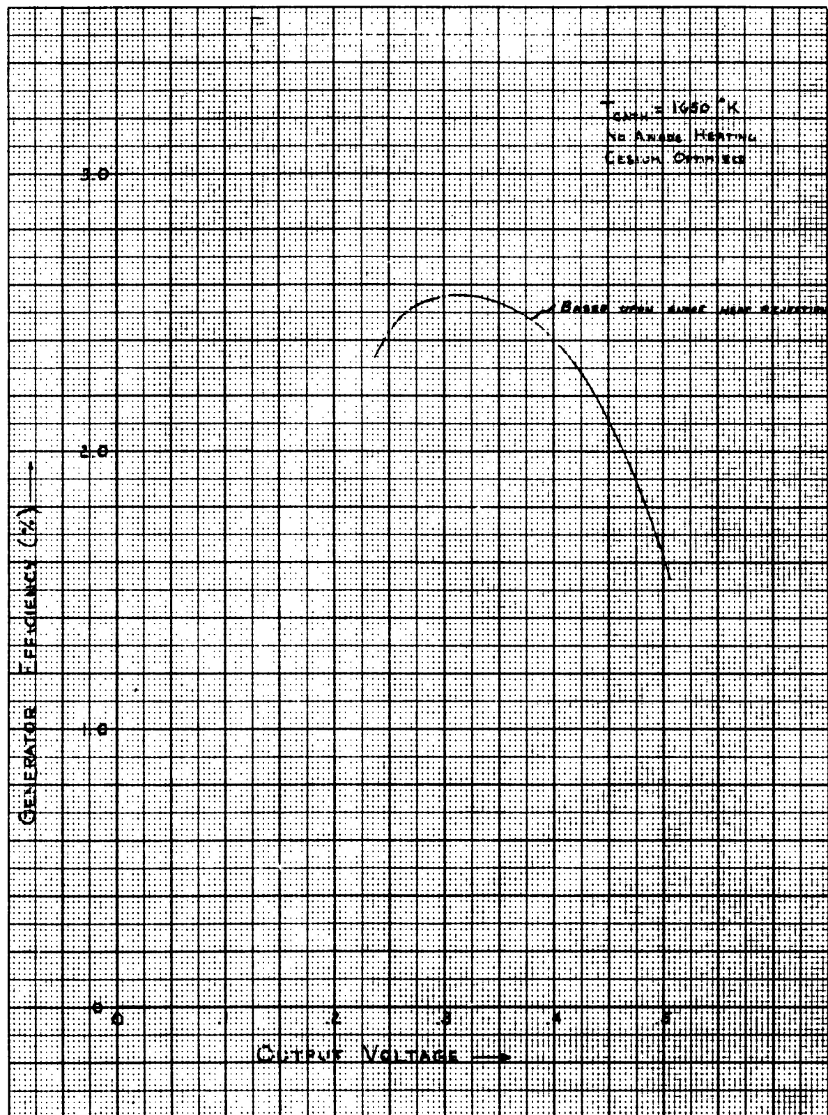
Figure 85. Predicted Efficiency with 43, 46, and 47 In Parallel
