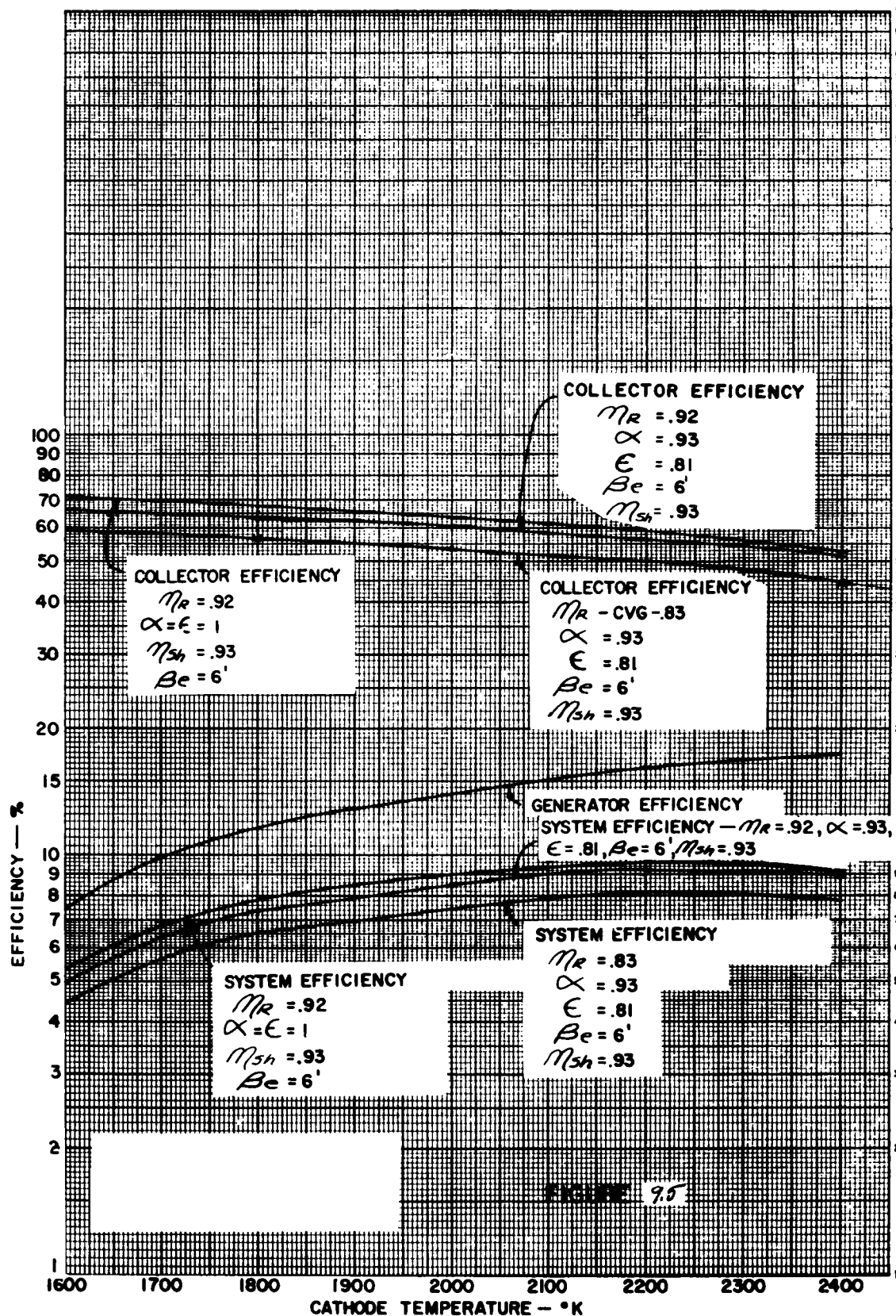
Figure 95. System Efficiencies vs. Cathode Temperature
