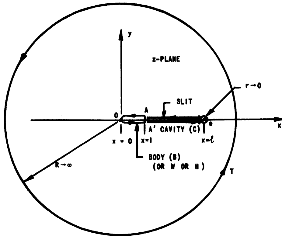
FIGURE 6. CONTOUR PATHS FOR COMPLEX INTEGRATION.
