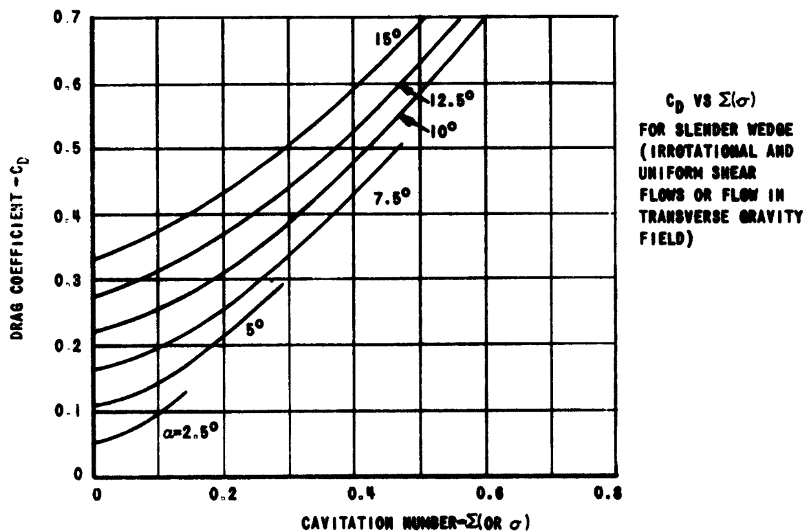
FIGURE 7. DRAG COEFFICIENT VS CAVITATION NUMBER FOR FLOW PAST A UNIT WEDGE.
