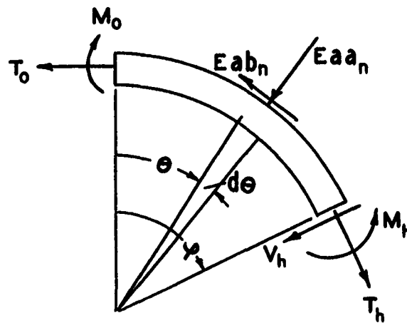
FIG. 2 FREE BODY DIAGRAM OF A SEGMENT OF THE RING, 0 \leq \varphi \leq \varphi_f
