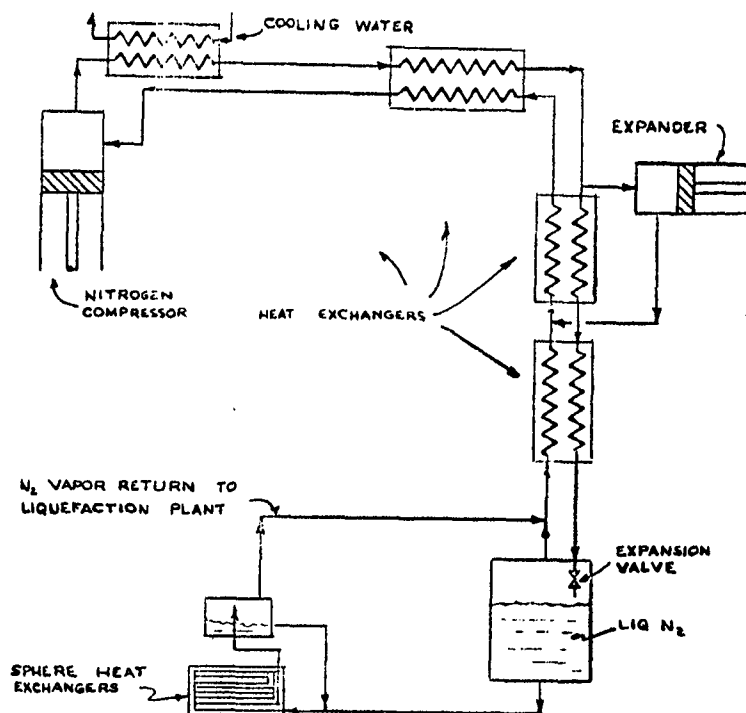
Figure IVC-1\ Claude Cycle
