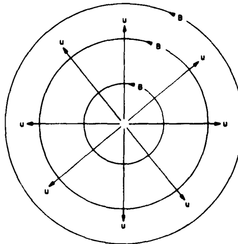
Figure 13-1. Source Flow Model of Crossed Field Accelerator
