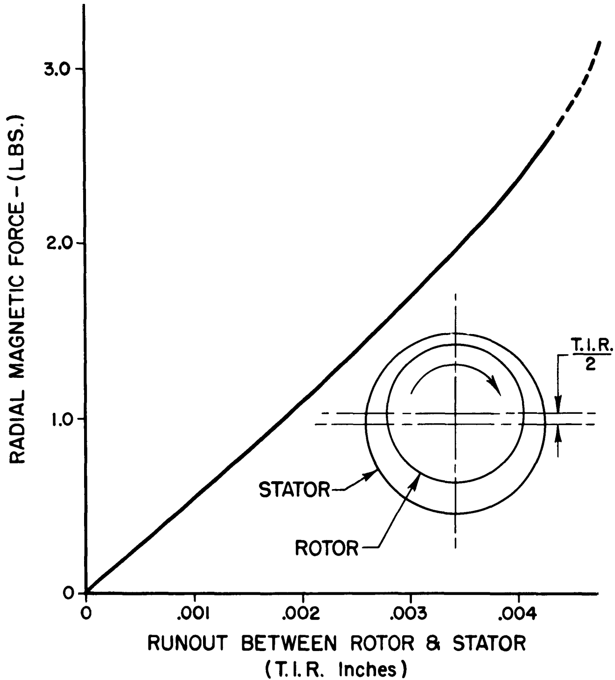
Fig. 6—Induction Motor Magnetic Force
