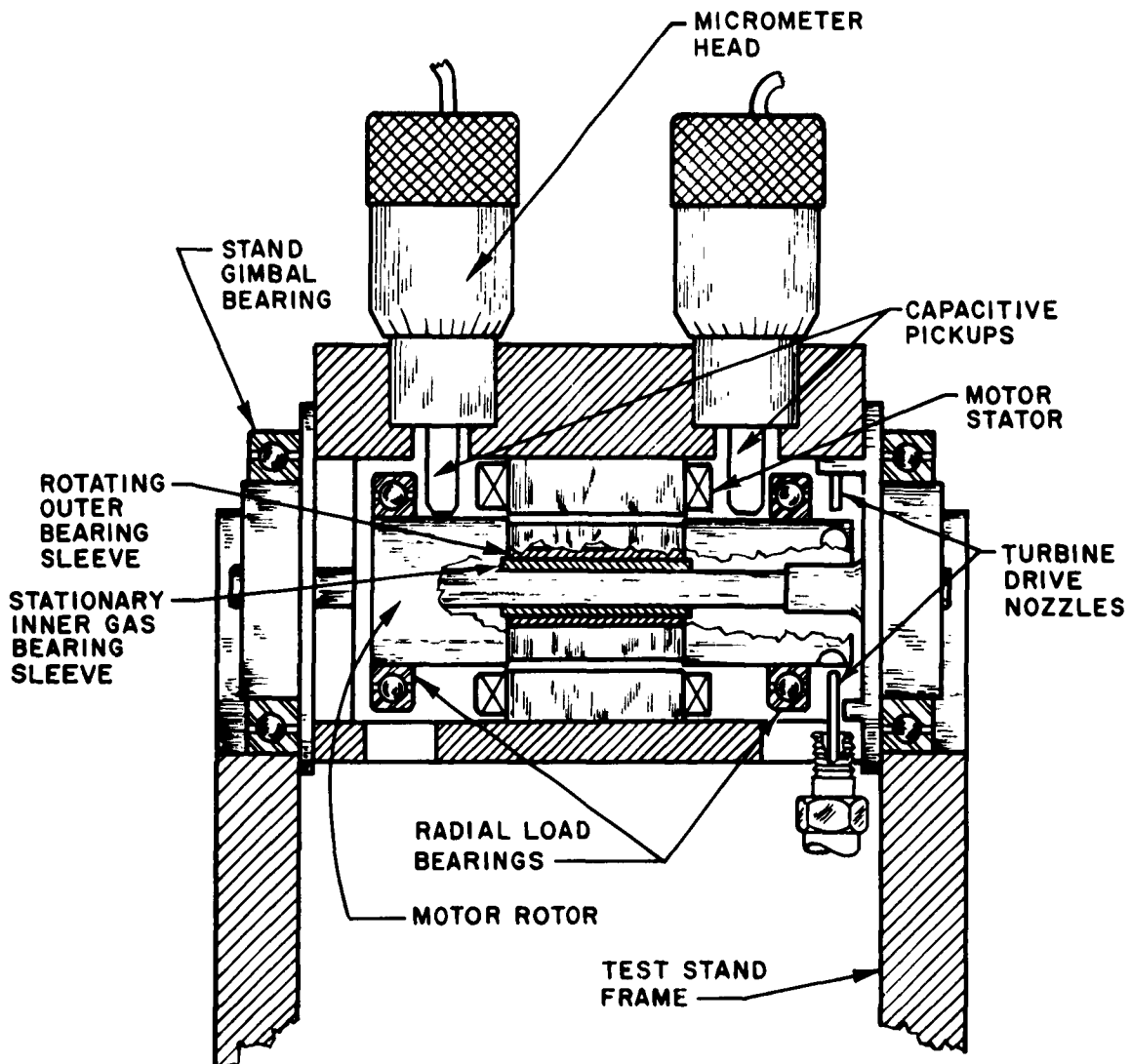
Fig. 1—Schematic of Gas Bearing Test Rig
