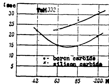
Fig. 8. Influence of abrasive mesh on machining time.
