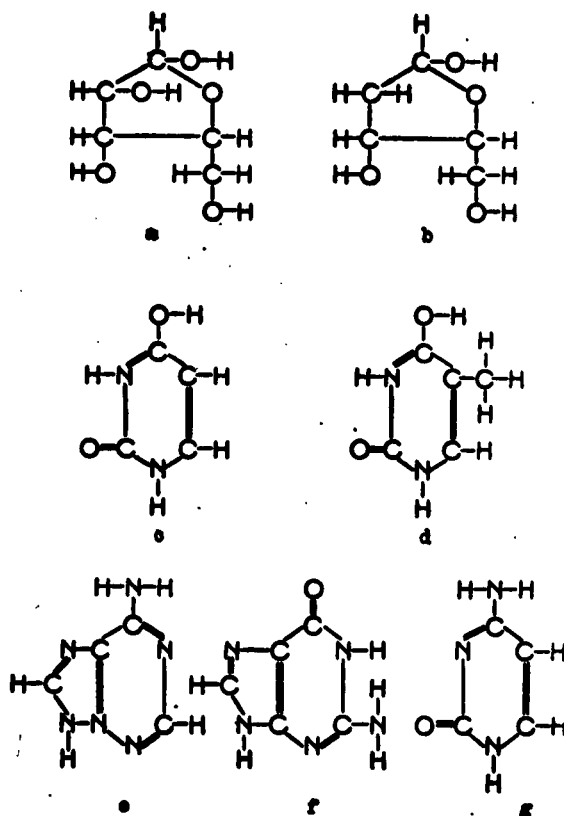
Fig. 6. Chemical structure of carbohydrates and nitrogenous bases participating in ribonucleic* and deoxyribonucleic acids: a) d-ribose; b) d-2-deoxyribose; c) uracil; d) thymine; e) adenine; f) guanine; g) cytosine.
