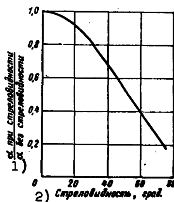
Fig. 1.9. Influence of the sweepback of the wing on the heat transfer at the critical point of the leading edge. 1) ( \alpha with sweepback)/( \alpha without sweepback); 2) sweepback, deg.
