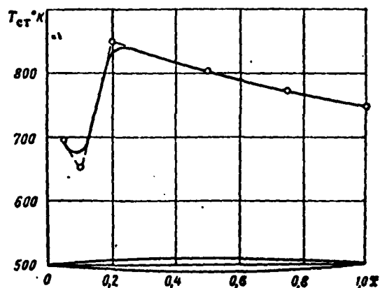
Fig. 3.1. Temperature distribution along the chord on the lower surface of the wing profile. M_\infty = 5 ; H = 30 km; \alpha = 10^\circ ; s = 0.8 .
