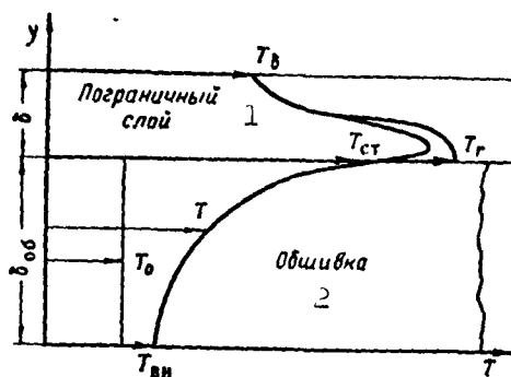
Fig. 4.2. Diagram of temperature distribution along the thickness of the boundary plating. 1) Boundary layer; 2) plating.
