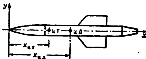
Fig. 6.49. Missile with tail surfaces shifted forward
