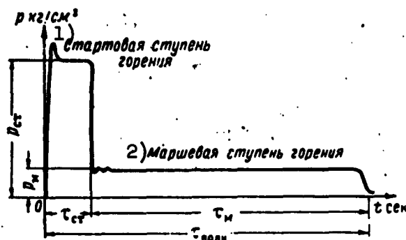
Fig. 5.35. Burning curve with two thrust stages providing for maximum speed for entry of missile into the controlled-flight phase. p_{st} and p_m ) pressure in combustion chamber during launch and cruising regimes, respectively; \tau_{st} and \tau_m ) engine operating time during launch and cruising regimes, respectively; \tau_{полн} ) total engine operating time; 1) starting stage of burning; 2) cruising stage of burning.
