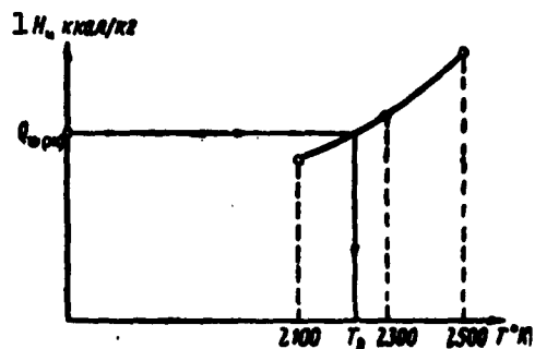
Fig. 4.2. Graph for the determination of true temperature of the products of powder combustion. H_1 is the heat content (enthalpy) of the powder; 1) H_1 , kcal/kg.
