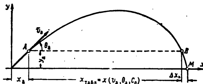
Fig. 6.45. Calculation diagram for trajectory to determine trajectory elements through utilization of ballistic tables. x_a, y_a ) coordinates of the end of the active trajectory phase; v_a ) velocity at the end of the active trajectory phase; \theta_a ) the angle of inclination of the tangent to the trajectory at the end of the active phase.
