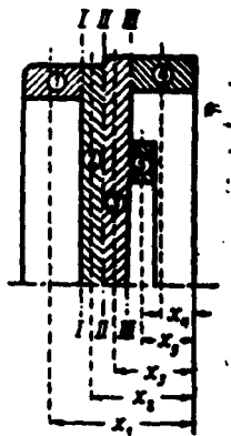
Fig. 6.17. Determination of position of center of gravity for a complex figure. 1-5) elements of figure; x_1 ) coordinate of the center of gravity of the i -th component of the figure.
