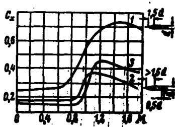
Fig. 6.37. Laws governing resistance of standard missiles 1) The Siachchi law; 2) The law of the year "1930"; 3) The law of the year "1943."
