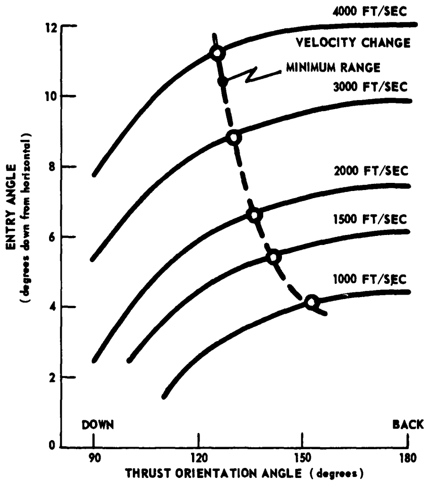
Fig. 5 ATMOSPHERIC ENTRY ANGLE VERSUS MAGNITUDE AND DIRECTION OF VELOCITY CHANGE FOR 300 N. MILE CIRCULAR ORBIT (ENTRY AT 400,000 FEET ALTITUDE)
