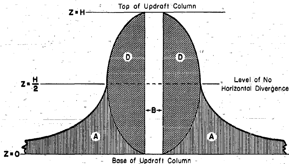
Fig. 3. Schematic illustration of Cases 3 and 4, discussed in the text and listed in Tables 3a, b and 4a, b. Horizontal divergence in the high atmosphere accompanies rising air motion and spreads precipitation packets horizontally as they descend in the shaded area marked D. The packets are contracted again by horizontal convergence in the lower atmosphere. Precipitation at the ground in the section marked B is due to condensation in a volume larger by the extent of horizontal shading than the unshaded cross section vertically overhead. When condensate augments precipitation at the level of nondivergence but not below that height, the region contributing to precipitation at B is further increased by the area of vertical shading marked A in the figure. Cloud in area A is swept inward and upward by horizontal convergence and ascends to the level of nondivergence, where it is collected by precipitation and ultimately deposited at the ground in Section B.
