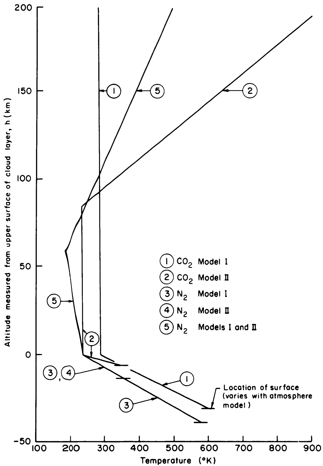
Fig. I—Temperature distribution of models of the Venus atmosphere
