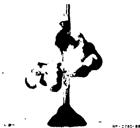
FIG. 2 PHOTOGRAPH OF W SPECIMEN AFTER RUN A
