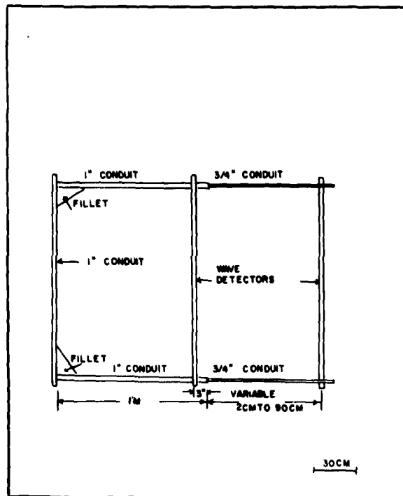
Fig. 18. Wave detector mounting.
