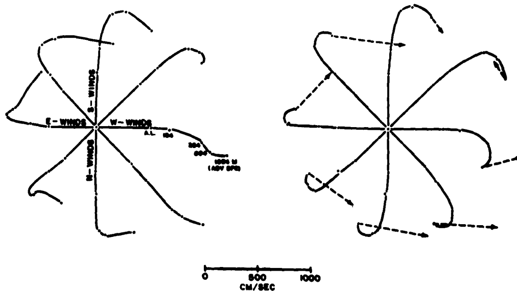
OBSERVED HODOGRAPHS (TOTAL OF 364 PROFILES)
