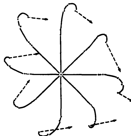
REDUCED HODOGRAPHS AND THERMAL WINDS
