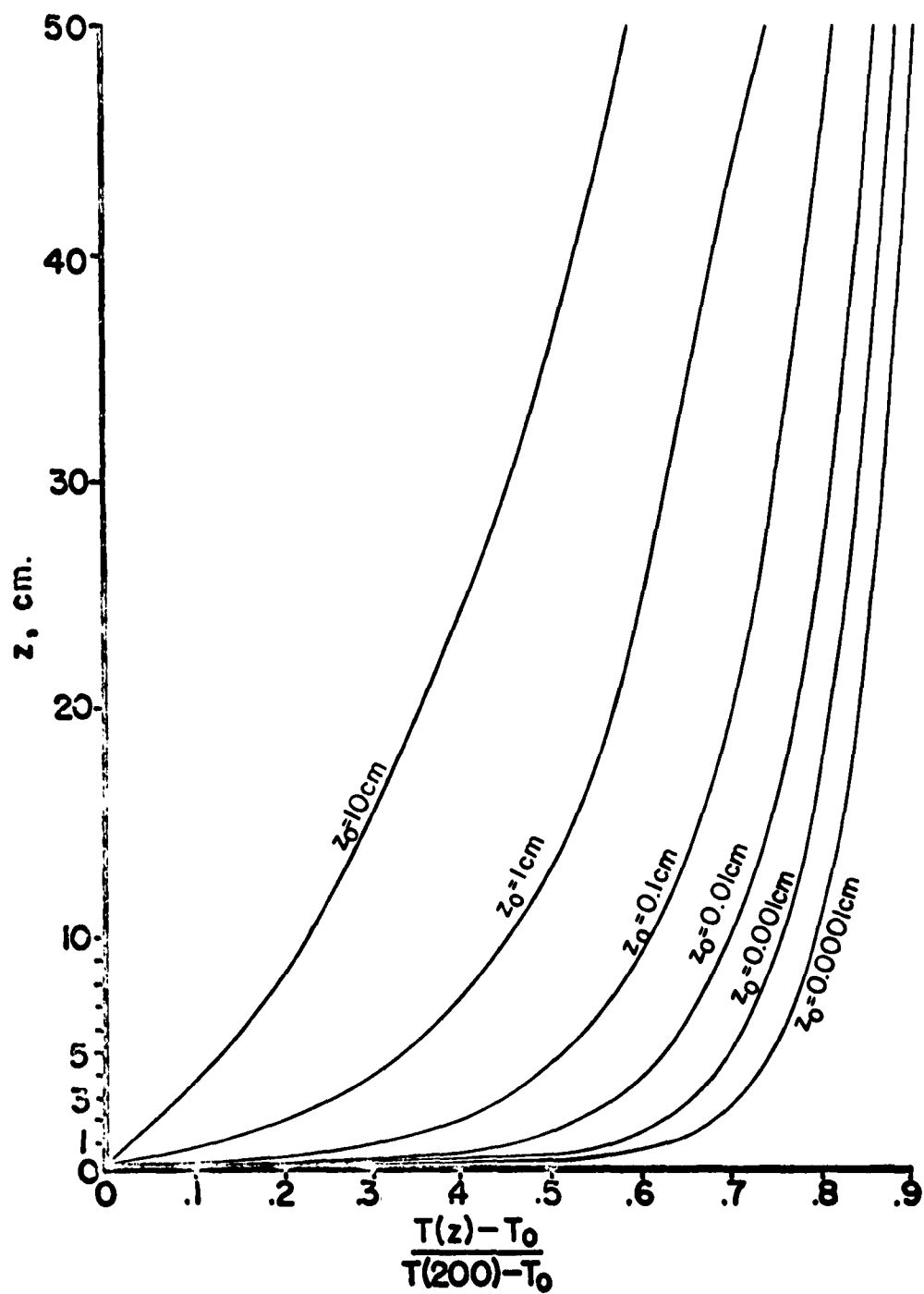
Fig. 3. Logarithmic profiles as a function of z_0 , plotted linearly versus height ( z ).
