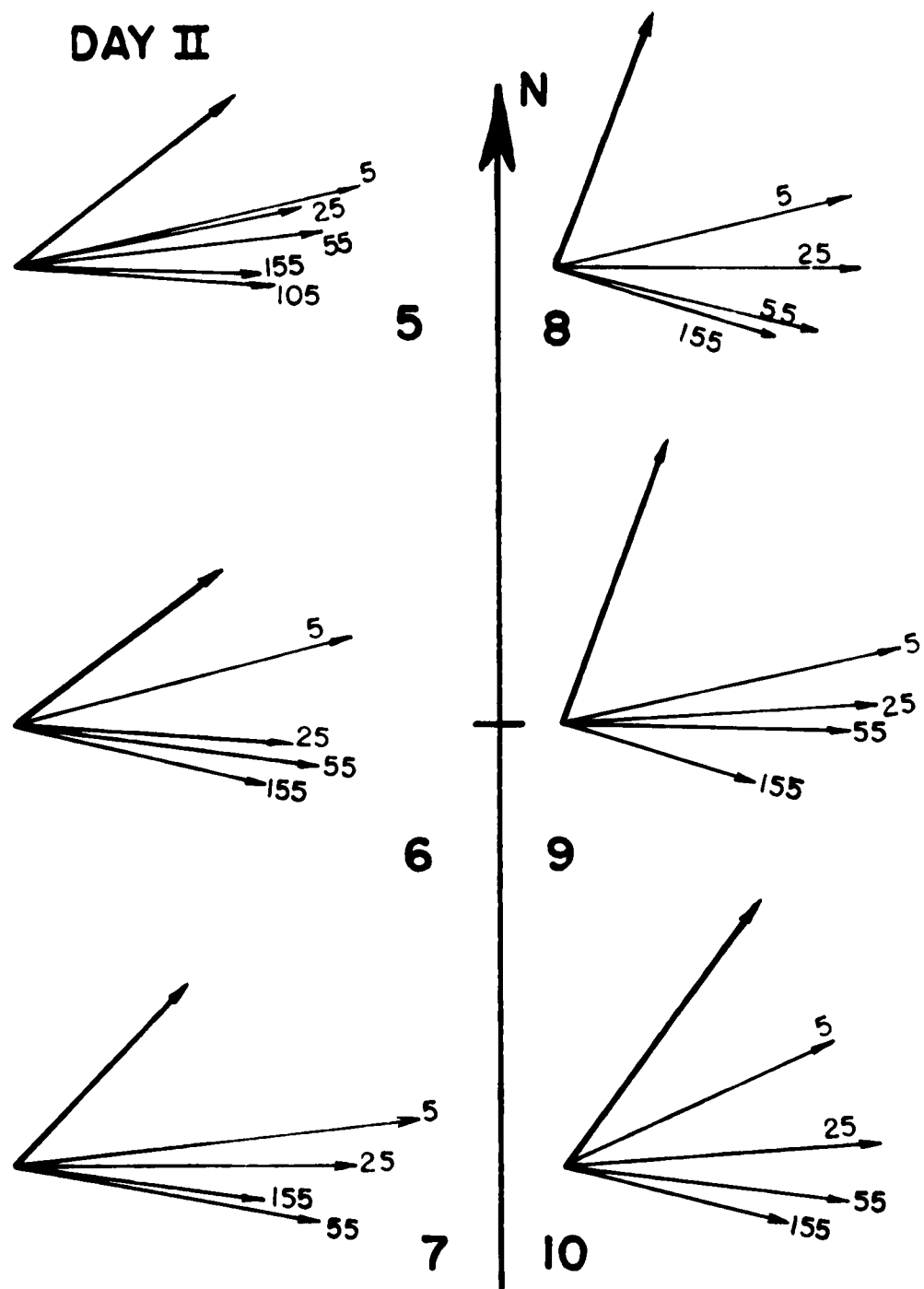
Fig. 4. Individual current hodographs in Lake Mendota on 18 August 1961, run 5 through 10.
