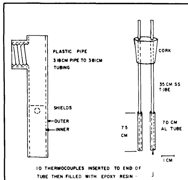
Fig. 17. Details of construction of temperature profile equipment.
