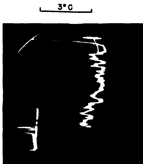
Fig. 4. A single downswEEP of the sensor, taken at 2:12 pm on September 9, 1961.
