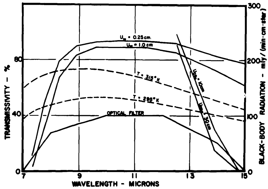
Fig. 3. Transmissivity and black-body radiation curves.
