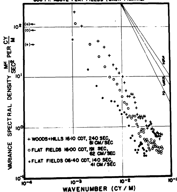
Fig. 4. The power spectra of turbulent vertical velocities measured with the airborne system.
