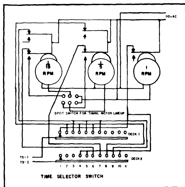
Fig. 33. Time switch and card selection.
