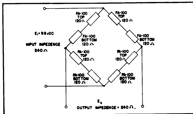
Fig. 22. Strain-gauge bridge circuit.
