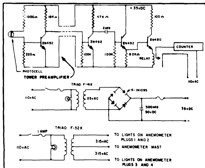
Fig. 9. Anemometer counting circuit and power supply.
