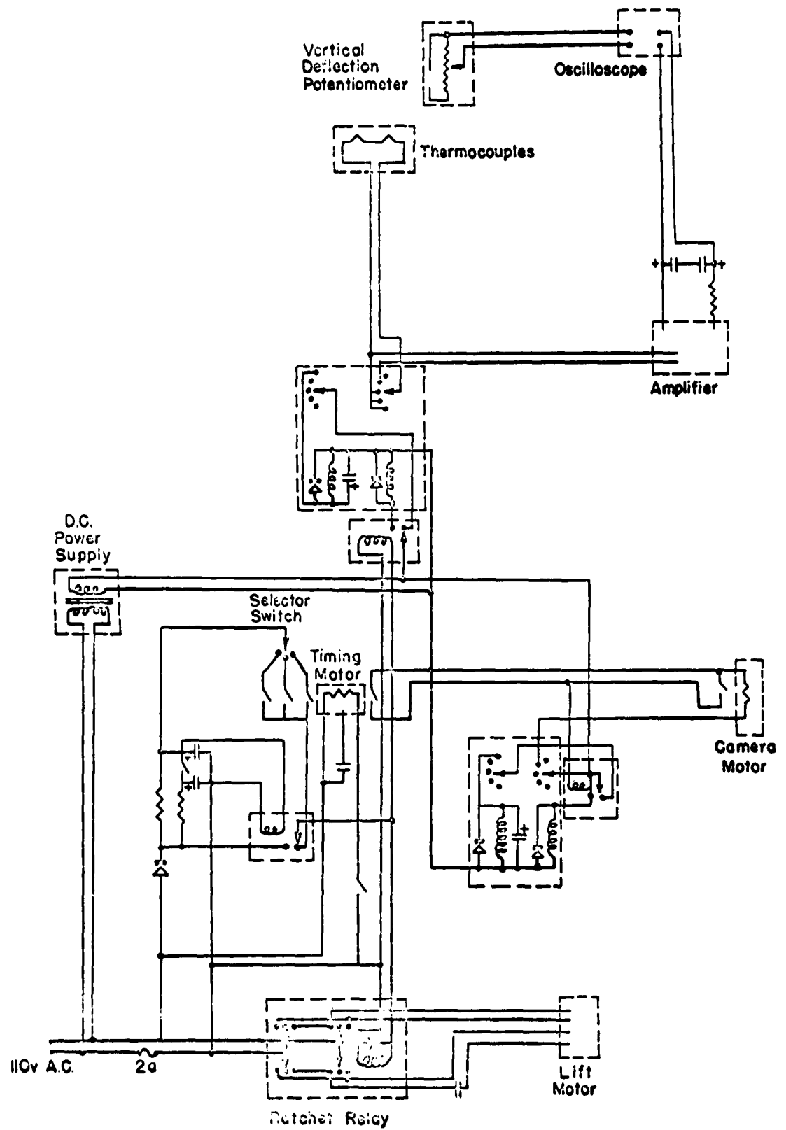
Fig. 1. Electrical circuitry.
