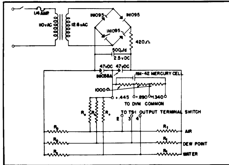
Fig. 12. Thermistor power supply.
