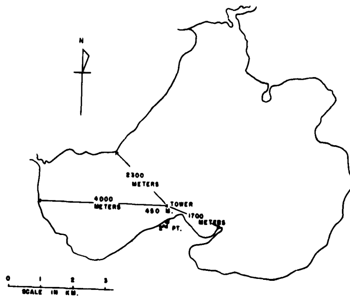
Fig. 1. Map of Lake Mendota with location of tower and instrument building.
