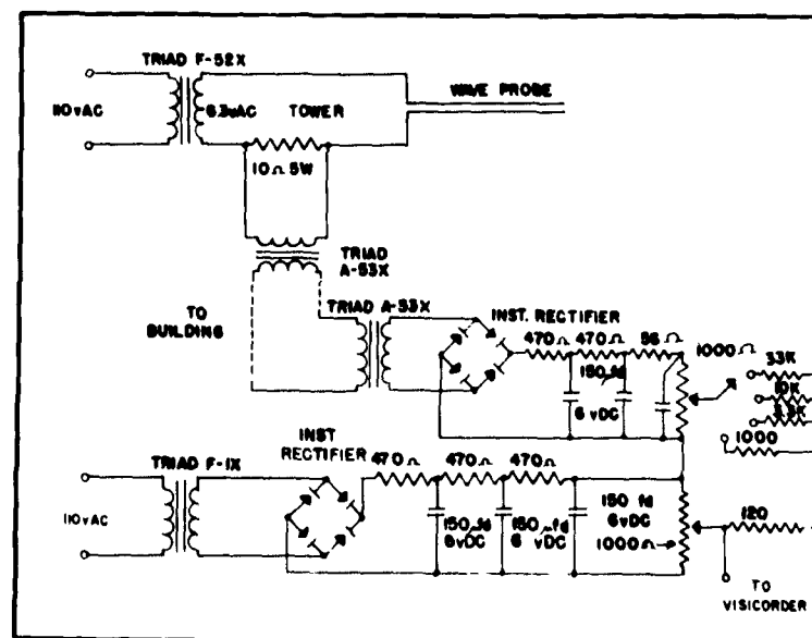
Fig. 19. Wave detector circuits.
