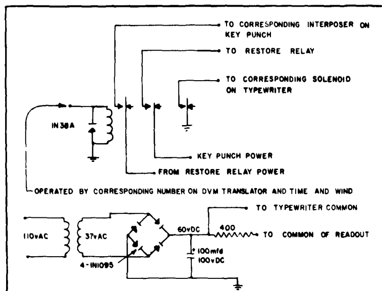
Fig. 32. Operation of key punch and typewriter.
