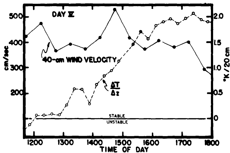
Fig. 9. 30-min averages of windspeed at 40 cm, 15-min averages of temperature difference between air at 20 cm and water; 6 September 1961, for the hours of run 21 to 26.
