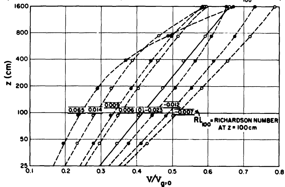
GEOSTROPHIC WIND RATIO V/V_{g,0} VS. LOGARITHM OF HEIGHT (z); O'NEILL, 1953 (CLASS-MEANS OF WINDPROFILES, RESULTING IN INDICATED MEAN Ri_{100} VALUES)
