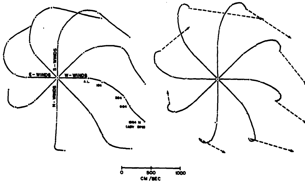
REDUCED HODOGRAPHS AND THERMAL WINDS
