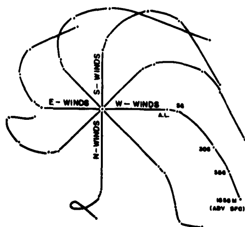
OBSERVED HODOGRAPHS (TOTAL OF 182 PROFILES)
