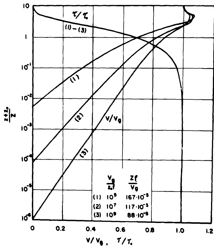
Fig. 2. Theoretical profiles, of wind ratio V/V_{g0} and stress ratio \tau/\tau_0 versus logarithm of relative height, through the entire atmospheric boundary layer in adiabatic states. The numbers at the curves refer to three indicated surface-Rossby numbers and subsequent coefficients for conversion from relative to metric height.
