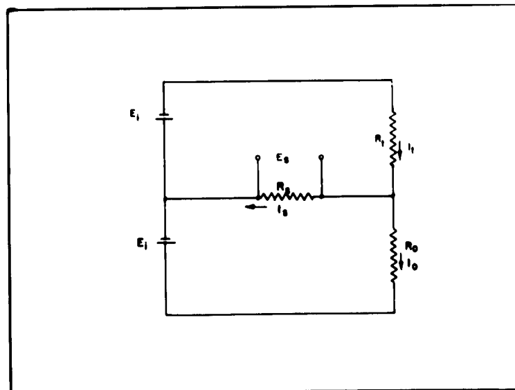
Fig. 13. Basic thermistor circuit.
