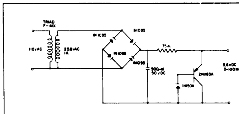
Fig. 23. Power supply for strain-gauge bridge.
