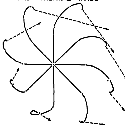
REDUCED HODOGRAPHS AND THERMAL WINDS
