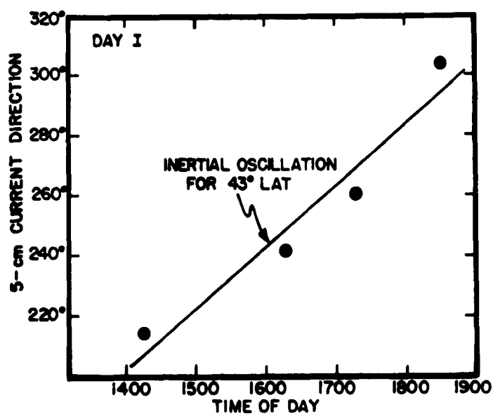
Fig. 3. Direction of 5 cm current (full dots) in Lake Mendota at indicated hour for the four runs on 17 August 1961. Note the systematic veering which is compared with the theoretical rate of rotation for an inertia oscillation at this geographical latitude.
