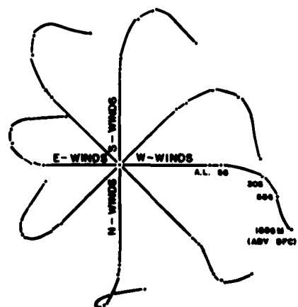
OBSERVED HODOGRAPHS (TOTAL OF 206 PROFILES)
