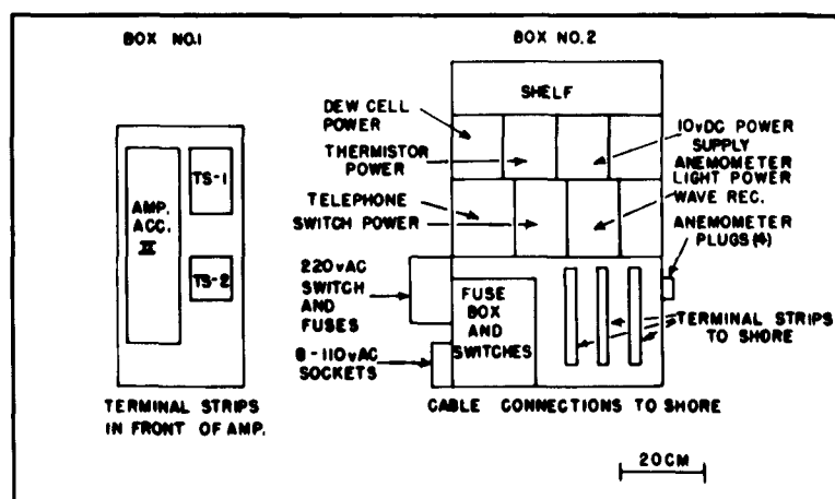
Fig. 5. Arrangement of electrical boxes on lake tower.
