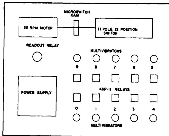
Fig. 28. Layout of DVM translator.
