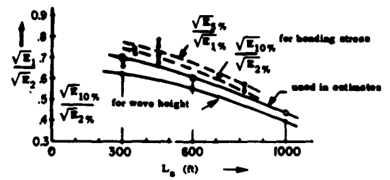
Figure 21 – Slopes of Probability Distribution Curves of Bending Stress and Wave Heights (From Figures 7 and 17)
